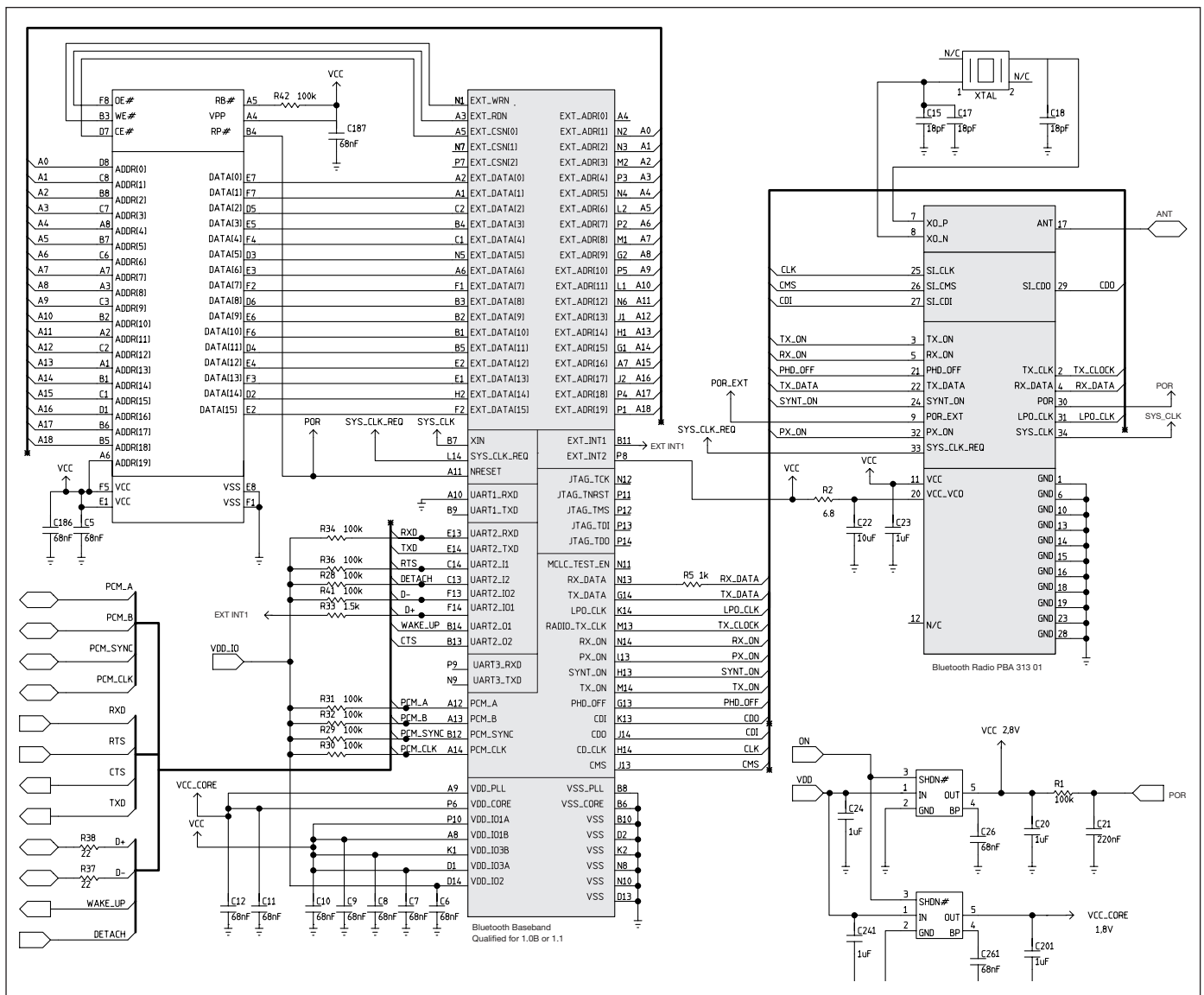
Figure 13. Example of interface between Ericsson Bluetooth Baseband and Bluetooth Radio.
