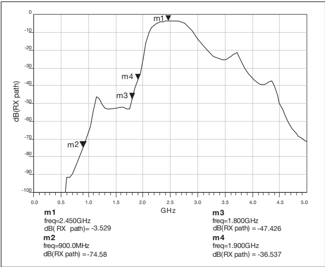
Figure 2. Typical out-of-band blocking characteristics excluding antenna isolation and on chip filtering.
