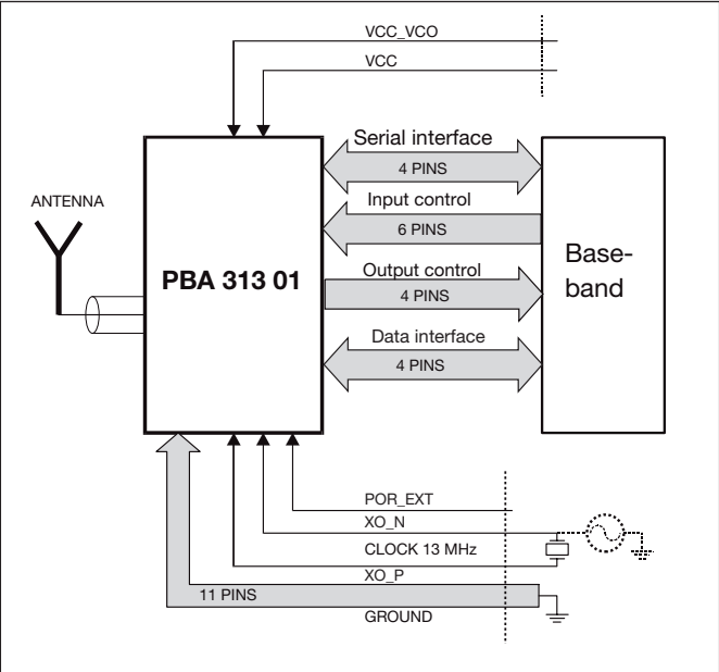
Figure 5. System overview.
