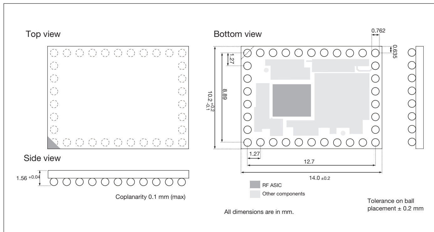
Figure 4. Mechanical dimensions of PBA 313 01.
