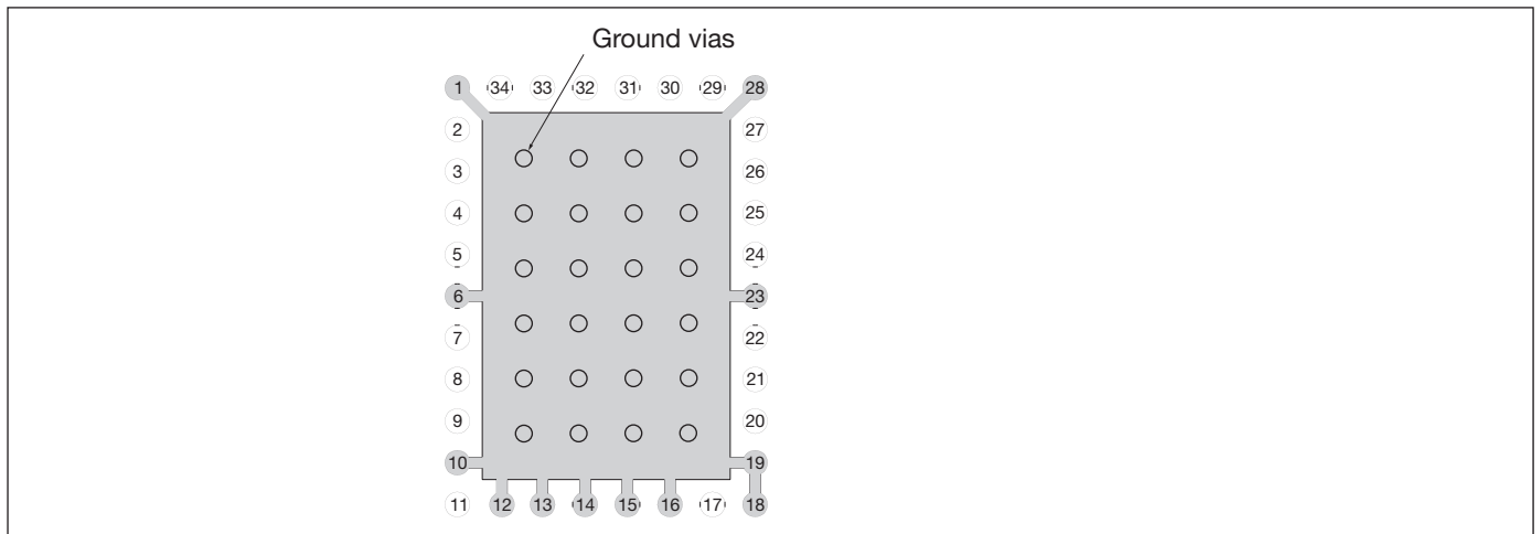
Figure 12. Example of local ground plane underneath the Bluetooth Radio.
