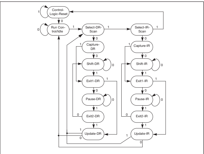
Figure 9. State machine for serial interface control. '0' denotes a logic level 'low' and '1' level 'high' level on the SI_CMS control pin.
