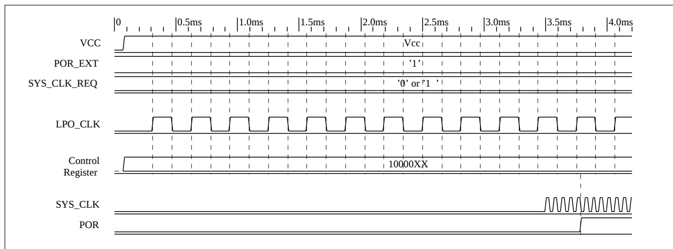
Figure 7. Powering up the module.
