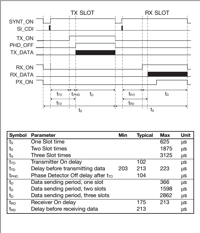
Figure 6 and table 2. Timing sequence for data transmission.
