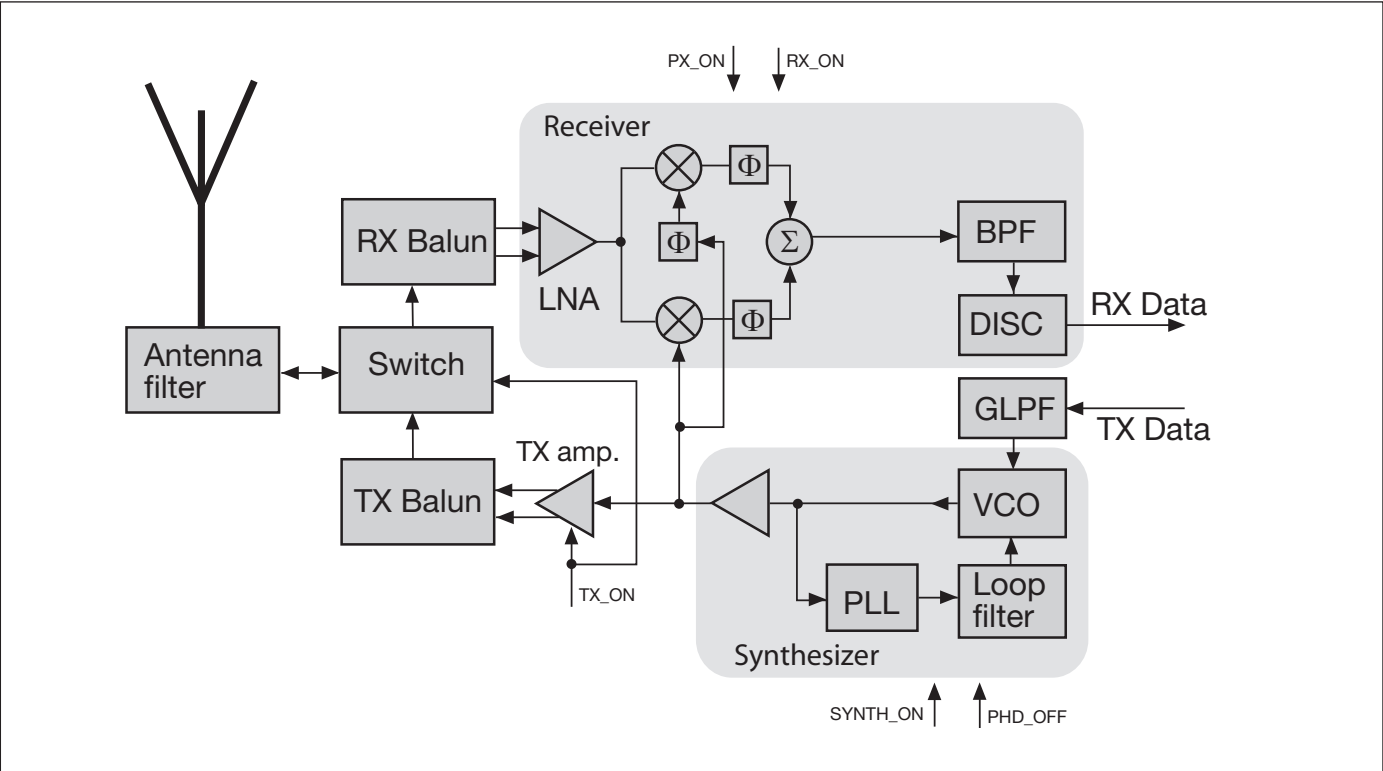
Figure 1. Block diagram.
