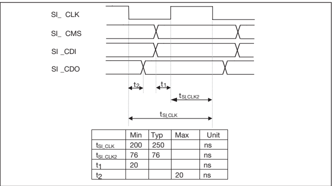
Figure 8. Timing diagram of the serial interface.
