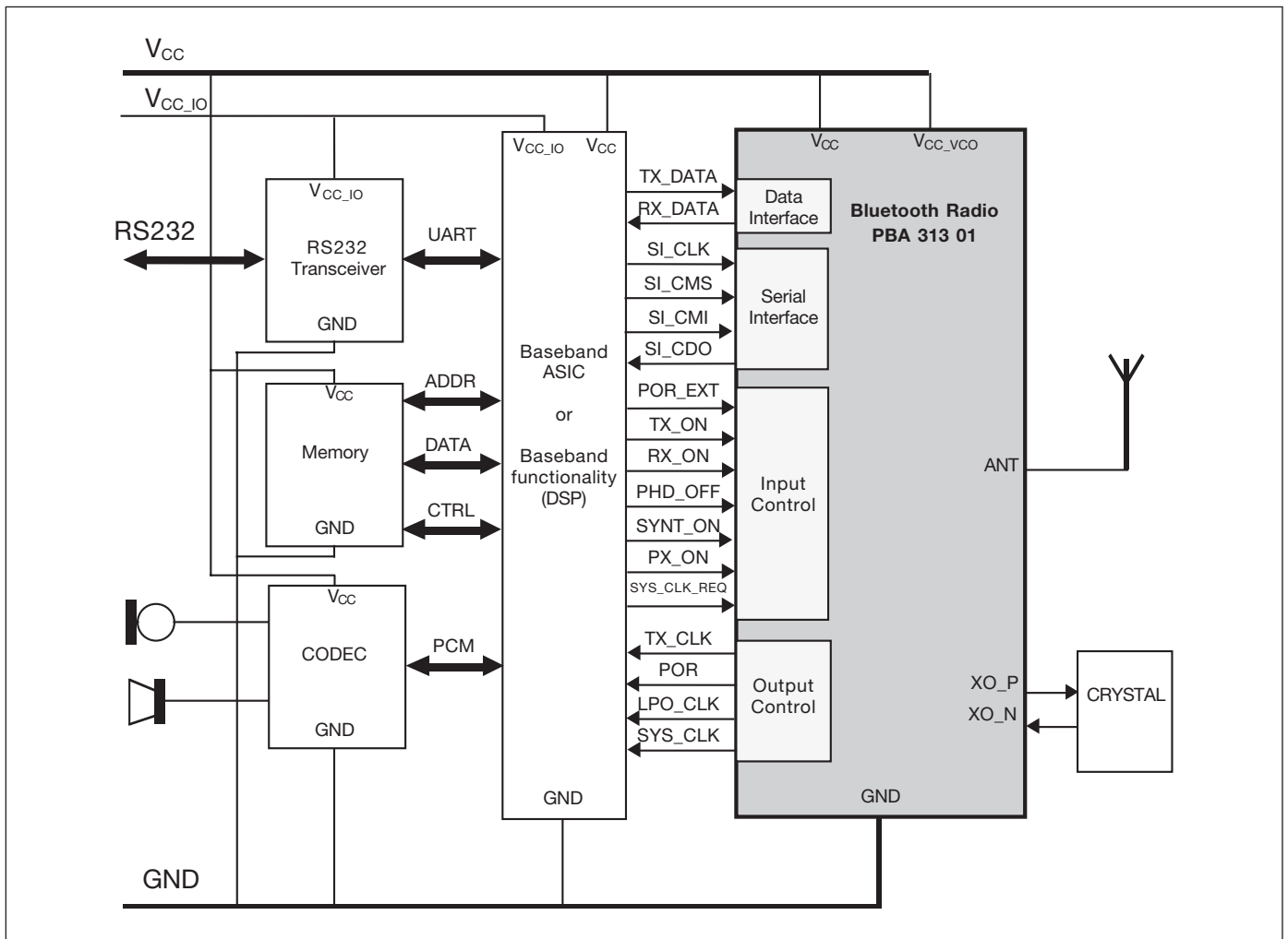
Figure 11. Typical UART or PCM configuration.
