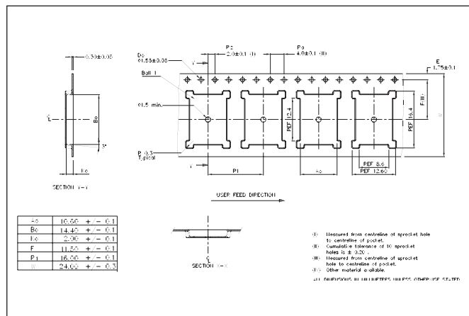
Figure 15. Carrier tape dimensions.
