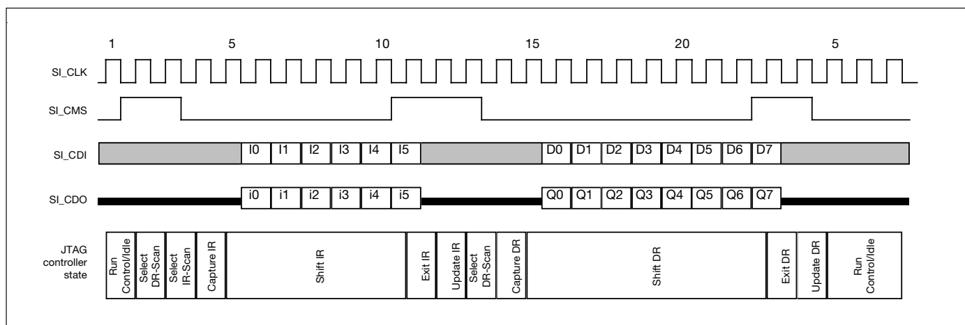
Figure 10. Reading and updating a data register. A data register is selected by entering the Shift IR state using SI_CMS, and transferring the appropriate bit code to the instruction register using SI_CDI (I[5:0]=01YYYY, where YYYY is the address of the register). Moving to the Shift-DR state, eight bits of register data can then be transferred on SI_CDI and SI_CDO. The data register selected by the instruction register is updated when the SI controller enters the Update-DR state. At the end of the data register access, the SI controller is once again held in the Run Control/Idle state.
