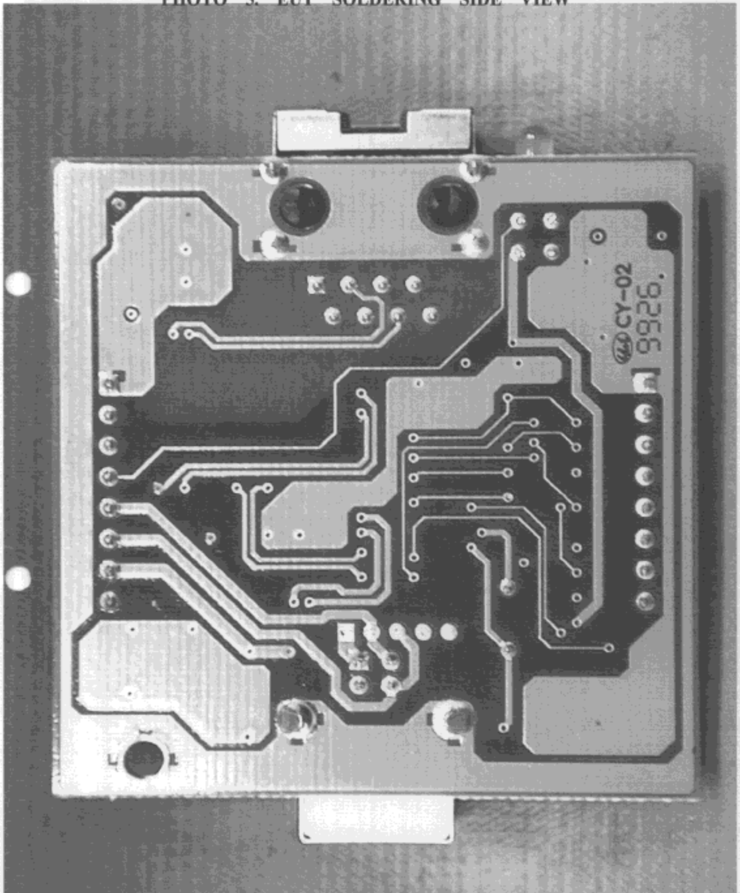
PHOTO 5. EUT SOLDERING SIDE VIEW
