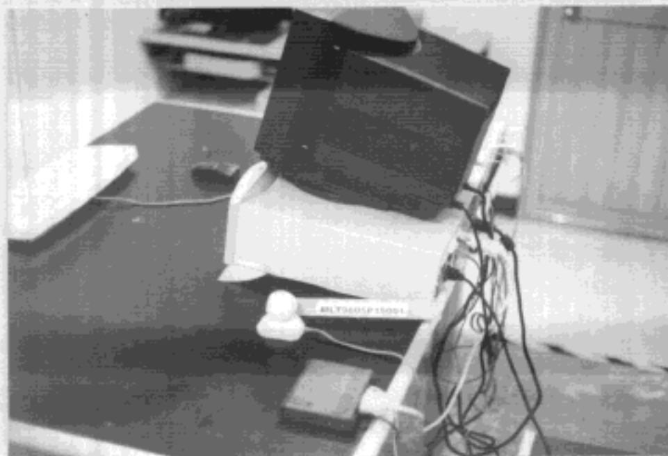
Rear View of The Test Configuration
