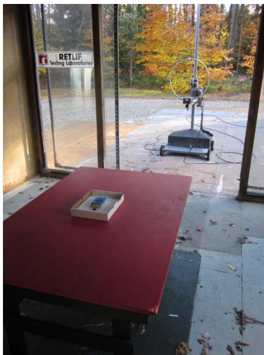
Test Setup, Fundamental and Spurious Emissions, 450 kHz to 30 MHz
