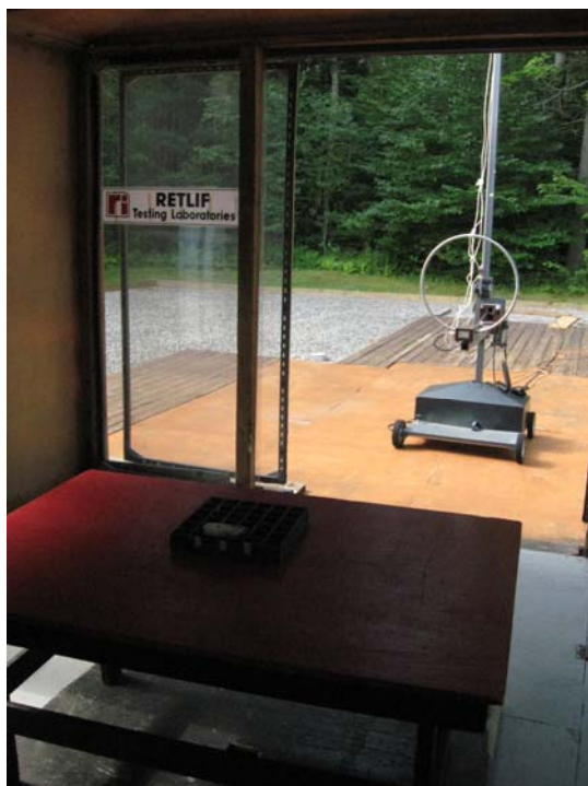
Test Setup, Planar
