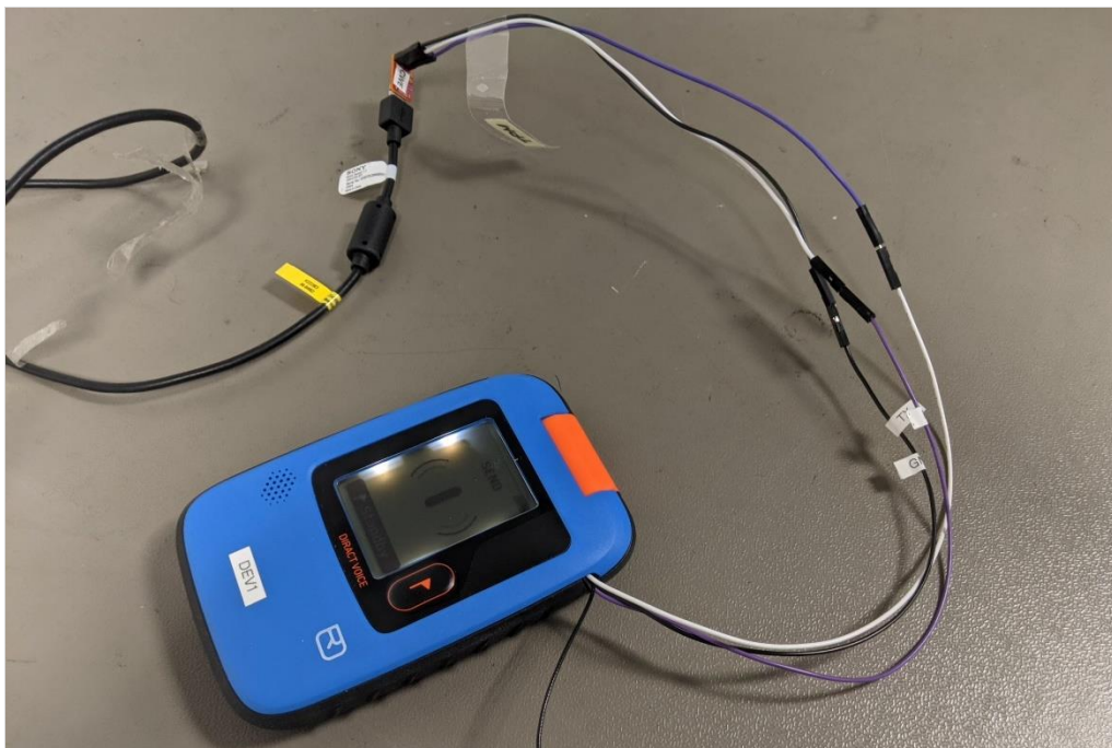
Photograph 8: Conducted Test Set up in the Radio Lab, close view
