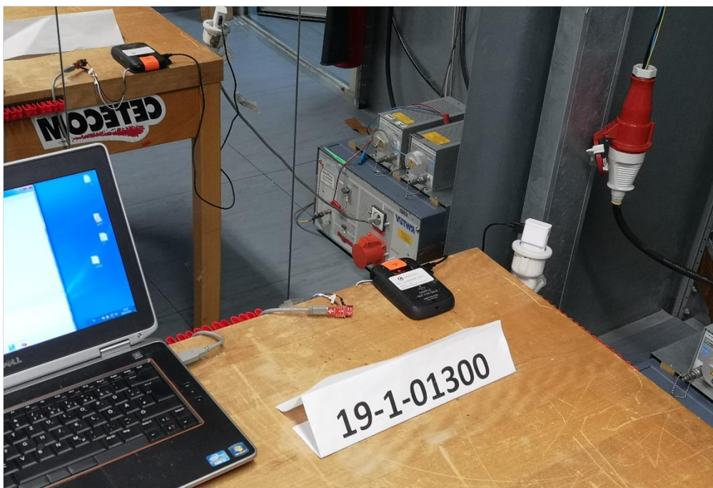
Photograph 10: EUT Setup Conducted emissions on AC-Power lines
