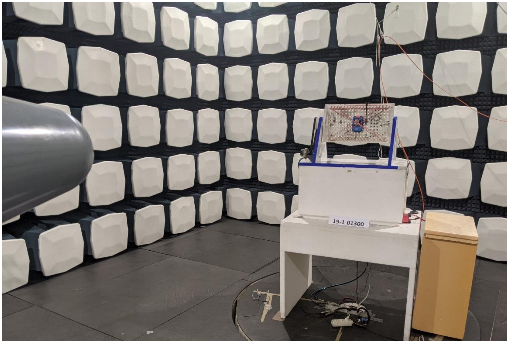
Photograph 5: EUT Test Setup in the fully anechoic chamber, Radiated interference field
