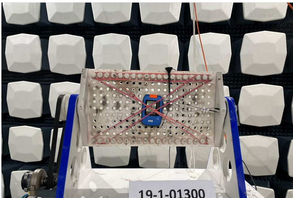
Photograph 6: EUT Test Setup in the fully anechoic chamber, Radiated interference field
