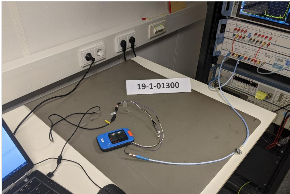
Photograph 7: Conducted Test Set up in the Radio Lab, overall view
