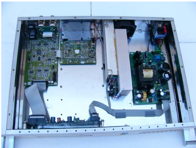
Top without main cover and PS cover
