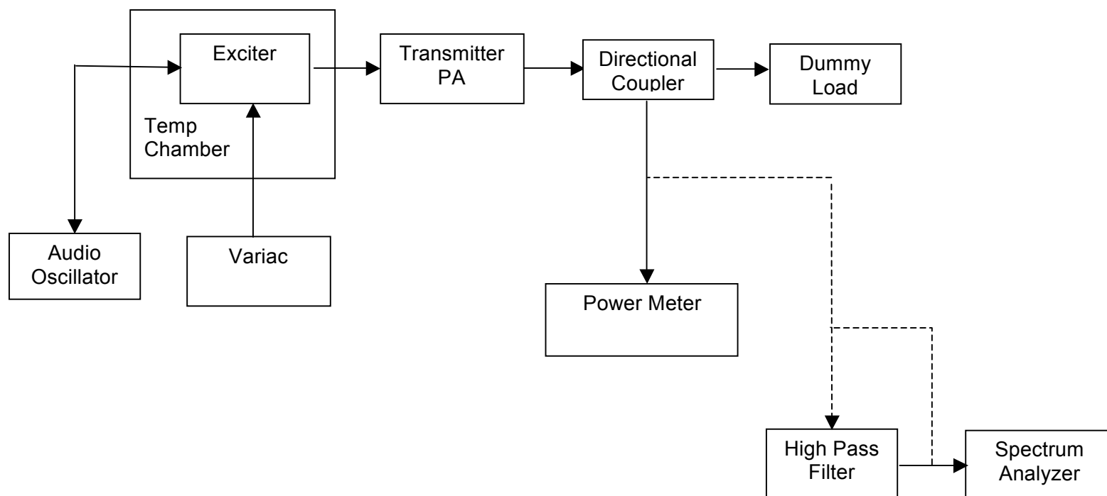
FIGURE 1—TEST EQUIPMENT CONFIGURATION
