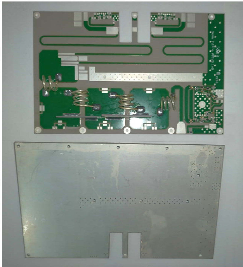
RF Combiner and Low Pass Filter Board
