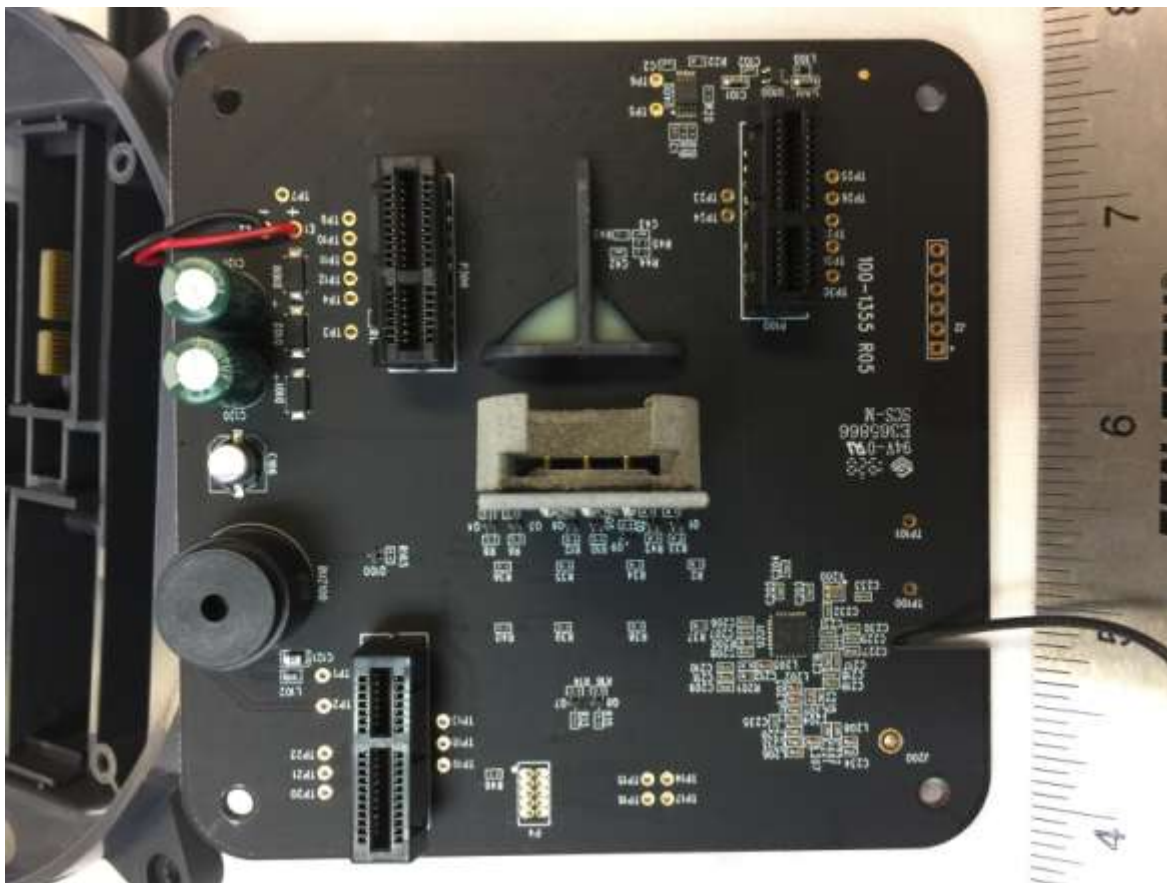
Figure 6. Main Board PCB Socket and Solder Side
