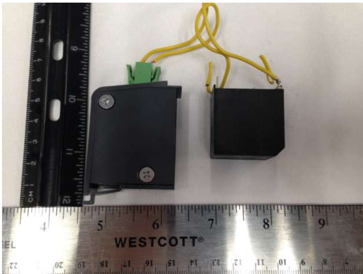
Figure 5. Long Wire Module (Separate Modular Certification Pending) Removed from Main Enclosure
