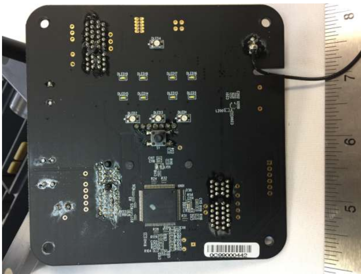
Figure 7. Main Board PCB, LED and IC Circuit Side
