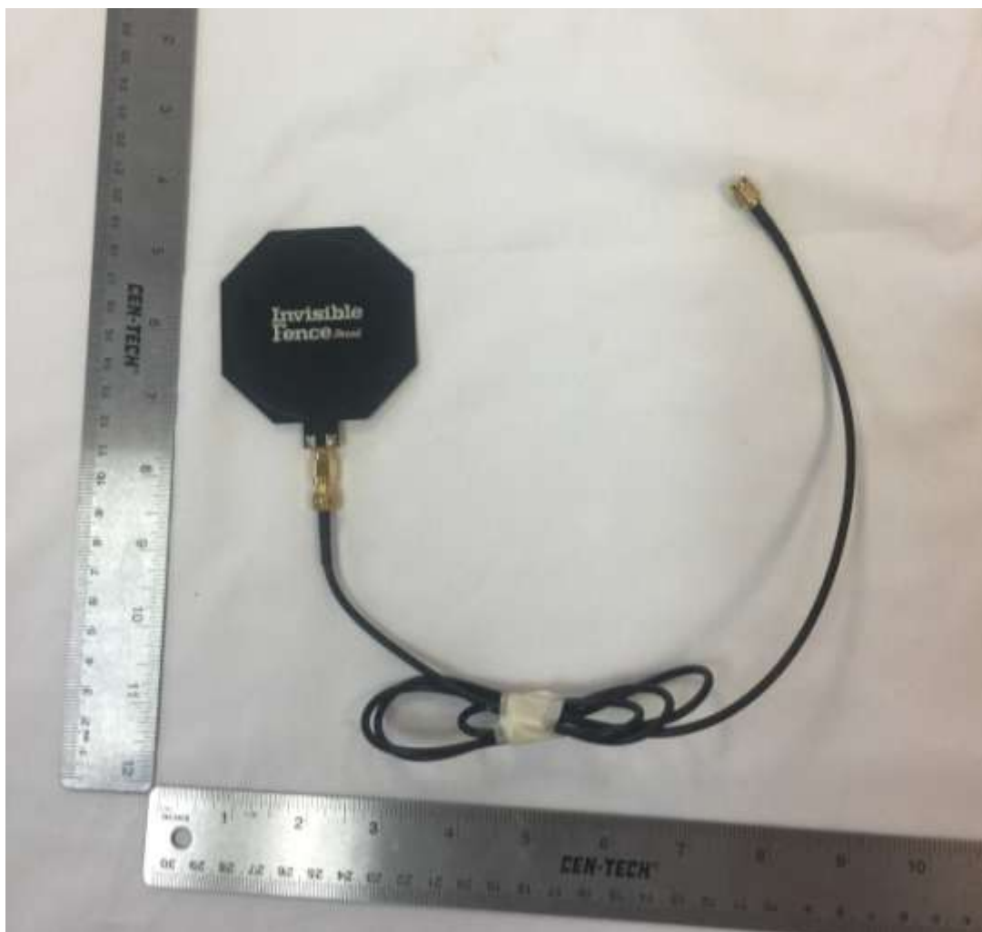
Figure 7. External MURS Antenna
