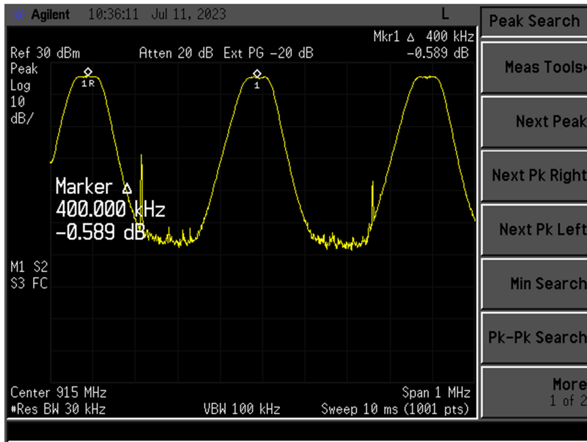
Figure 22. Channel Separation
