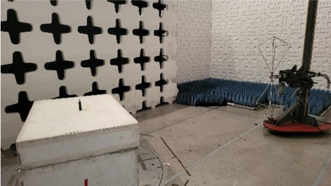
Figure 3. Radiated Emissions Test Setup, 30 MHz to 200 MHz, 0.5-mile (STD00-17811)
