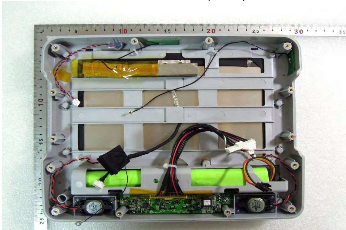
WLAN Antenna (Main)
