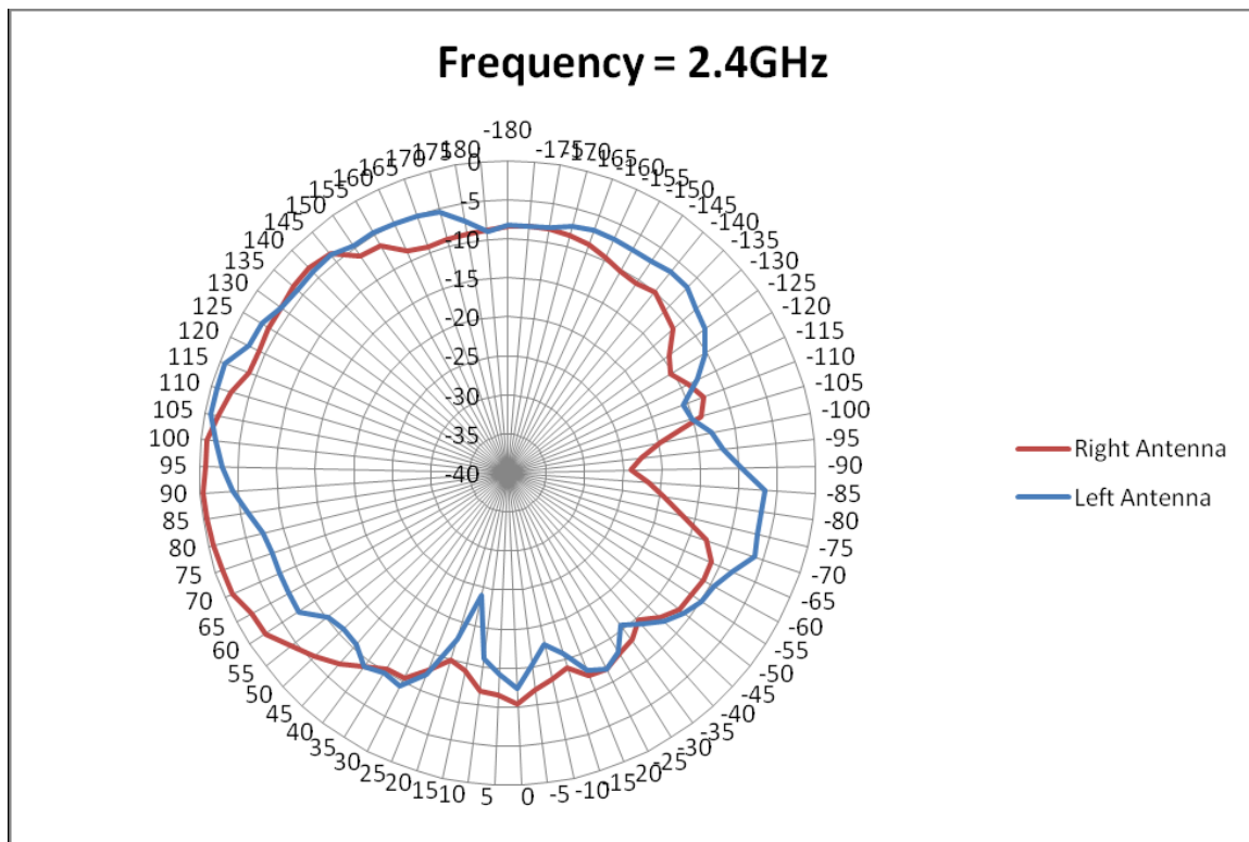
Figure 21 Radiation Plots for 2.400GHz (E2-Plane) Left/Right Antenna
