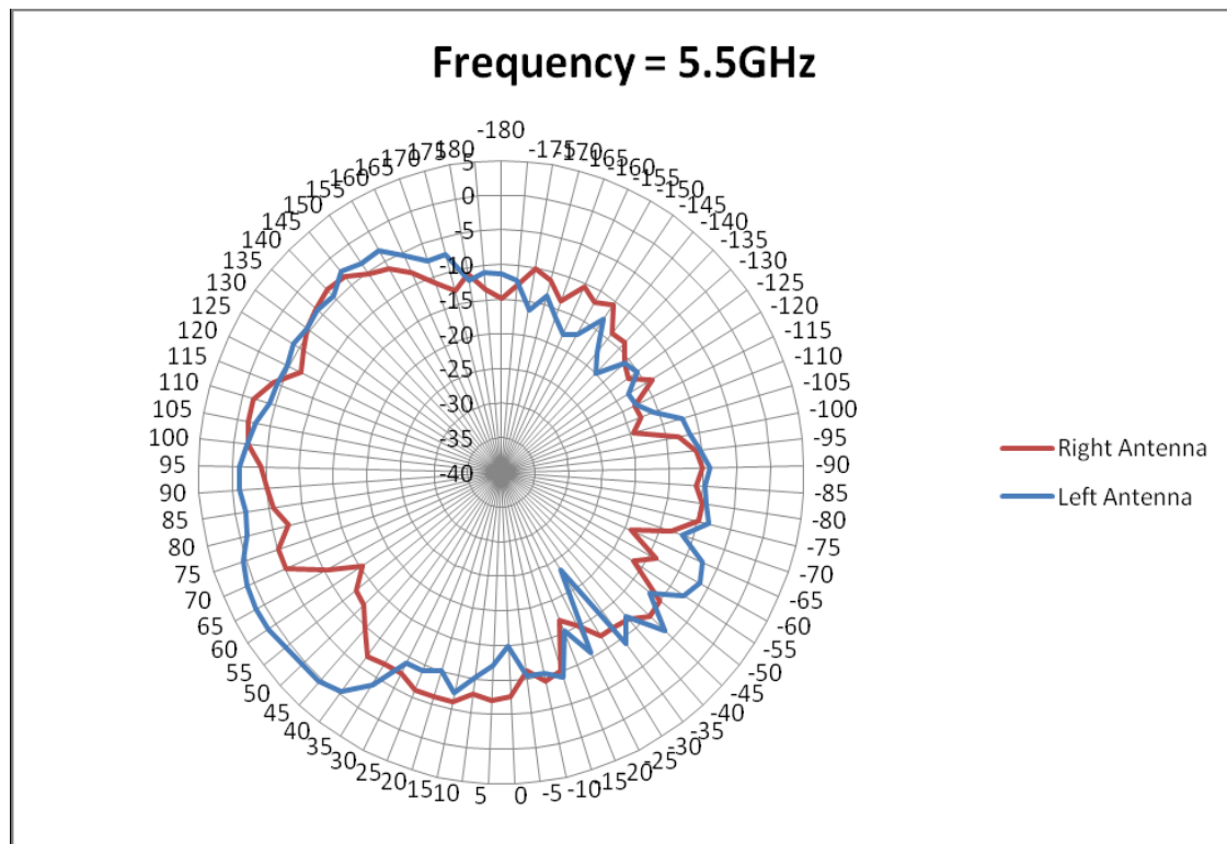
Figure 38 Radiation Plots for 5.500GHz (E2-Plane) Left/Right Antenna
