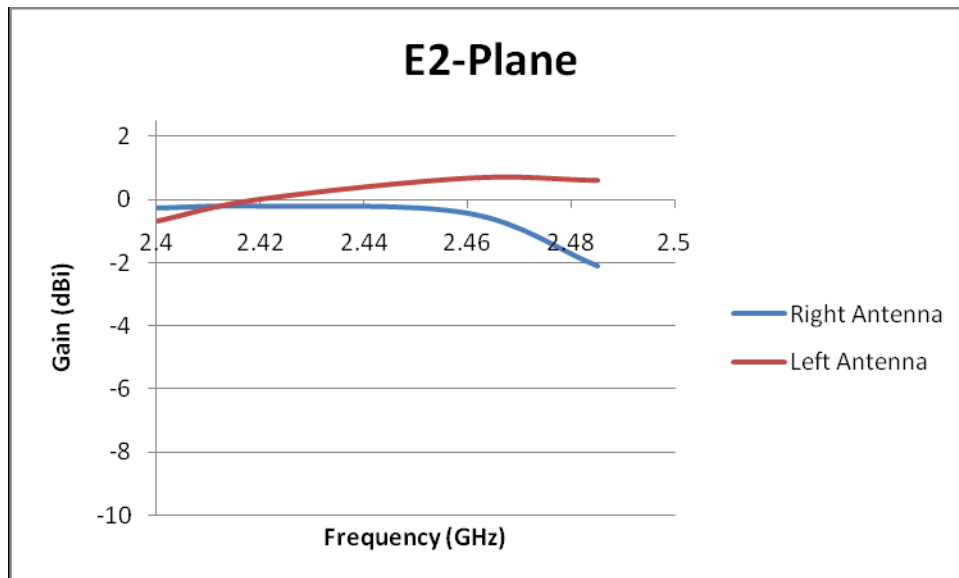
Figure 27 Peak Gain for Bluetooth Printed Antenna (E2-Plane) Left/Right Antenna
