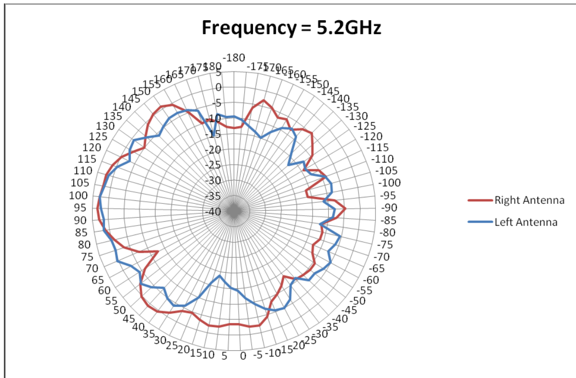
Figure 29 Radiation Plots for 5.200GHz (H-Plane) Left/Right Antenna
