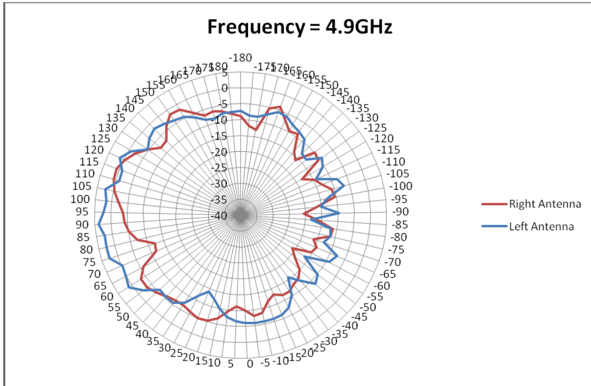
Figure 28 Radiation Plots for 4.900GHz (H-Plane) Left/Right Antenna
