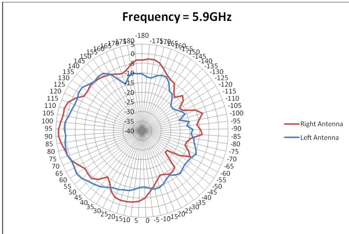
Figure 31 Radiation Plots for 5.900GHz (H-Plane) Left/Right Antenna
