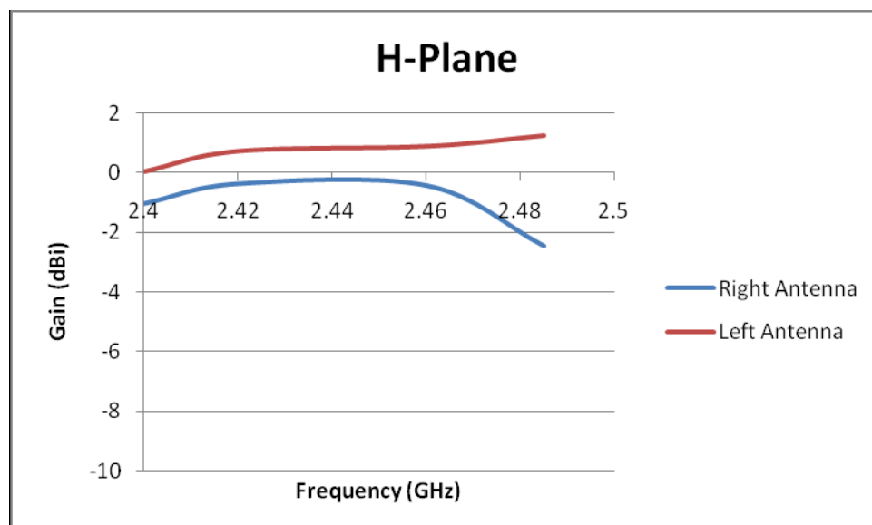
Figure 25 Peak Gain for Bluetooth Printed Antenna (H-Plane) Left/Right Antenna
