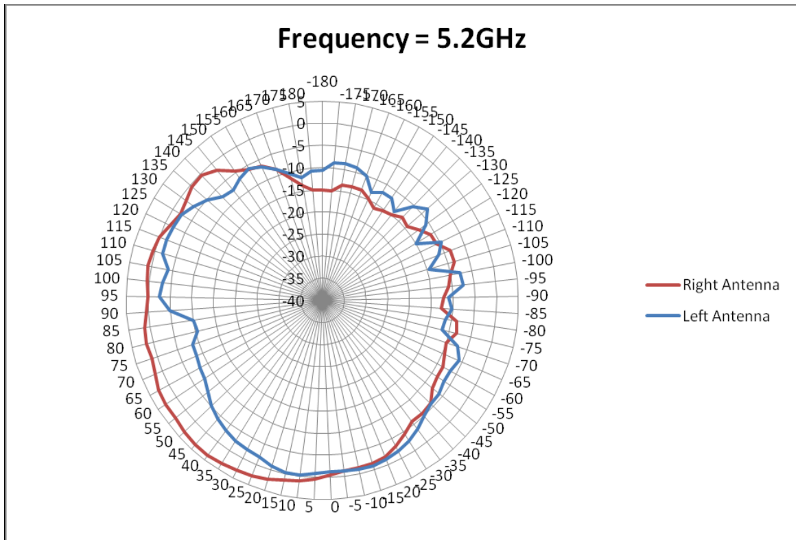
Figure 33 Radiation Plots for 5.200GHz (E1-Plane) Left/Right Antenna
