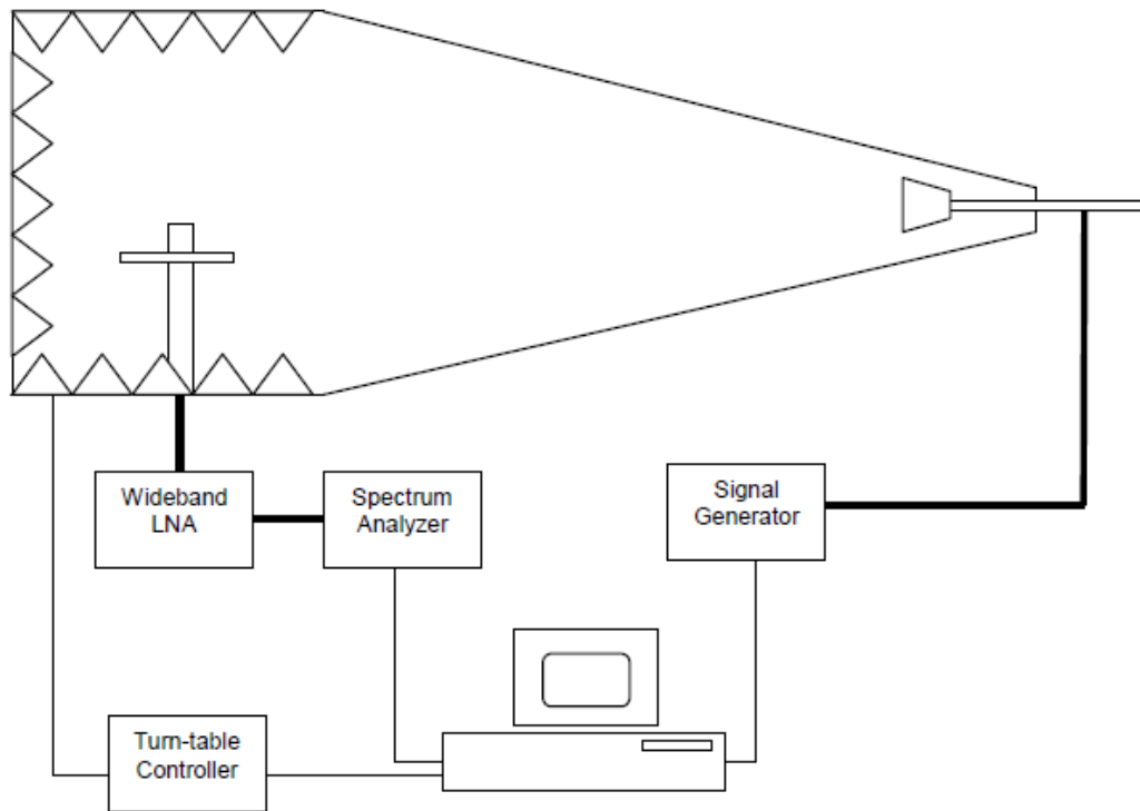
Figure 11 Anechoic Chamber Setup
