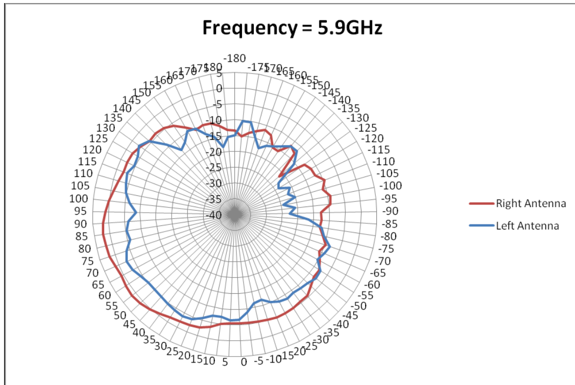
Figure 35 Radiation Plots for 5.900GHz (E1-Plane) Left/Right Antenna
