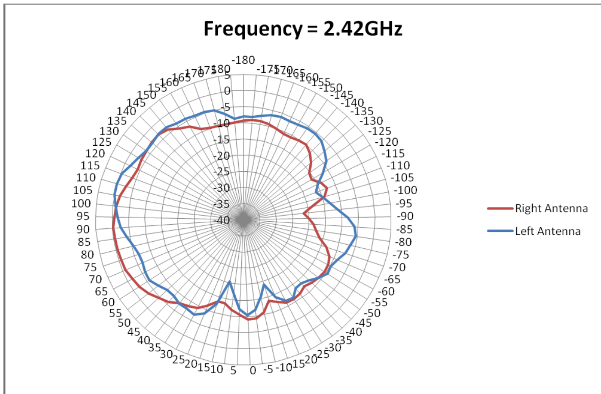
Figure 22 Radiation Plots for 2.420GHz (E2-Plane) Left/Right Antenna
