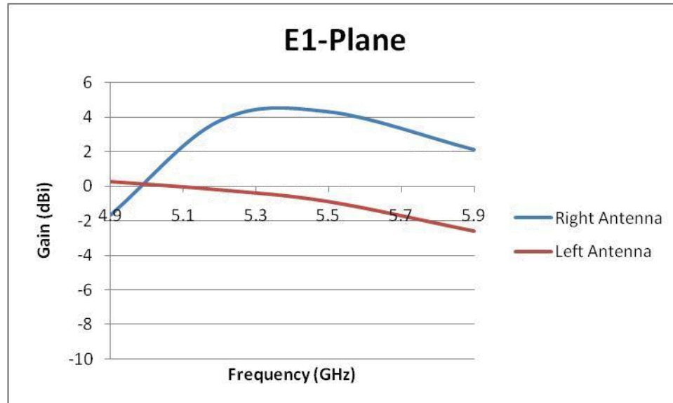
Figure 41 Peak Gain for External Antenna (E1-Plane) Left/Right
