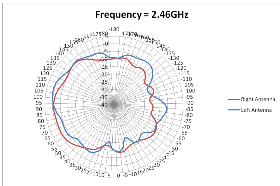
Figure 23 Radiation Plots for 2.460GHz (E2-Plane) Left/Right Antenna
