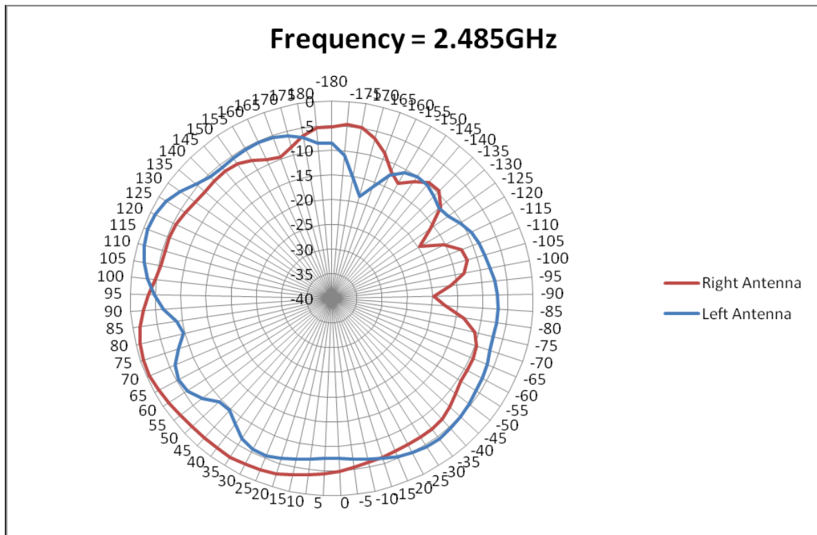
Figure 20 Radiation Plots for 2.485GHz (E1-Plane) Left/Right Antenna
