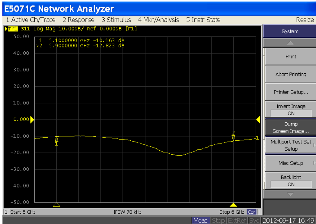
Figure 7 Right Antenna 5GHz Return Loss
