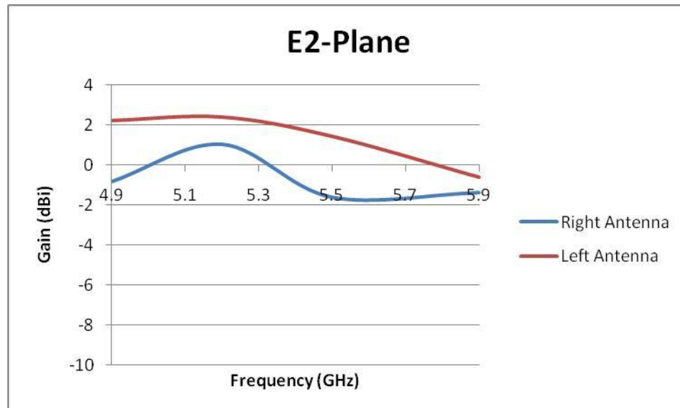
Figure 42 Peak Gain for External Antenna (E2-Plane) Left/Right
