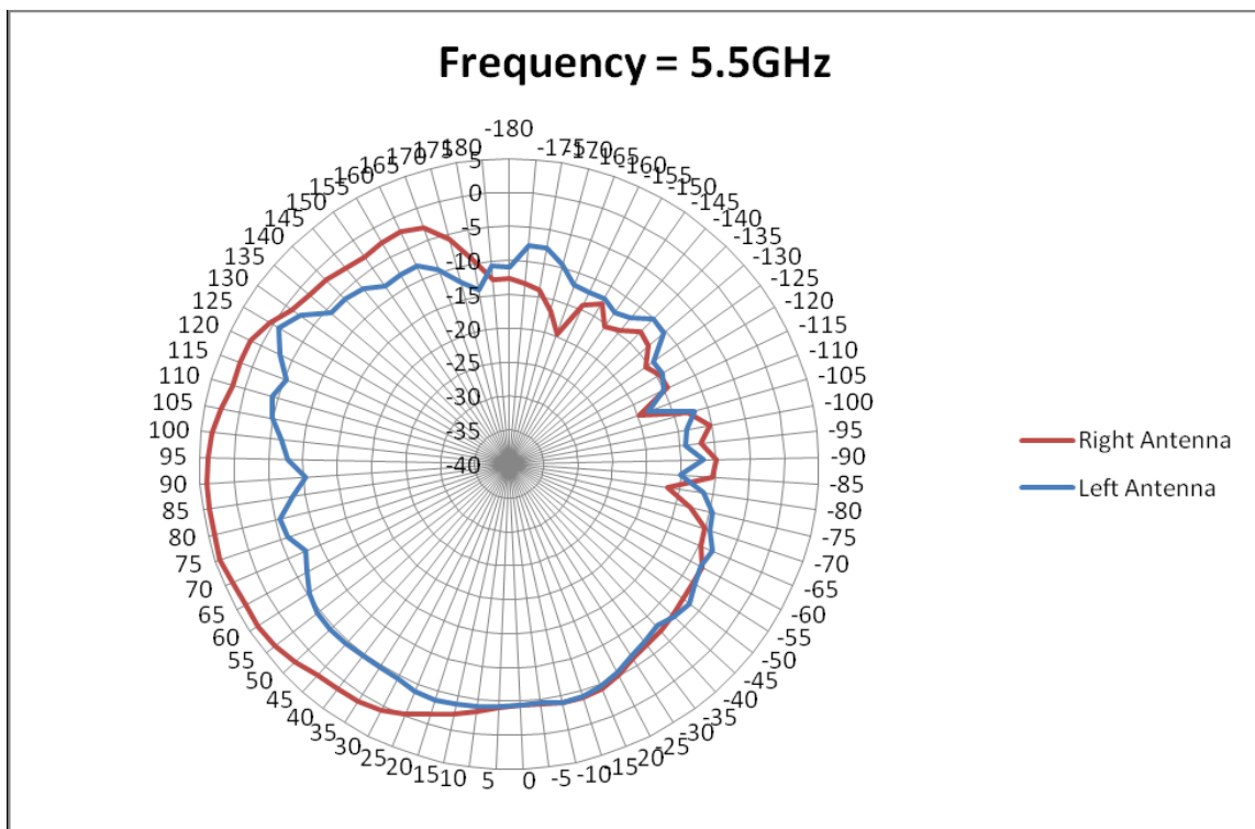
Figure 34 Radiation Plots for 5.500GHz (E1-Plane) Left/Right Antenna
