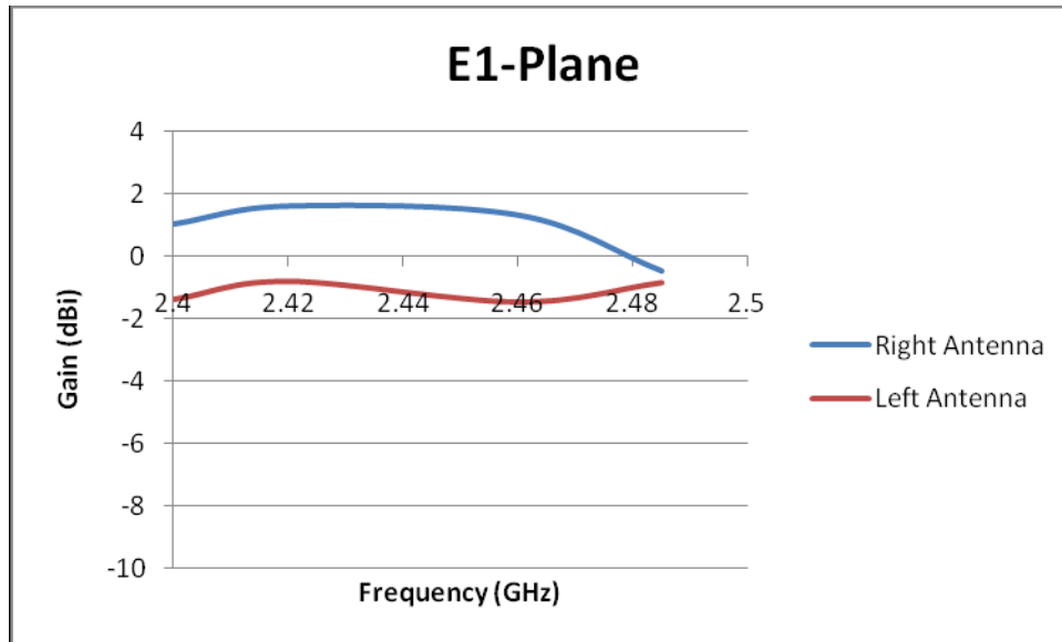
Figure 26 Peak Gain for Bluetooth Printed Antenna (E1-Plane) Left/Right Antenna
