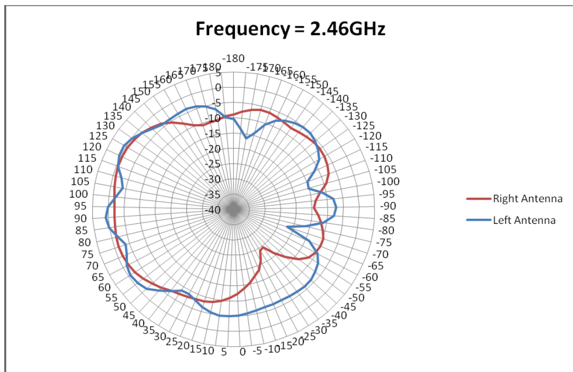
Figure 15 Radiation Plots for 2.460GHz (H-Plane) Left/Right Antenna
