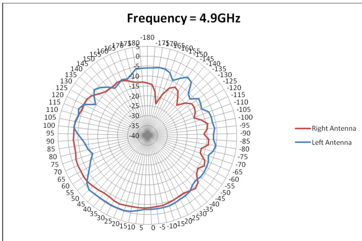
Figure 32 Radiation Plots for 4.900GHz (E1-Plane) Left/Right Antenna
