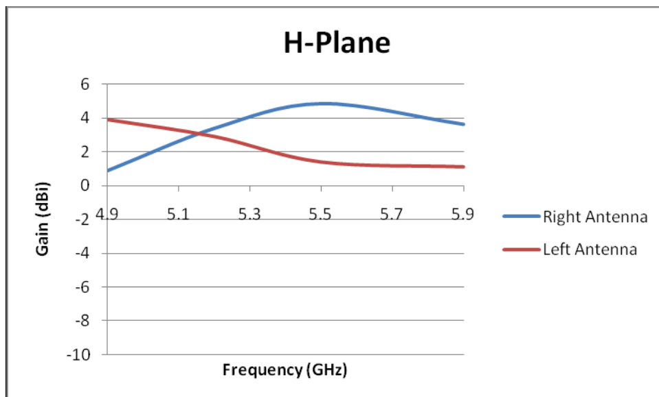
Figure 40 Peak Gain for External Antenna (H-Plane) Left/Right
