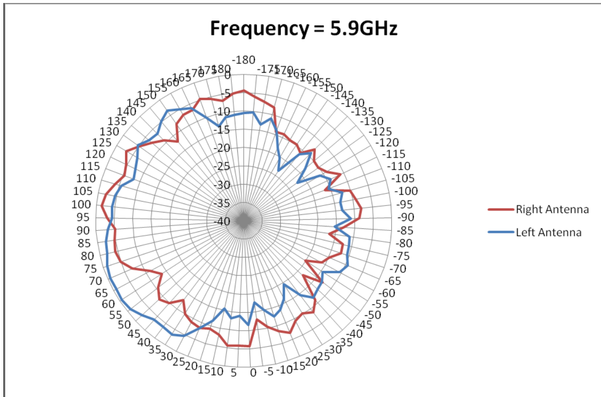
Figure 39 Radiation Plots for 5.900GHz (E2-Plane) Left/Right Antenna
