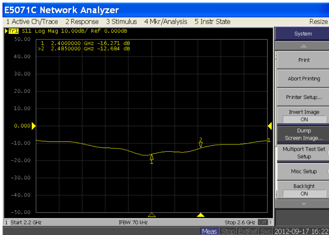
Figure 5 Right Antenna 2.4GHz Return Loss
