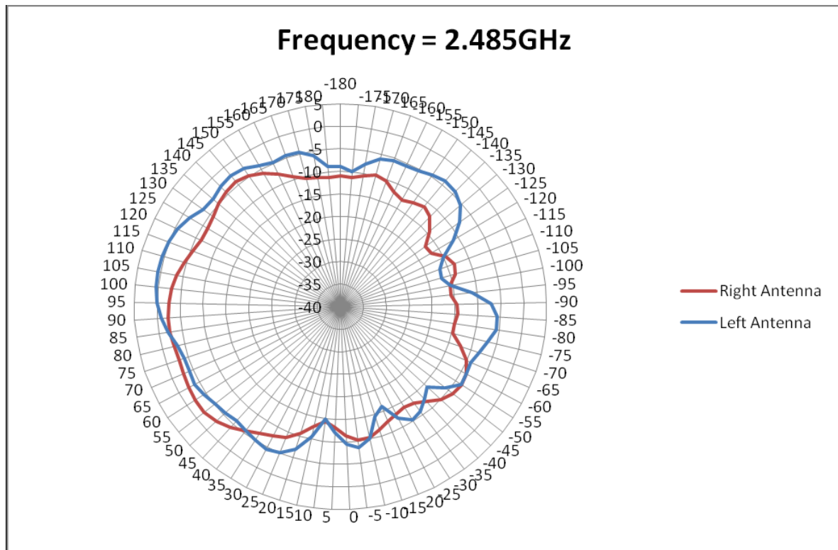
Figure 24 Radiation Plots for 2.485GHz (E2-Plane) Left/Right Antenna
