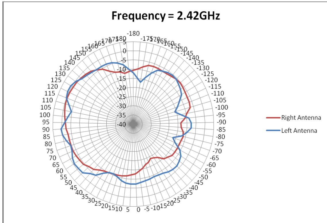
Figure 14 Radiation Plots for 2.420GHz (H-Plane) Left/Right Antenna
