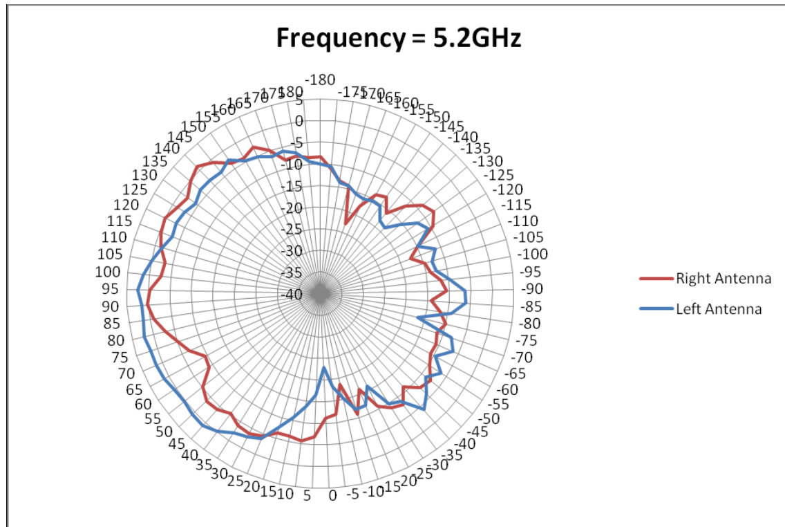
Figure 37 Radiation Plots for 5.200GHz (E2-Plane) Left/Right Antenna
