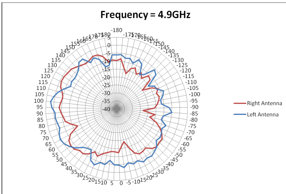
Figure 36 Radiation Plots for 4.900GHz (E2-Plane) Left/Right Antenna
