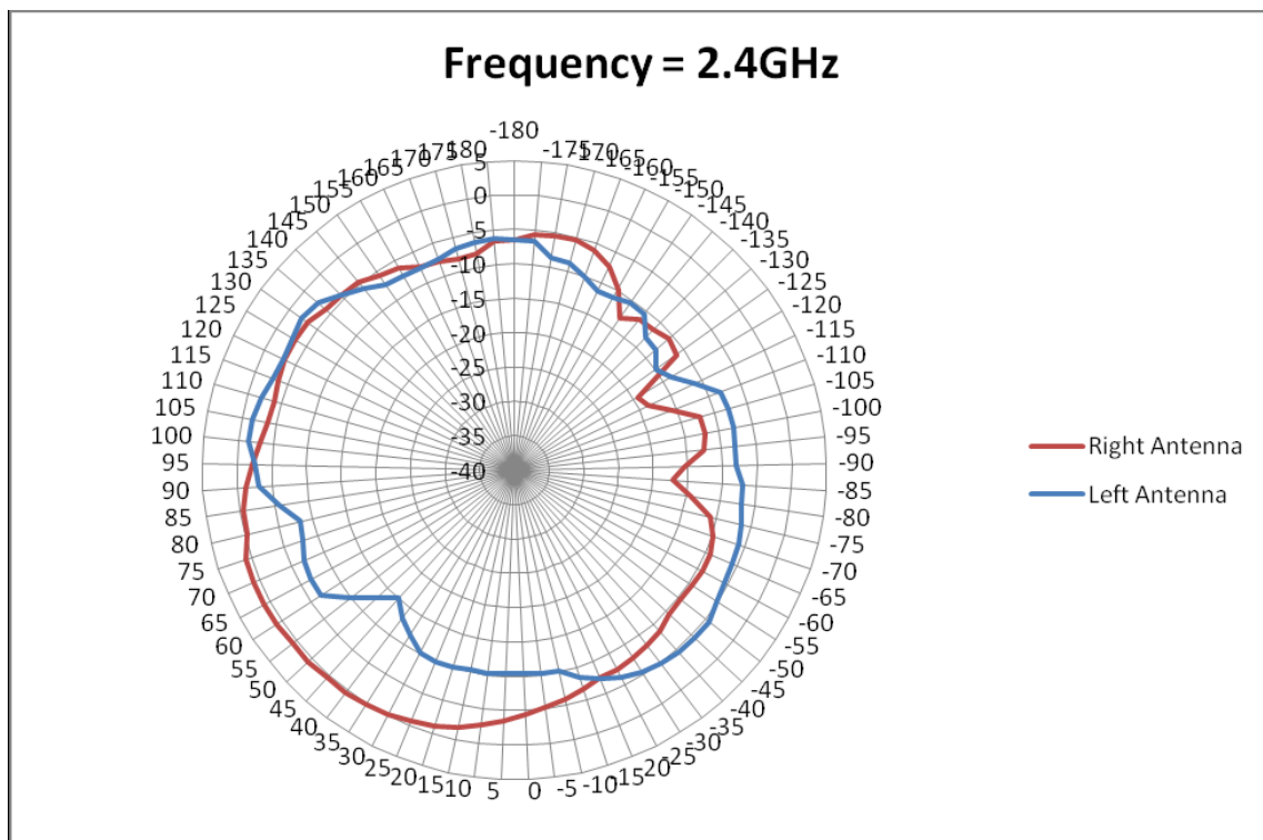
Figure 17 Radiation Plots for 2.400GHz (E1-Plane) Left/Right Antenna
