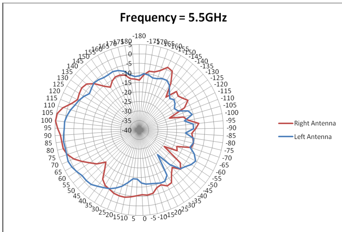
Figure 30 Radiation Plots for 5.500GHz (H-Plane) Left/Right Antenna
