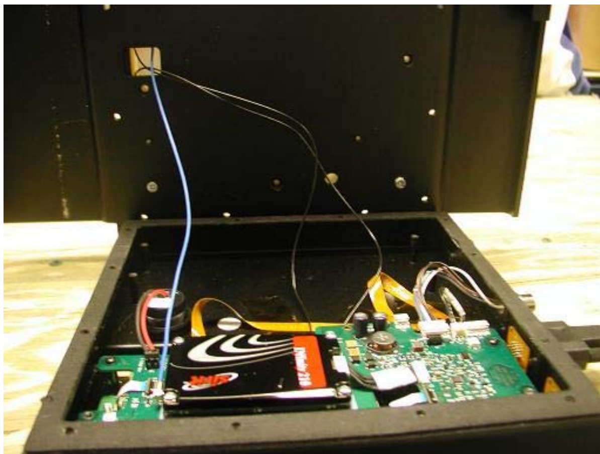
RFID and 802.11b/g modules with cables throughput attached to Antennas
