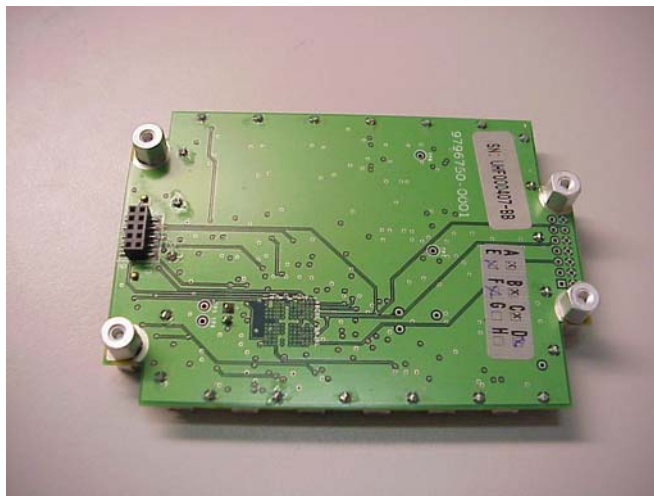
Photo of Bottom Side of Rx Board
