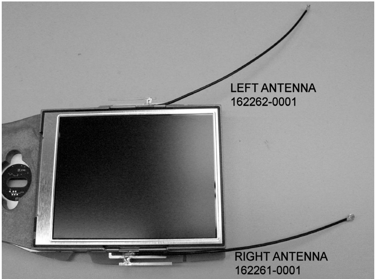
Figure 9: 802.11bg Antenna Locations
