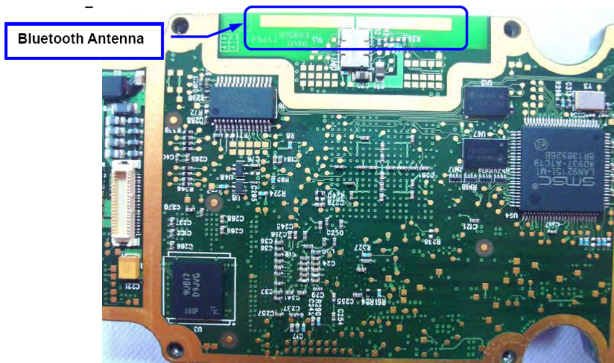
Figure 7: Bluetooth Antenna Location
