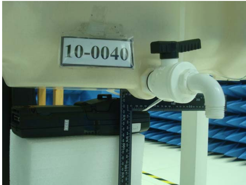
Figure 1. Body SAR Test Setup (Flat Section)
