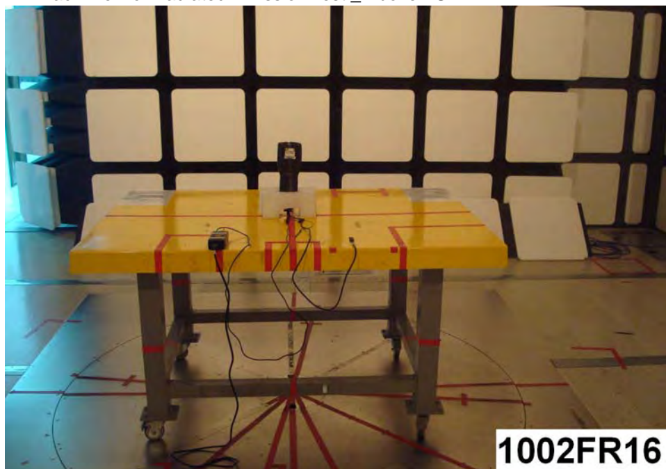
Description : Back View of Radiated Emission Test _ Above 1GHz
