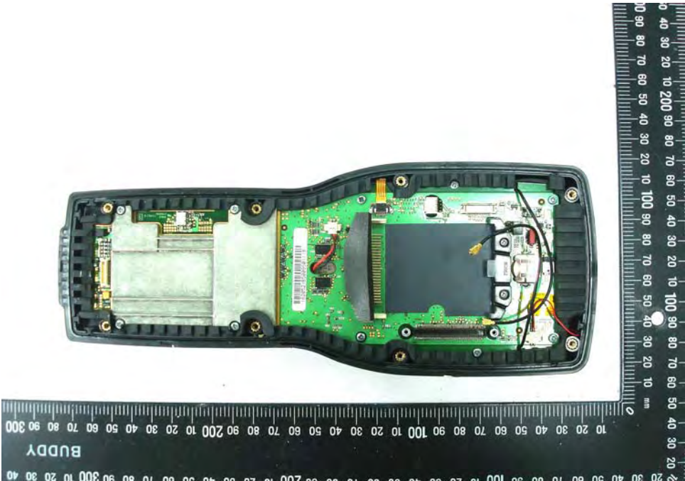
EUT Photo _ 22 of 32
