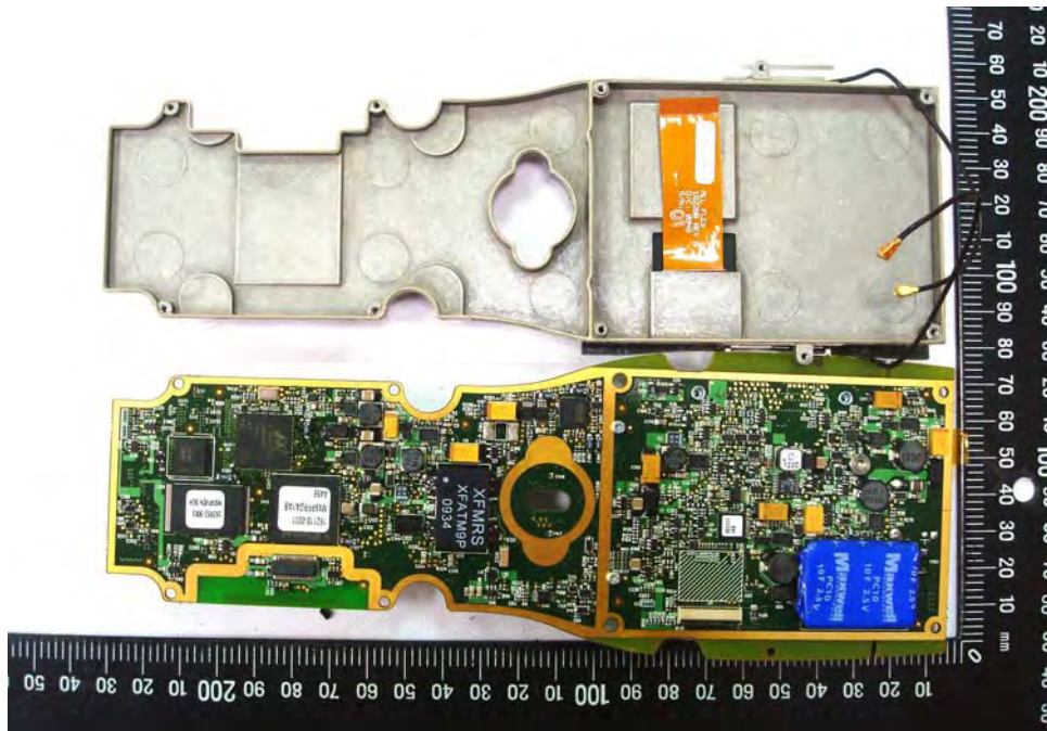
EUT Photo _ 29 of 32
