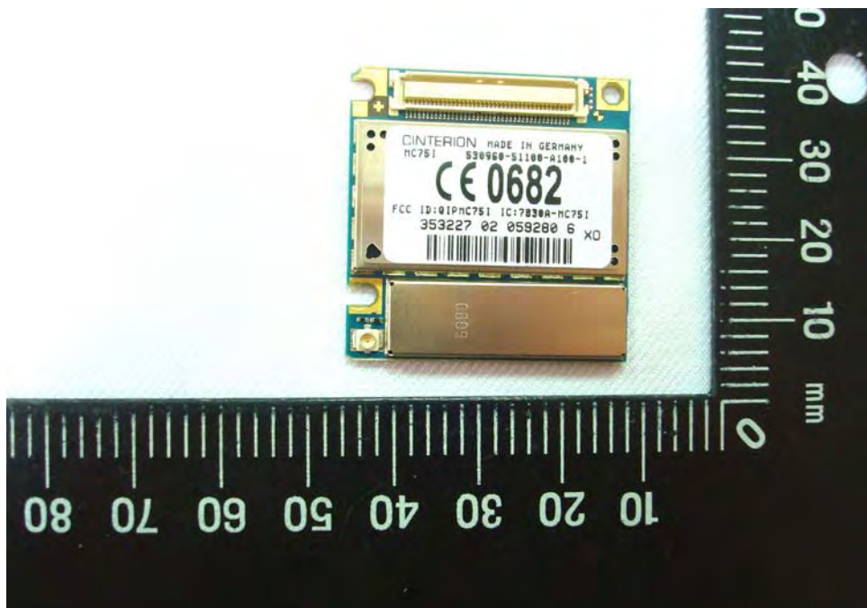
EUT Photo _ 10 of 32
