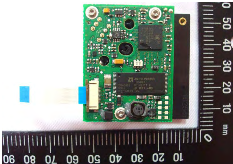
EUT Photo _ 6 of 32
