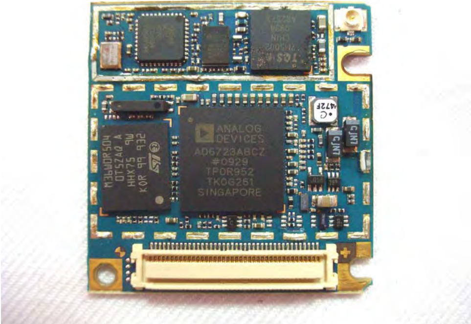
EUT Photo _ 11 of 32 (WWAN Module)
