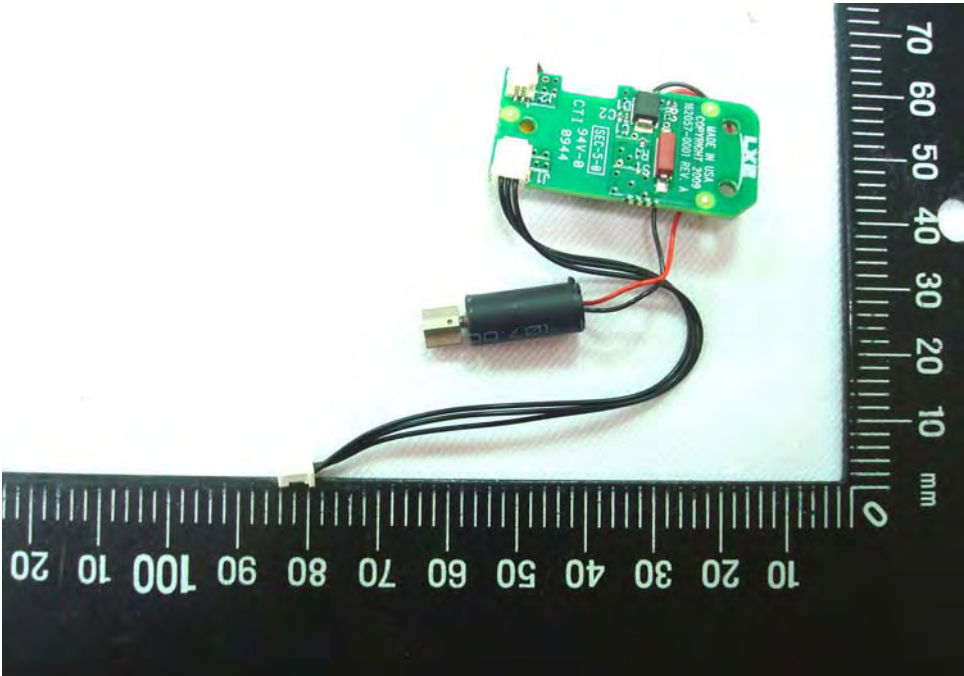
EUT Photo _ 15 of 32
