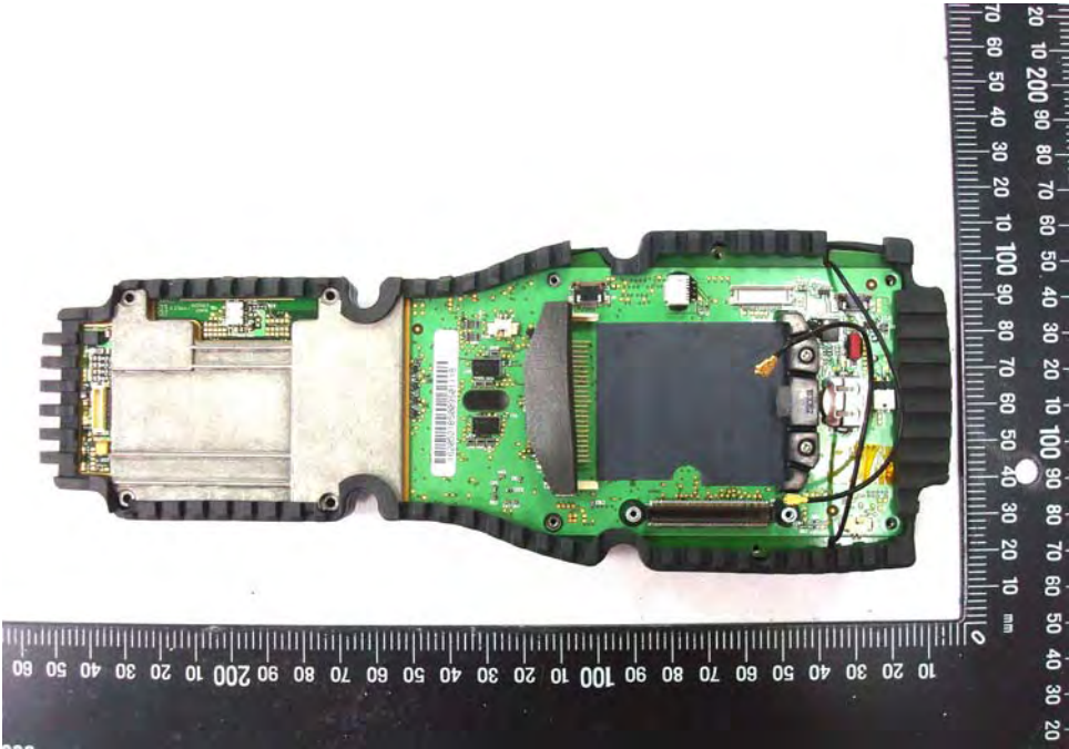
EUT Photo _ 23 of 32
