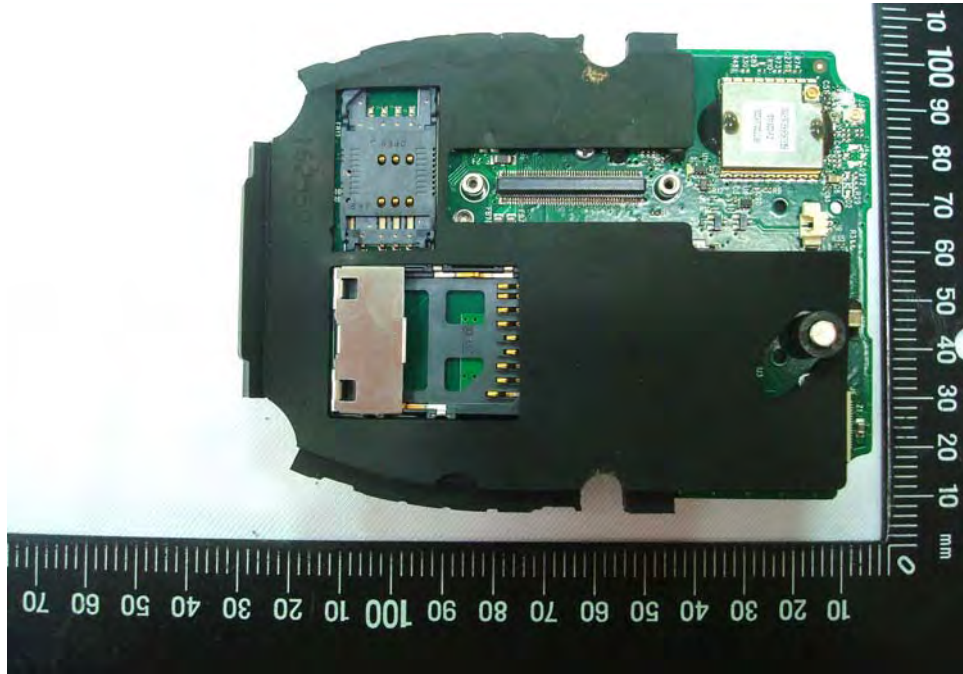
EUT Photo _ 3 of 32
