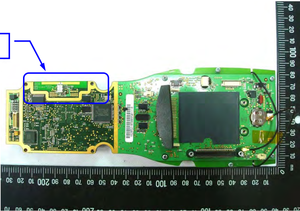
EUT Photo _ 24 of 32
