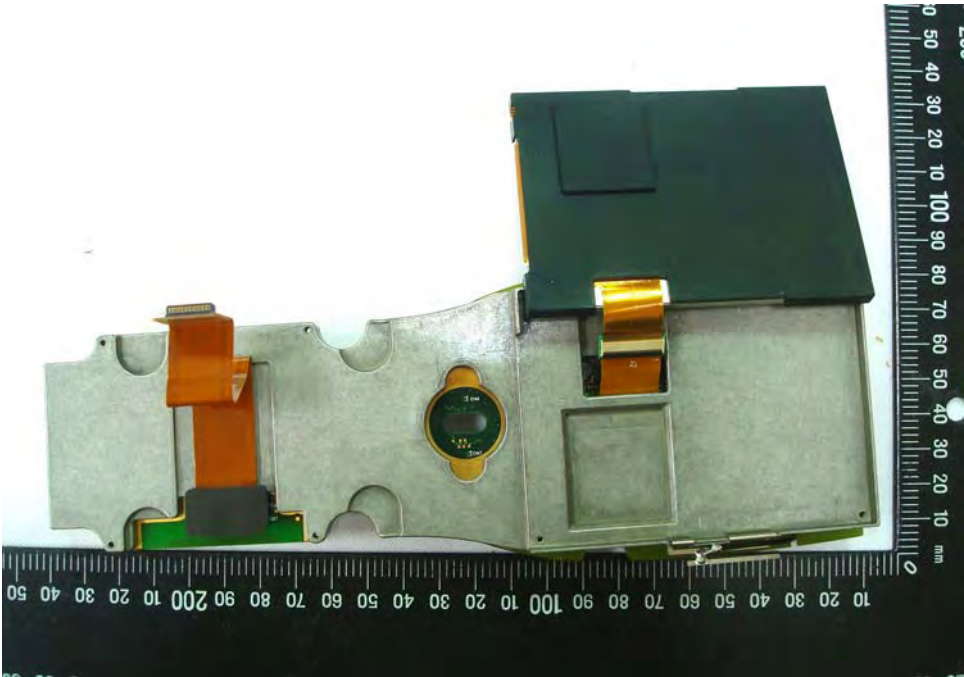
EUT Photo _ 28 of 32
