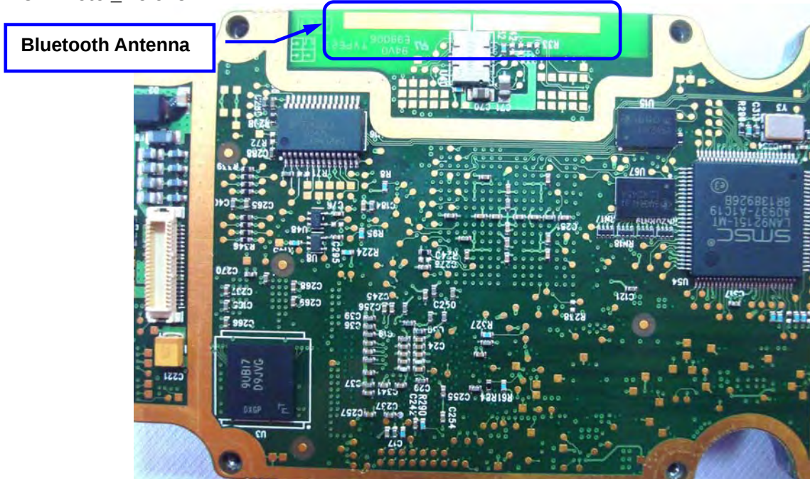
EUT Photo _ 25 of 32
