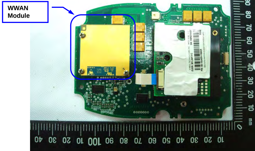
EUT Photo _ 5 of 32
