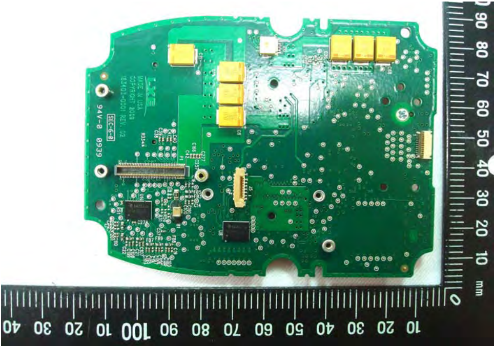
EUT Photo _ 13 of 32
