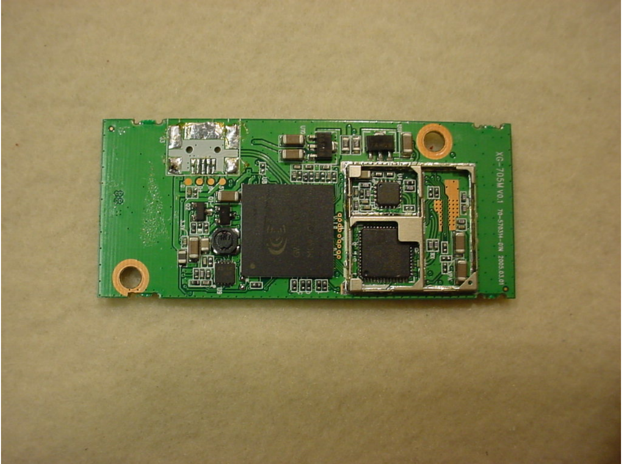
Figure 7: Internal Photos – Radio Module Back View
