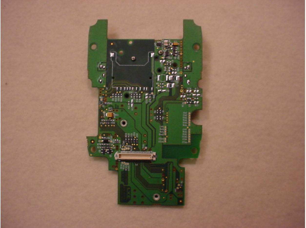
Figure 4: Internal Photos – Carrier Board Back View
