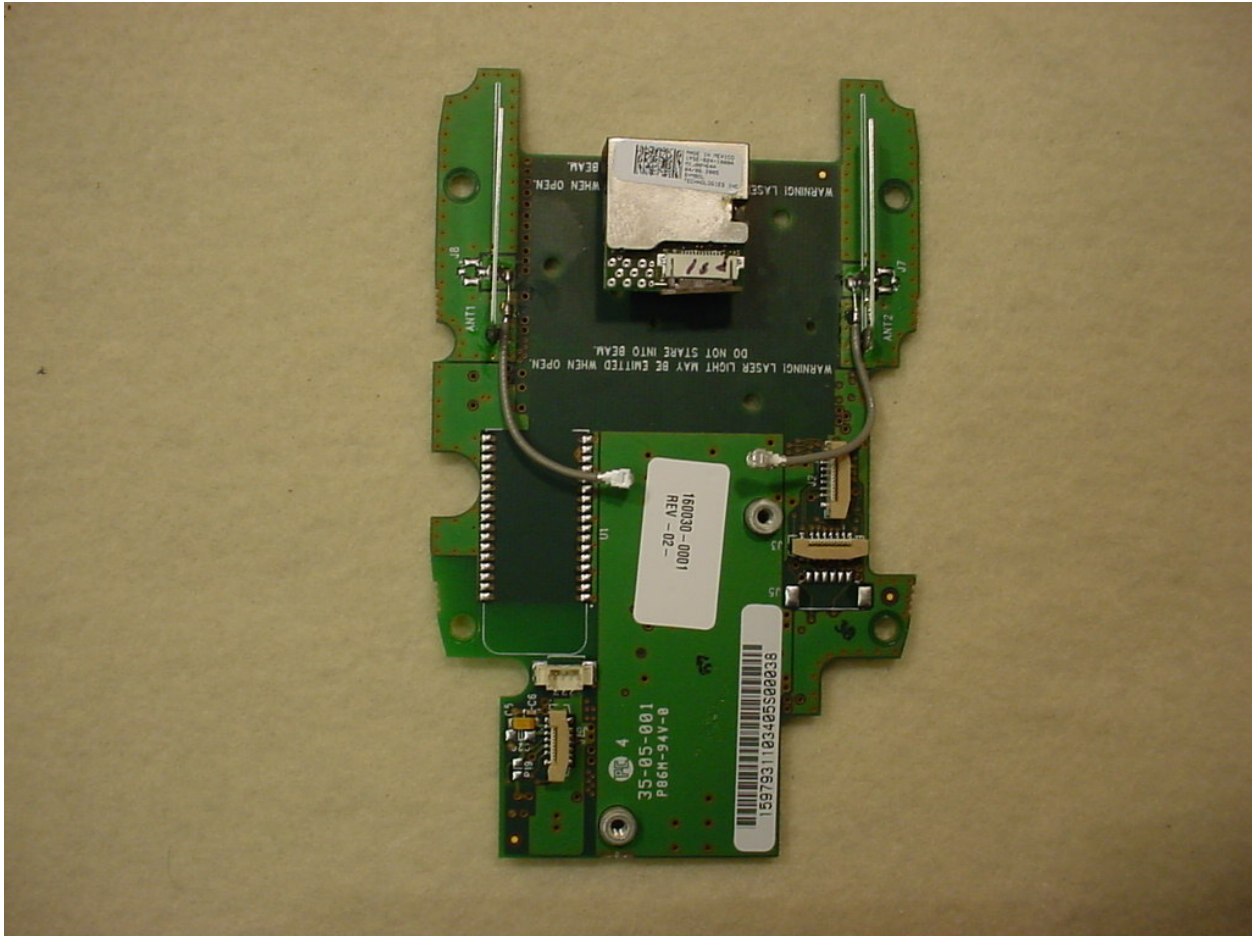
Figure 3: Internal Photos – Carrier Board Front View
