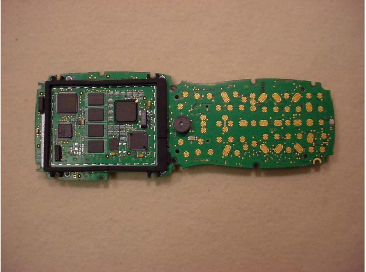
Figure 2: Internal Photos – CPU Board Back View
