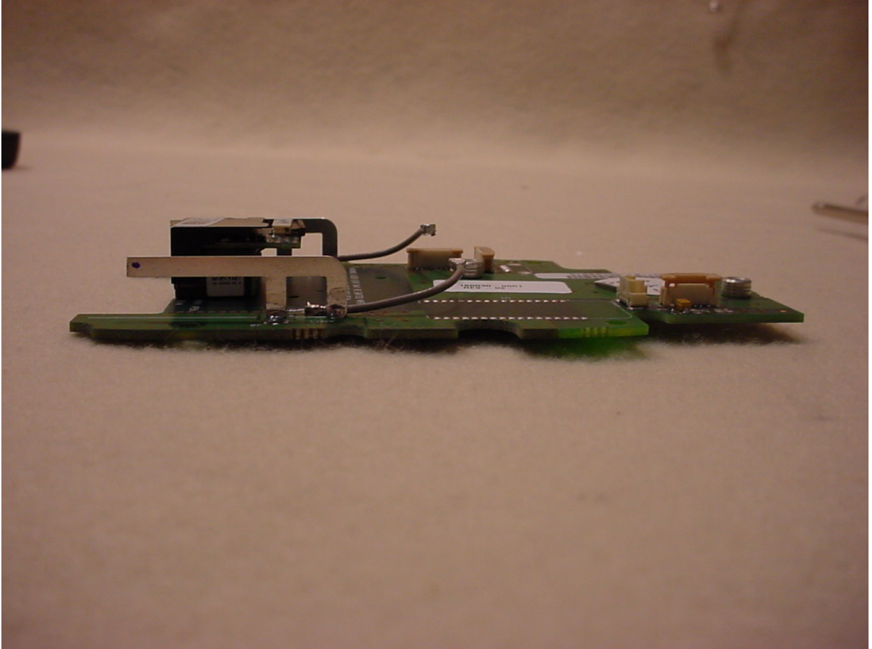
Figure 5: Internal Photos – Carrier Board Side View
