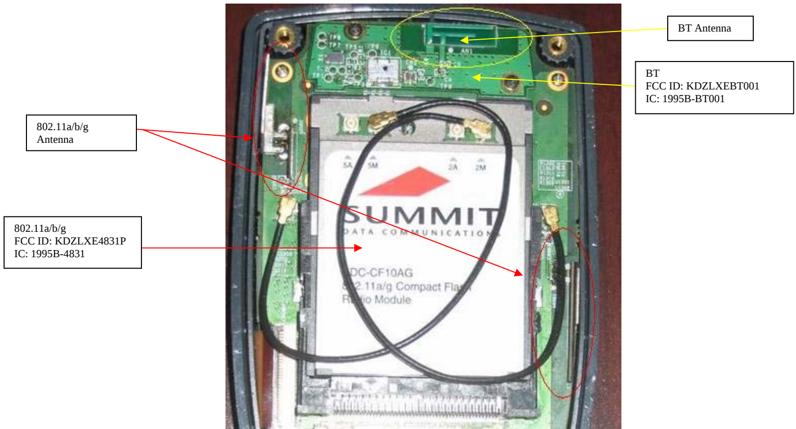
Figure 2: Internal photo showing antenna collocation and module placement.
