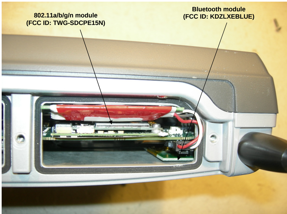
Figure 2: Module Locations in Host VX8 Terminal Host
