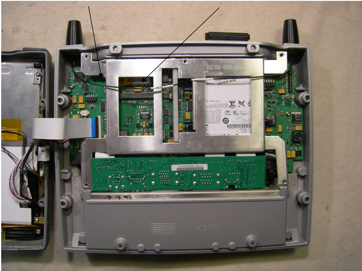
Figure 1: Module Locations in Host VX8 Terminal Host
