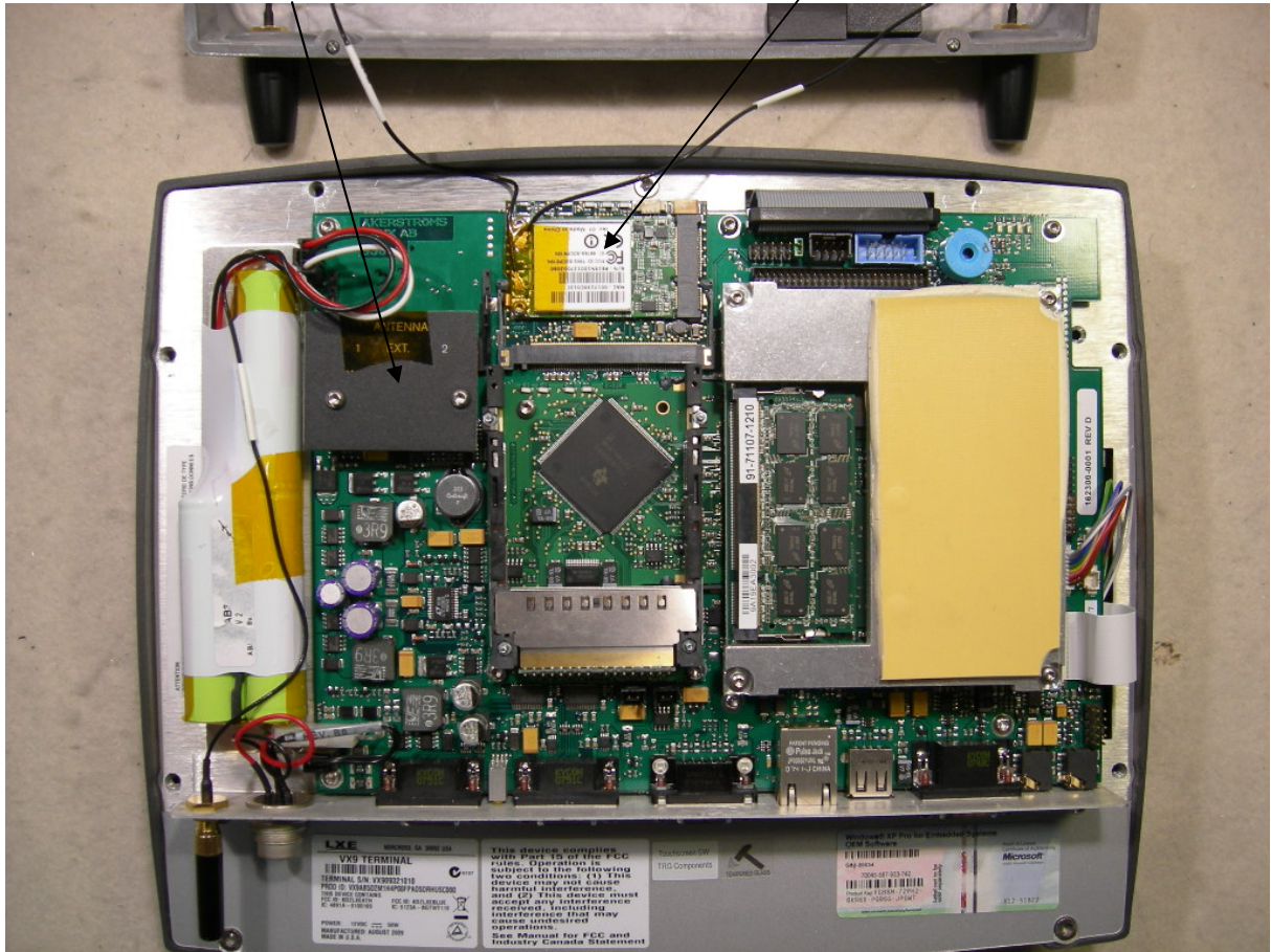
Figure 3: Module Locations in Host VX9 Terminal Host
