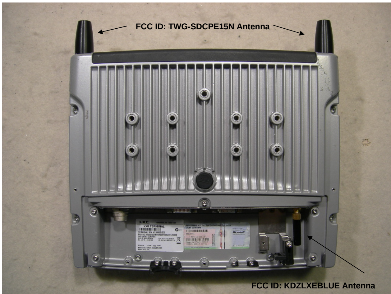
Figure 2: VX8 Terminal Host Back
