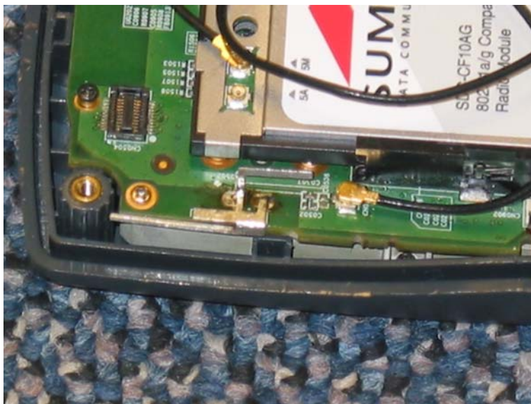
Left Antenna
