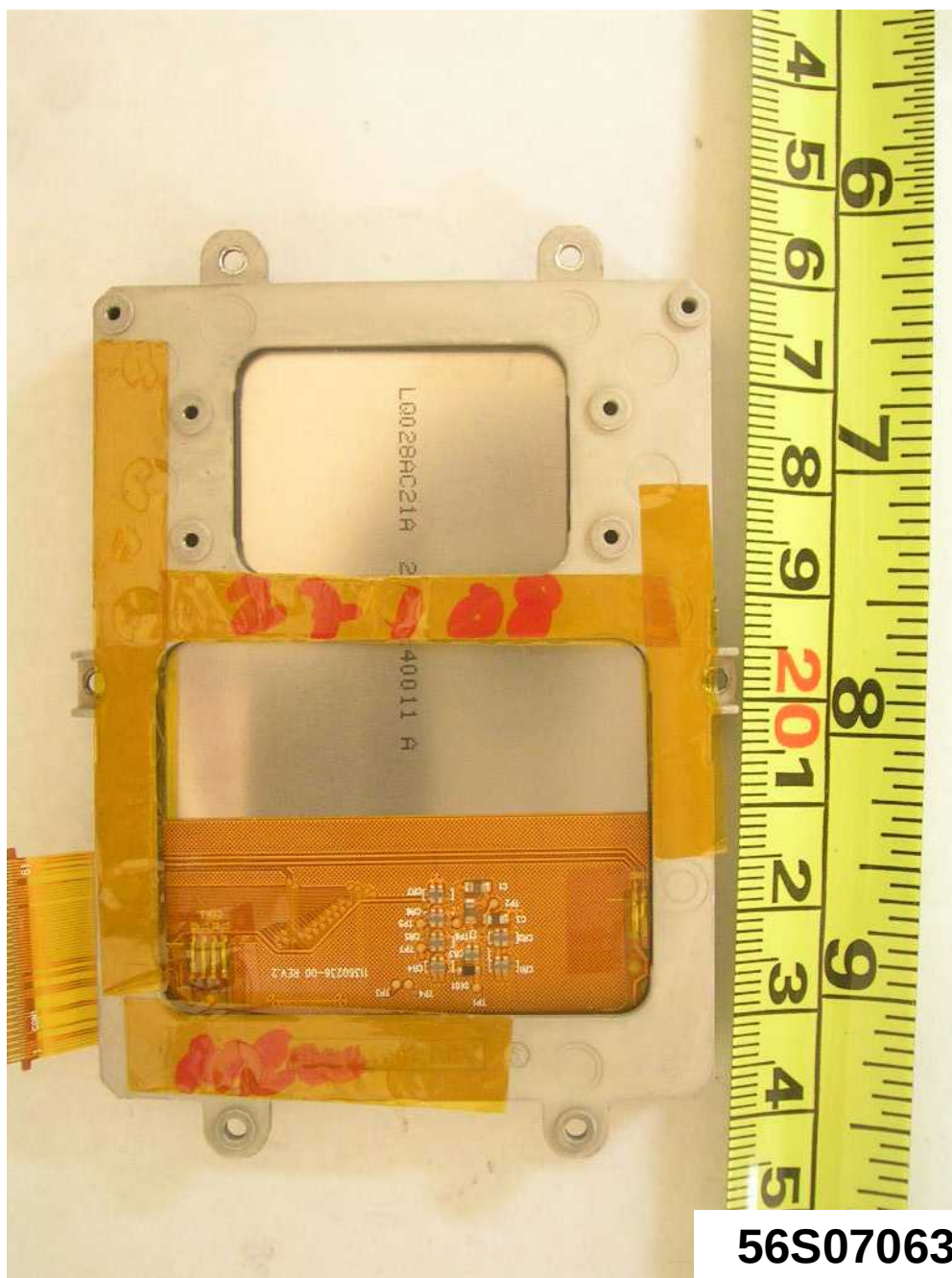
LCD Display PCB Trace Side
