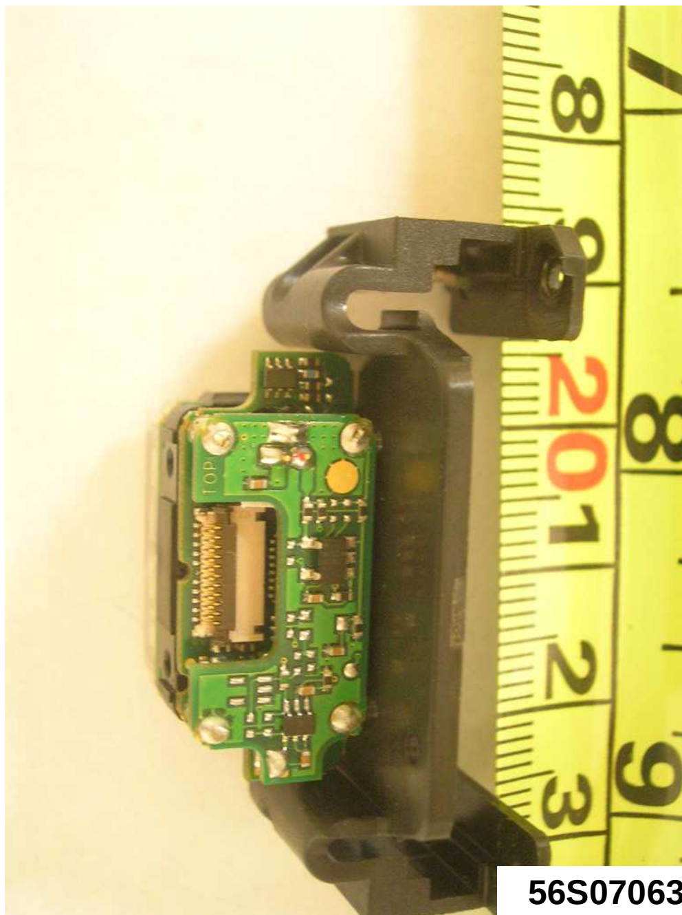
Scanner Board PCB Trace Side
