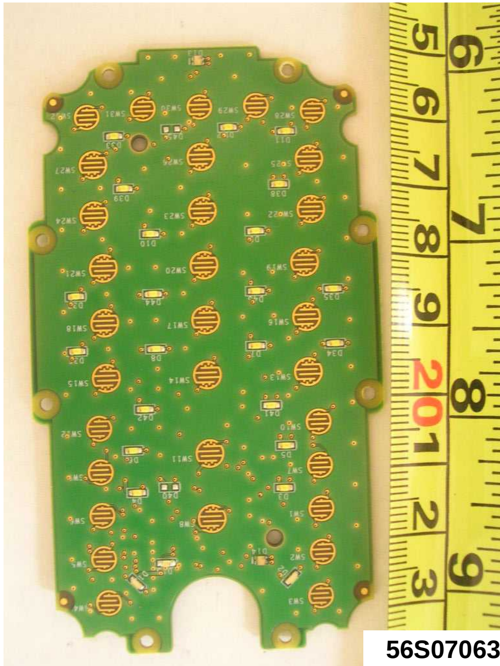
Key Pad Board PCB Component Side
