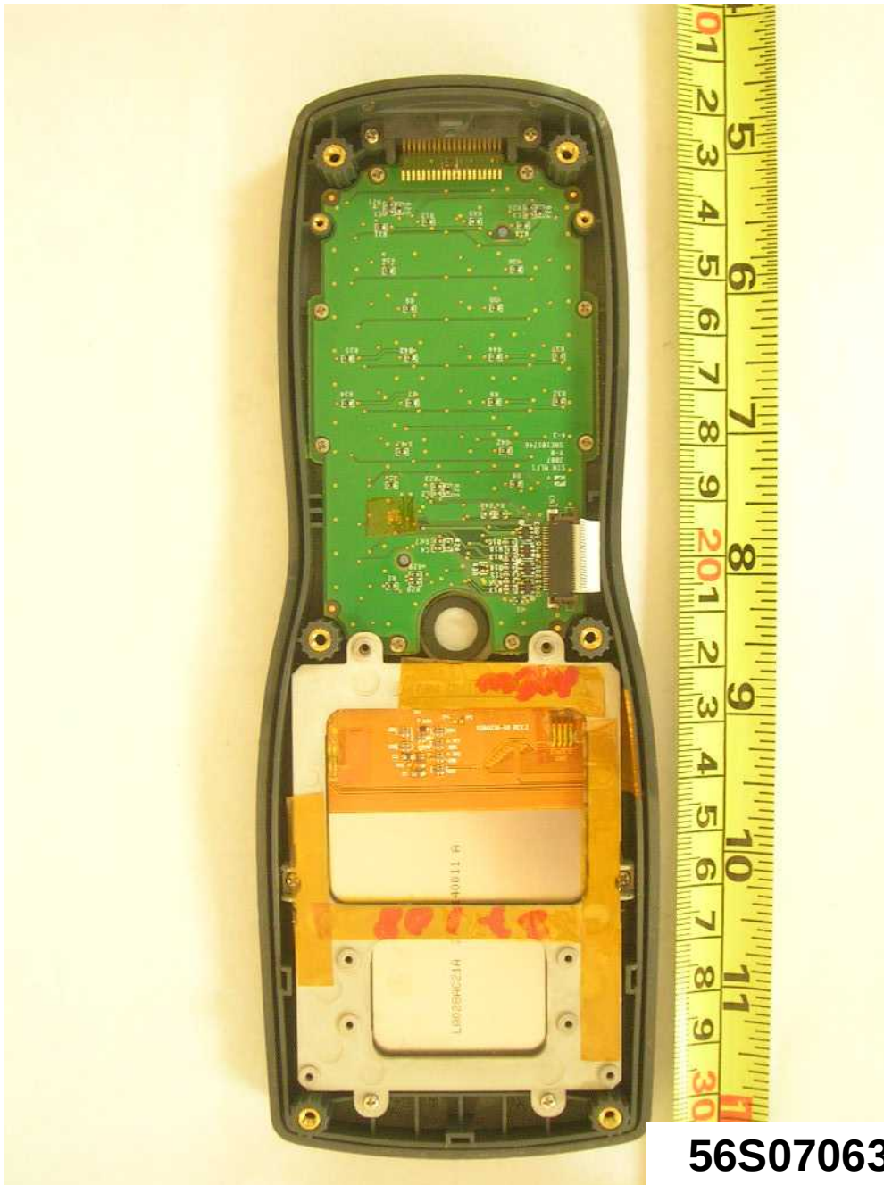
Top Housing Internal View 2
