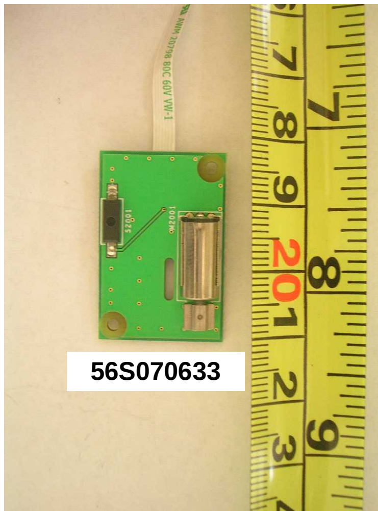
Vibrator Board PCB Component Side
