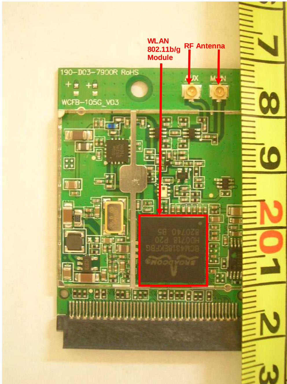
WLAN 802.11b/g Module Circuit with RF Shield Removed
