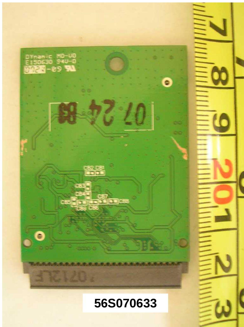
WLAN 802.11b/g Module Board PCB Trace Side
