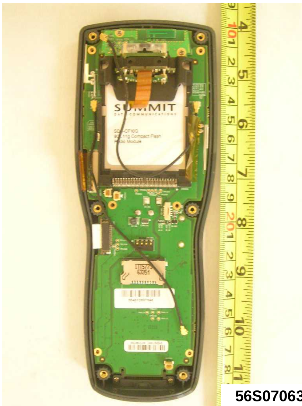
Top Housing Internal View 1
