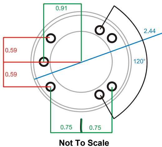
Figure 36 RAM Assembly Footprint
