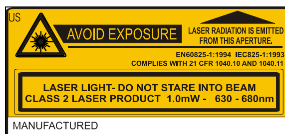
Figure 2 Caution Label – Class 2 Laser Scanner
