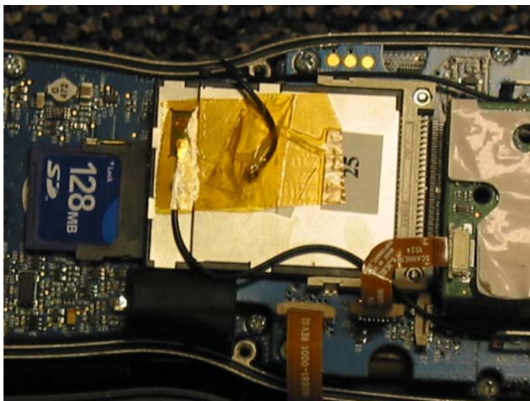
RF Module in Unit
