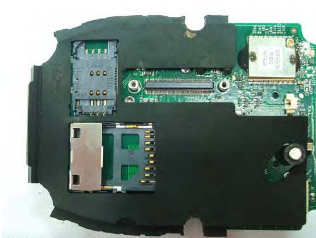
Figure 2: Cellular Modem Board
