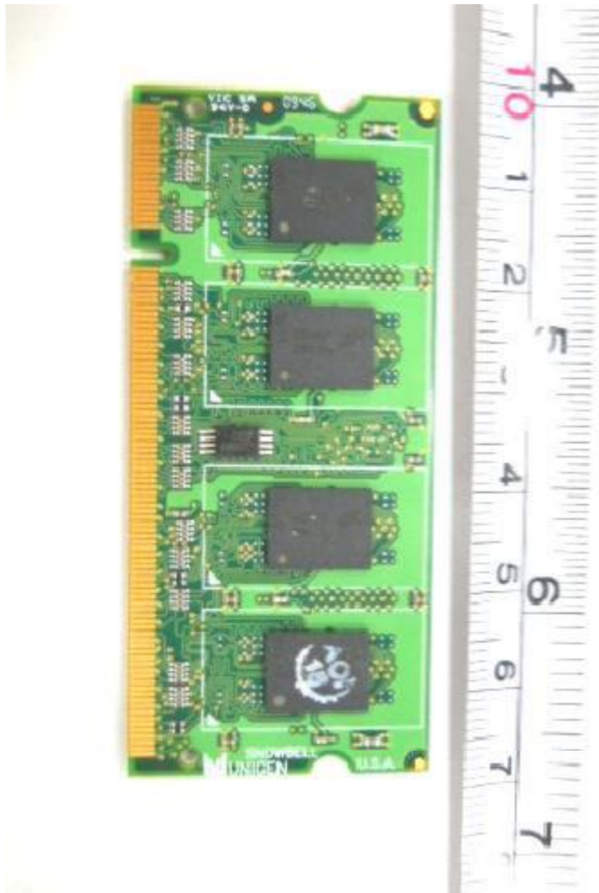
DDR2-SODIMM PCB Component Side
