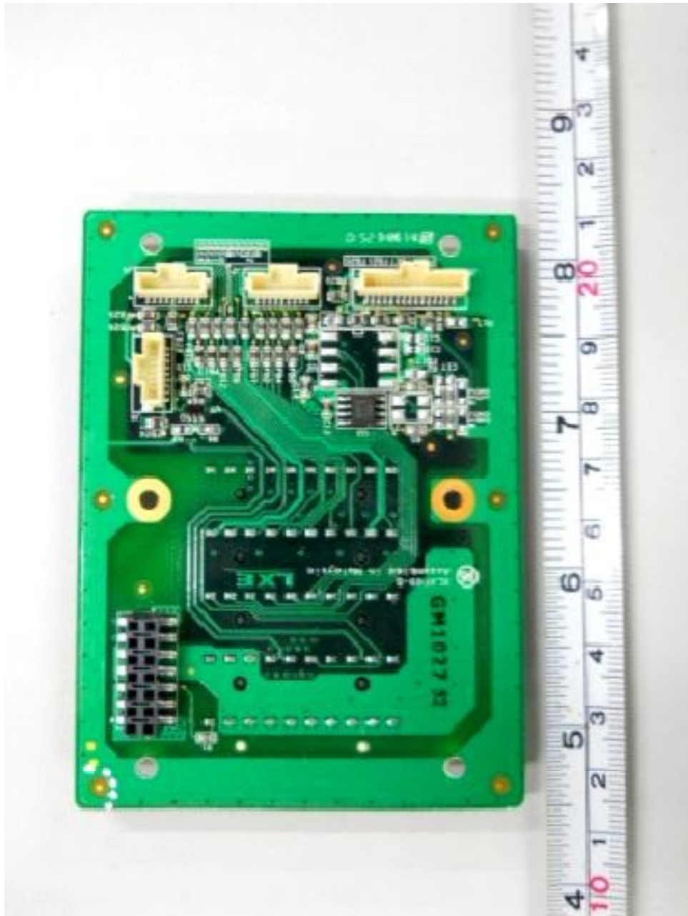
Docking Interface PCB Trace Side
