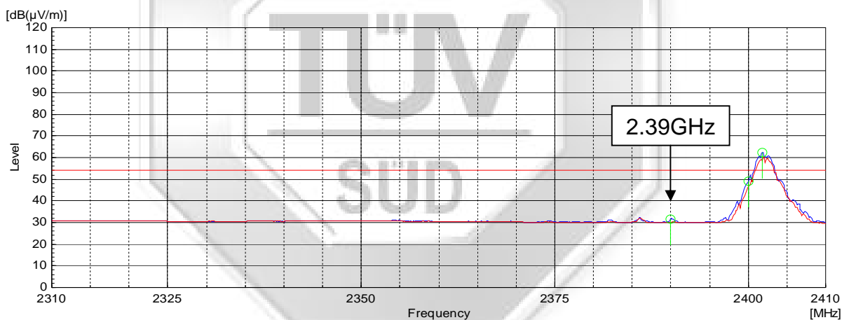
Plot 31 – Average Plot at Lower Band Edge at 2.4000GHz
