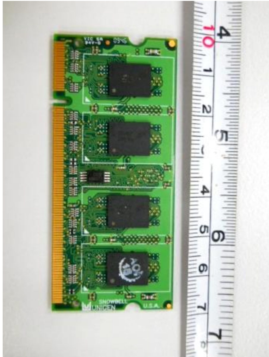
DDR2-SODIMM PCB Component Side
