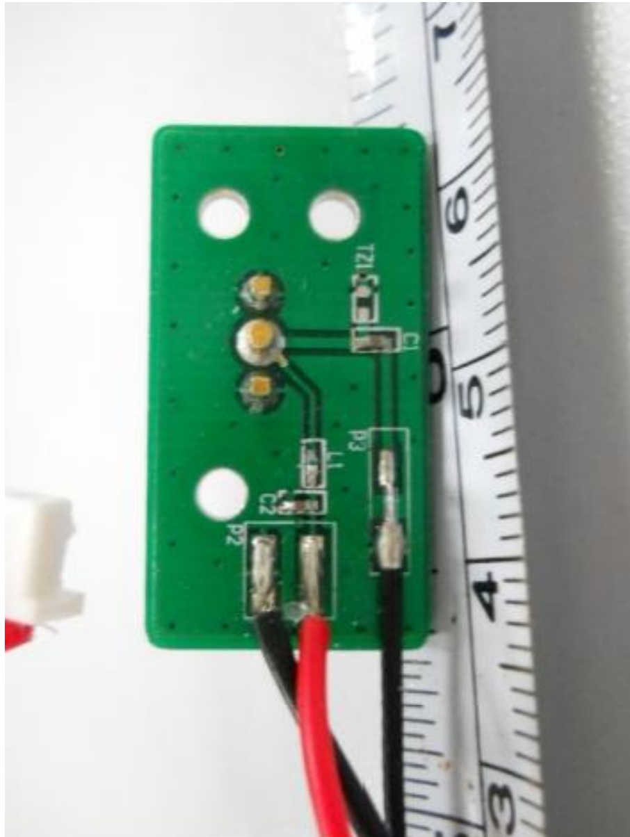
GPS Power-3.3V PCB Trace Side
