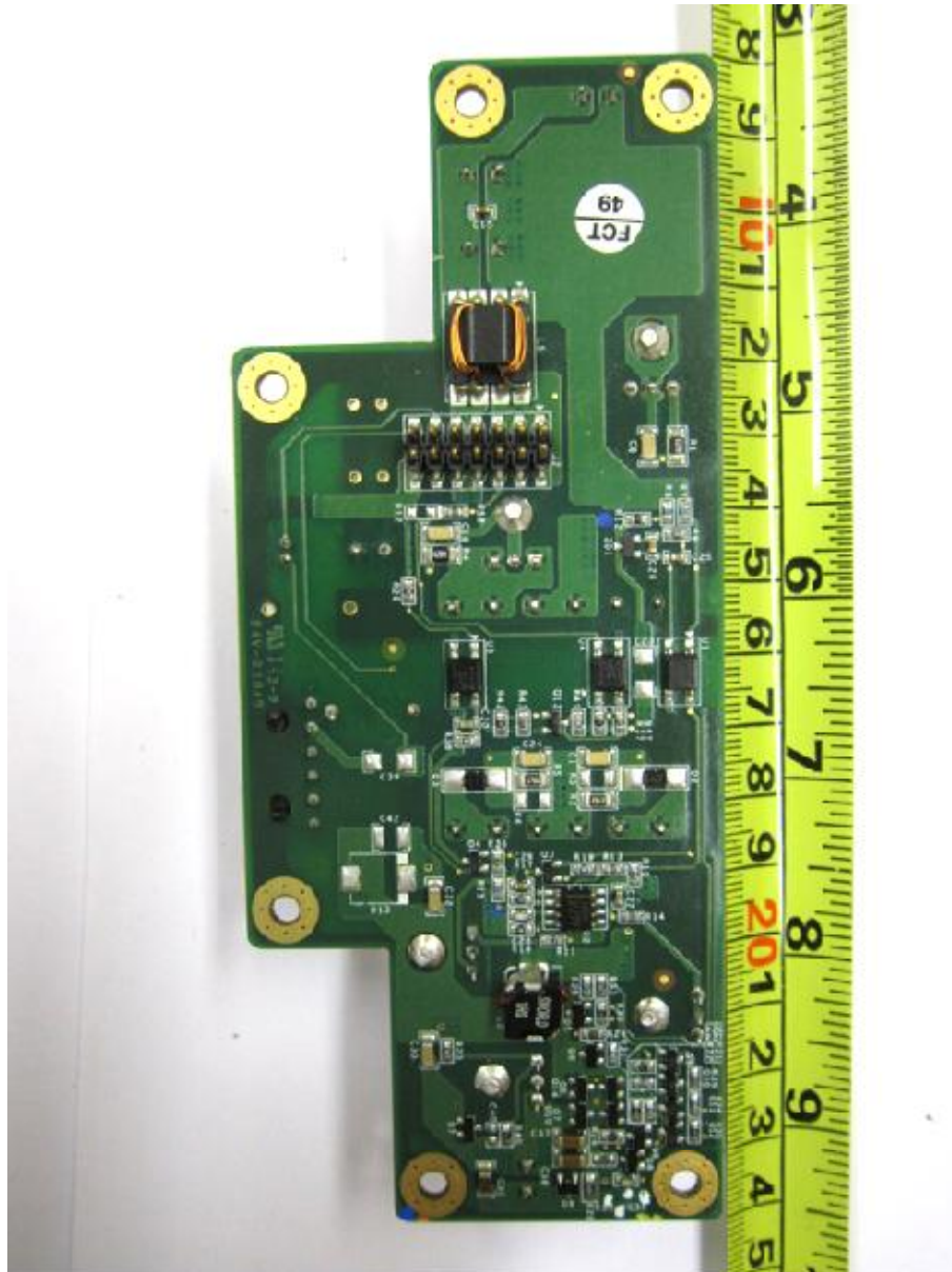
DC-DC Converter PCB Trace Side
