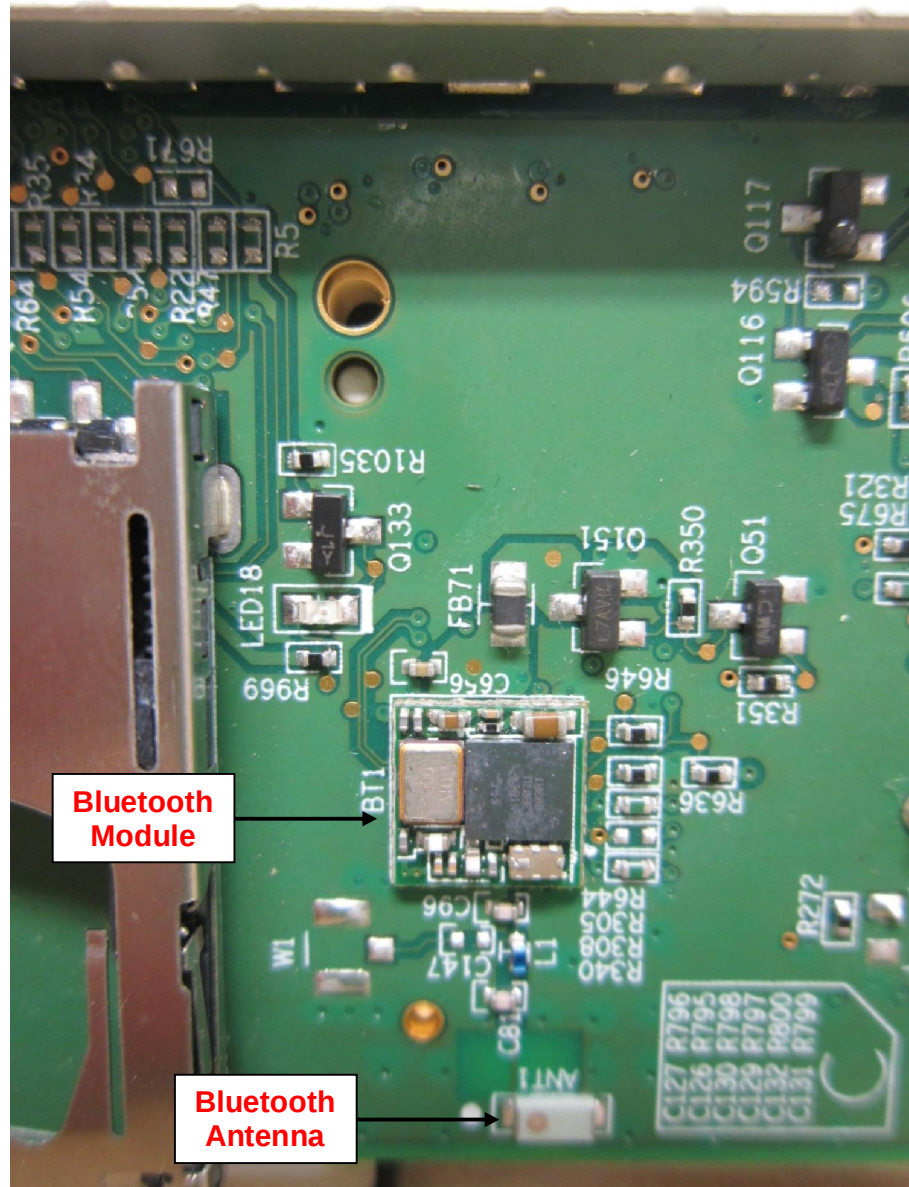
Bluetooth-Module PCB Component Side
