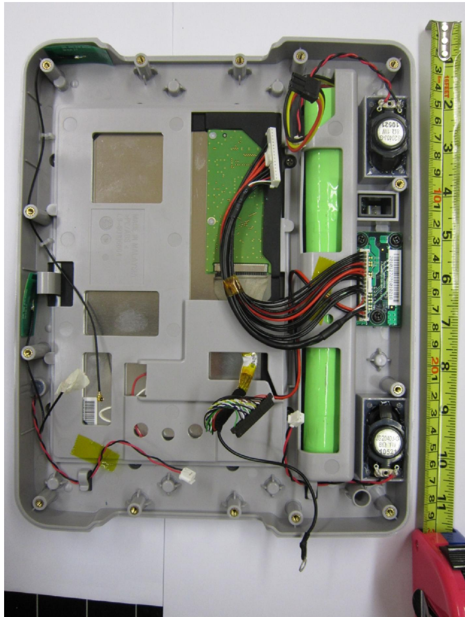
EUT Top Housing Internal View 1
