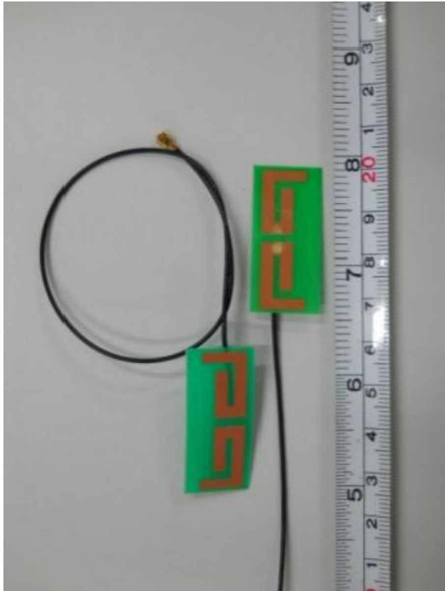
Internal WLAN Antennas-PCB Module PCB Component Side
