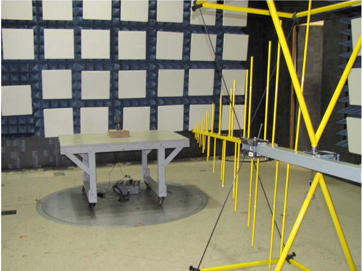
Figure 4: Radiated Emissions – 30 MHz to 1000 MHz.
