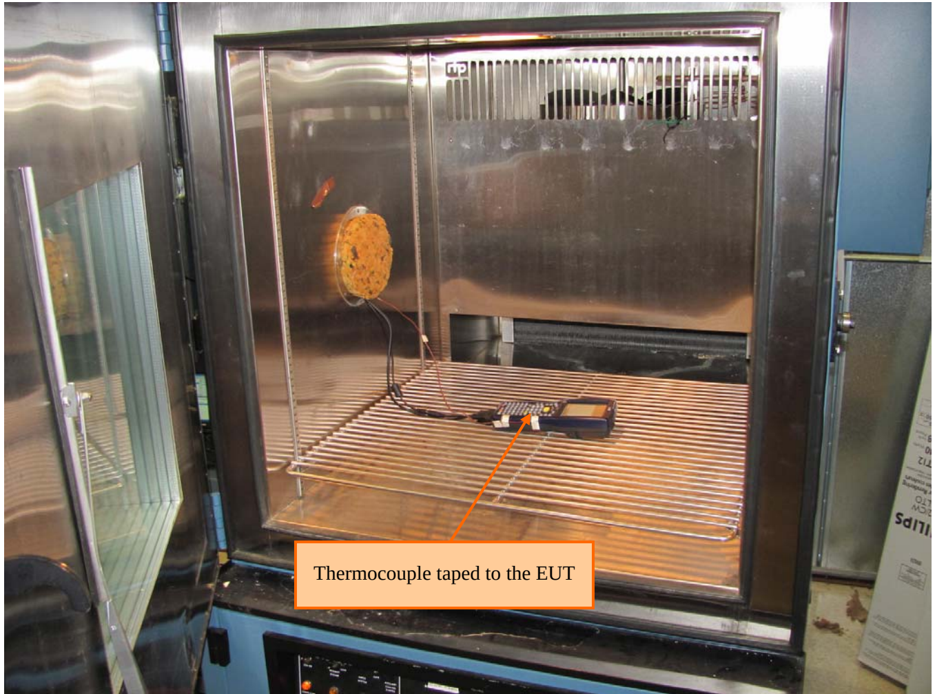
Figure 8 – Photo of EUT inside temperature chamber for Voltage Requirement tests.
