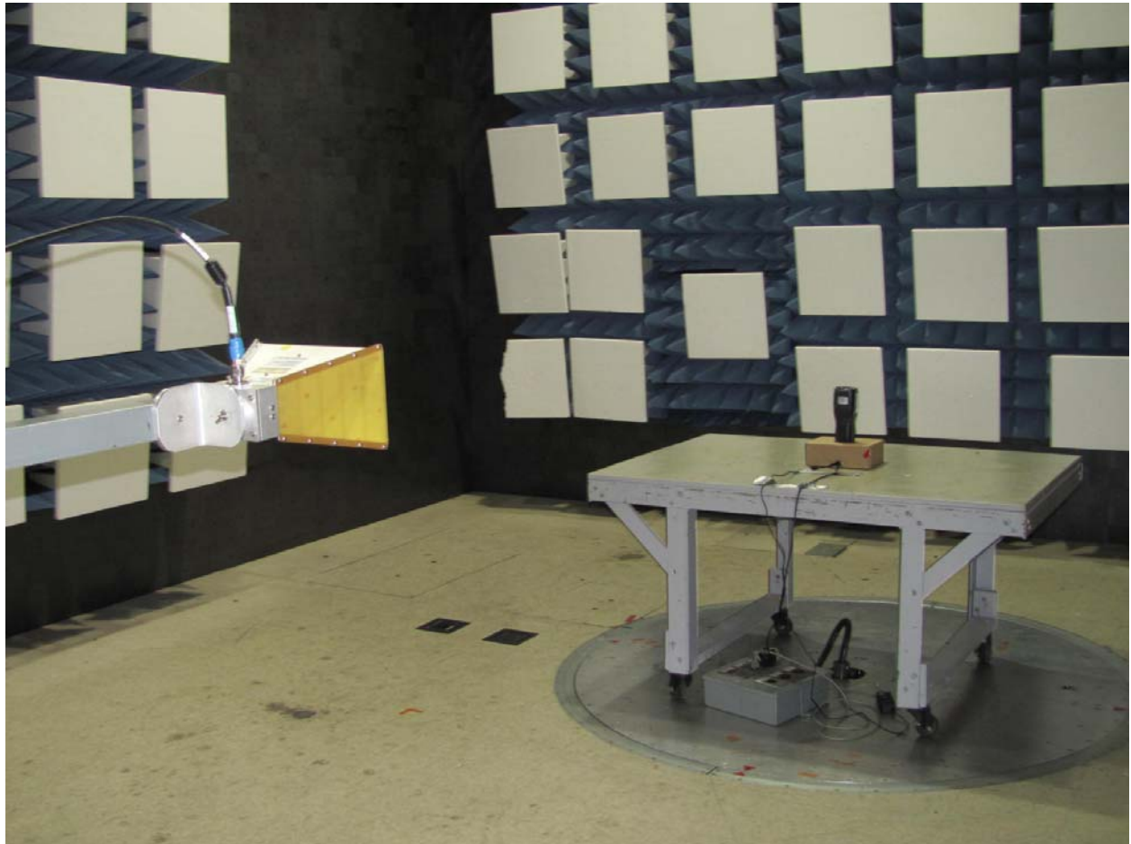
Figure 5: Radiated Emissions – 1 GHz to 18 GHz.
