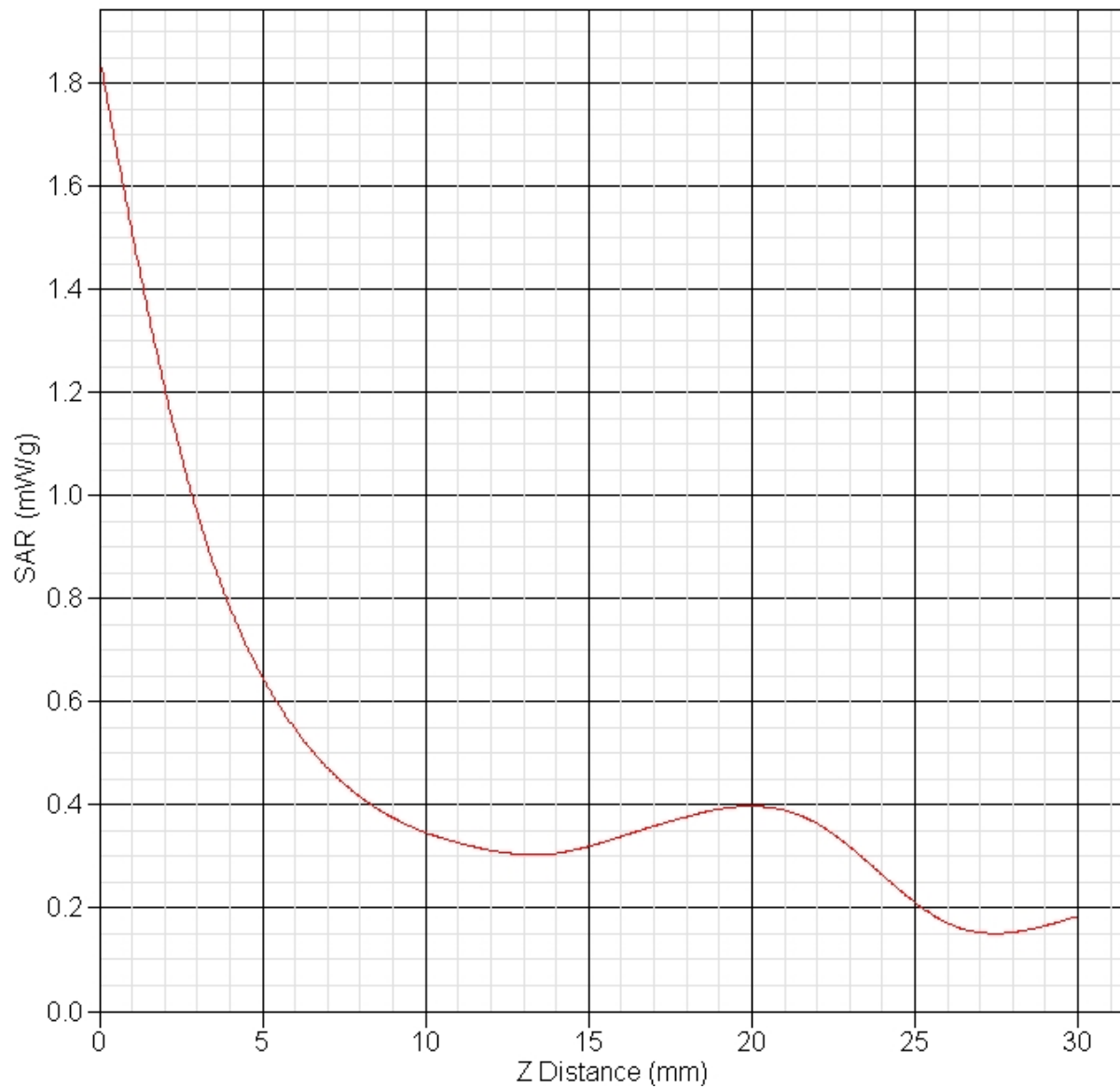
SAR-Z Axis at Hotspot x:0.09 y:14.89
