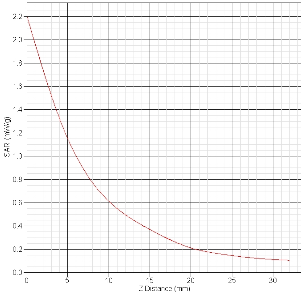
SAR-Z Axis at Hotspot x:8.03 y:6.90
