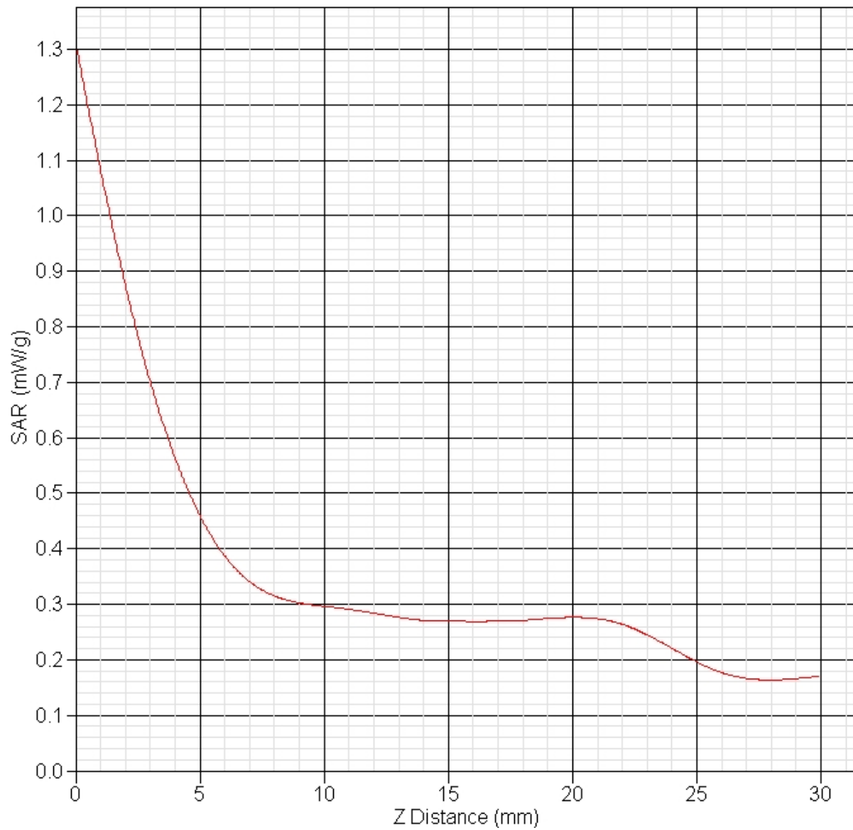
SAR-Z Axis at Hotspot x:7.02 y:7.87
