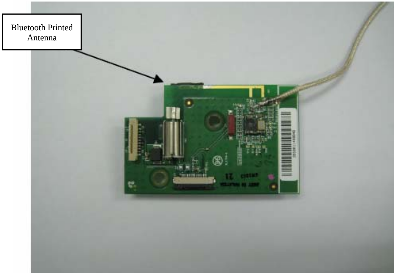
Figure 2: Location of Bluetooth Antenna, Gain: 3dBi
