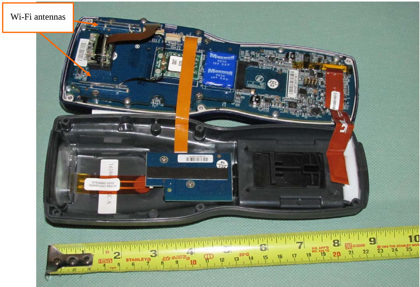
Figure 1: View with back cover off.
