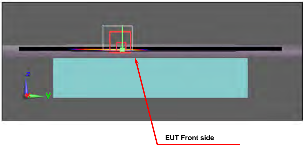
Body SAR Test Setup (Flat Section)
