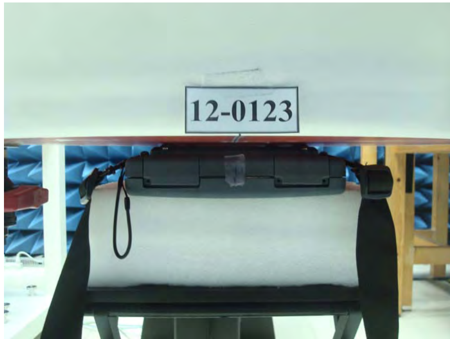
Body Setup (EUT with Thick Battery and Shoulder strap, Back surface to phantom 0mm)
