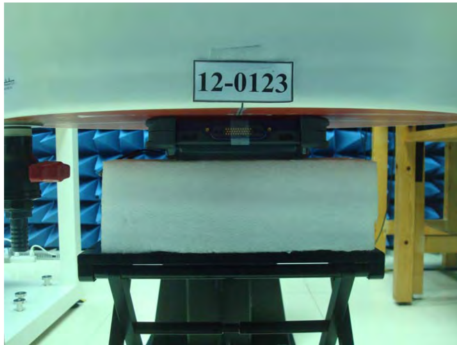
Body Setup (EUT with Thick Battery, Front surface to phantom 0mm)
