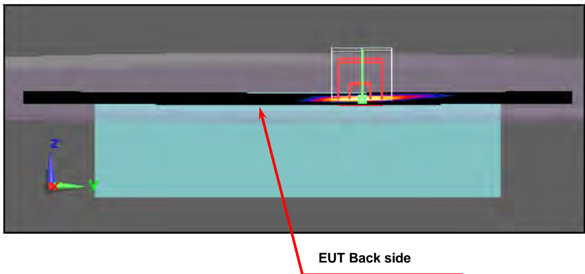
Body SAR Test Setup (Flat Section)
