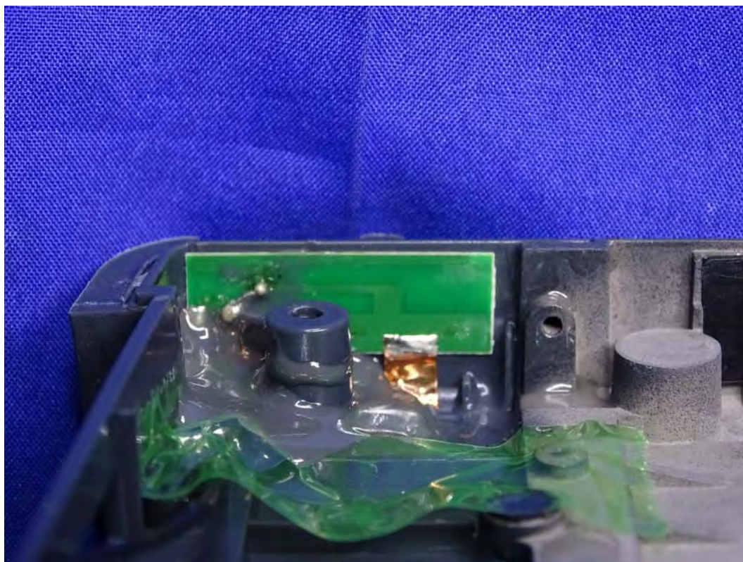
(18) EUT Photo-Antenna
