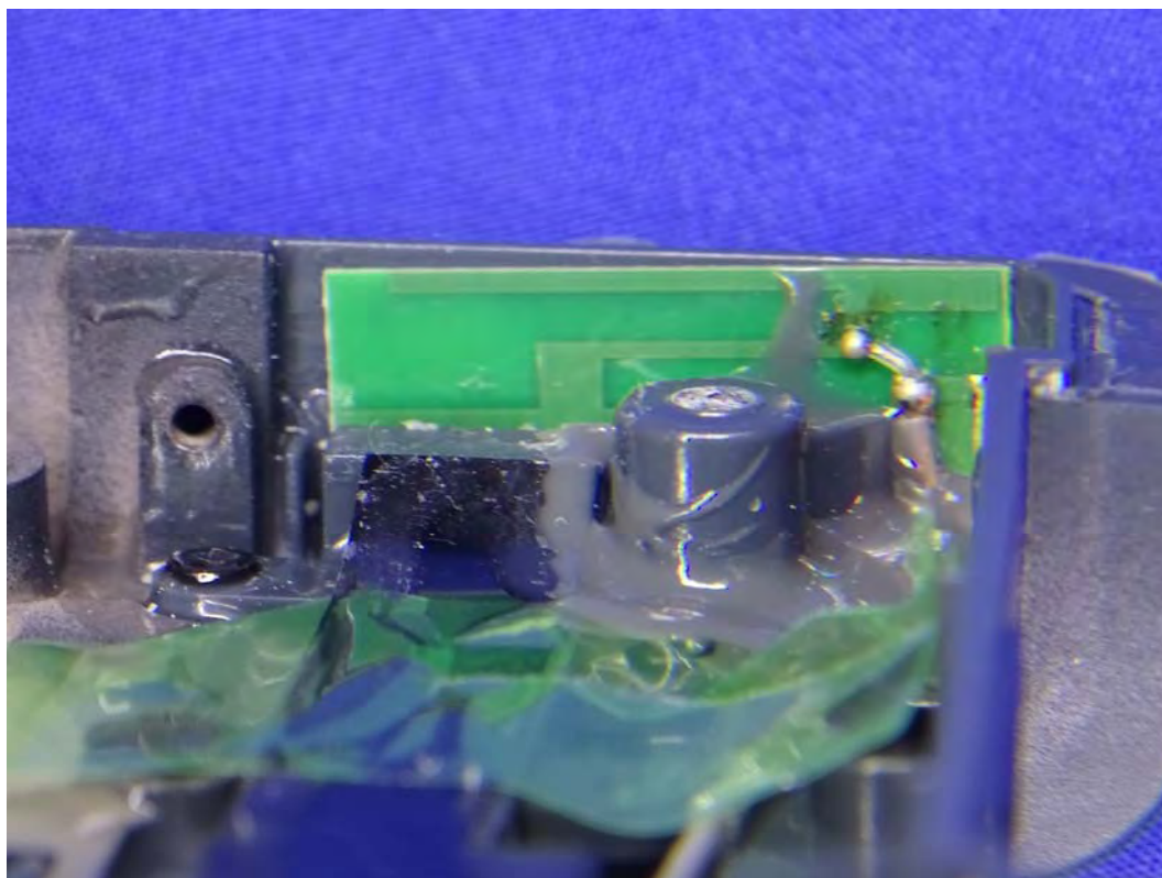
(19) EUT Photo-Antenna
