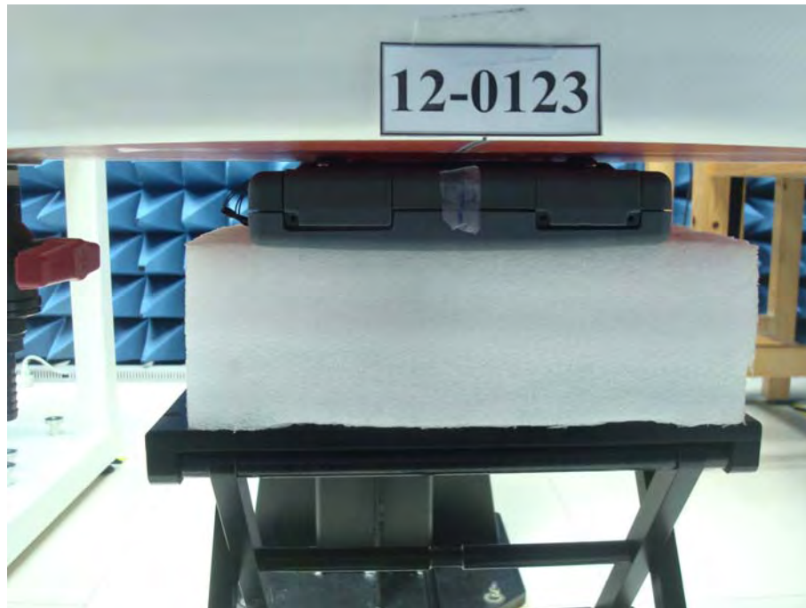
Body Setup (EUT with Hip Pad Battery, Back surface to phantom 0mm)
