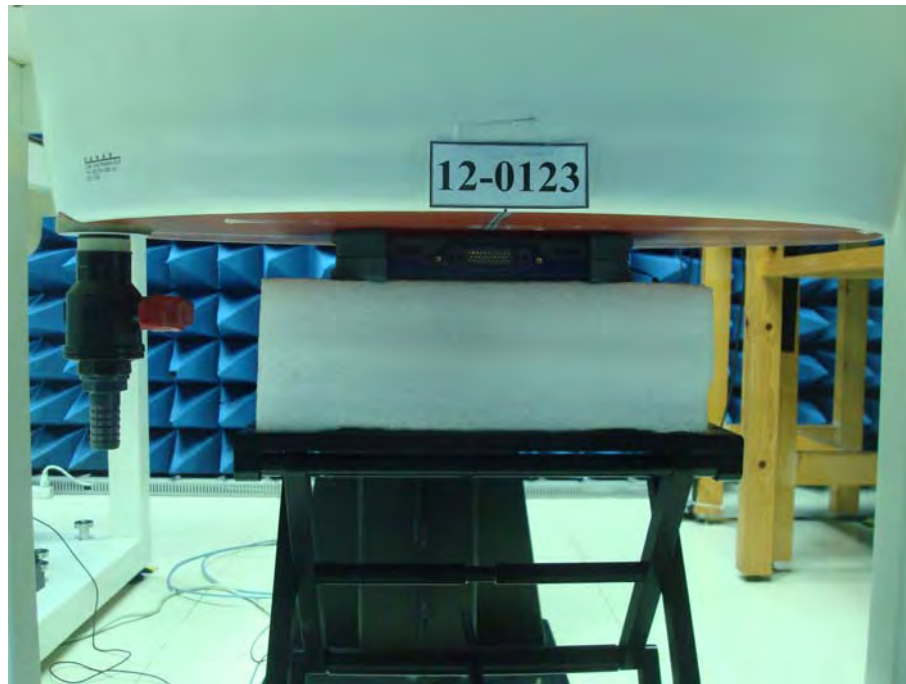
Body Setup (EUT with Internal Battery, Front surface to phantom 0mm)
