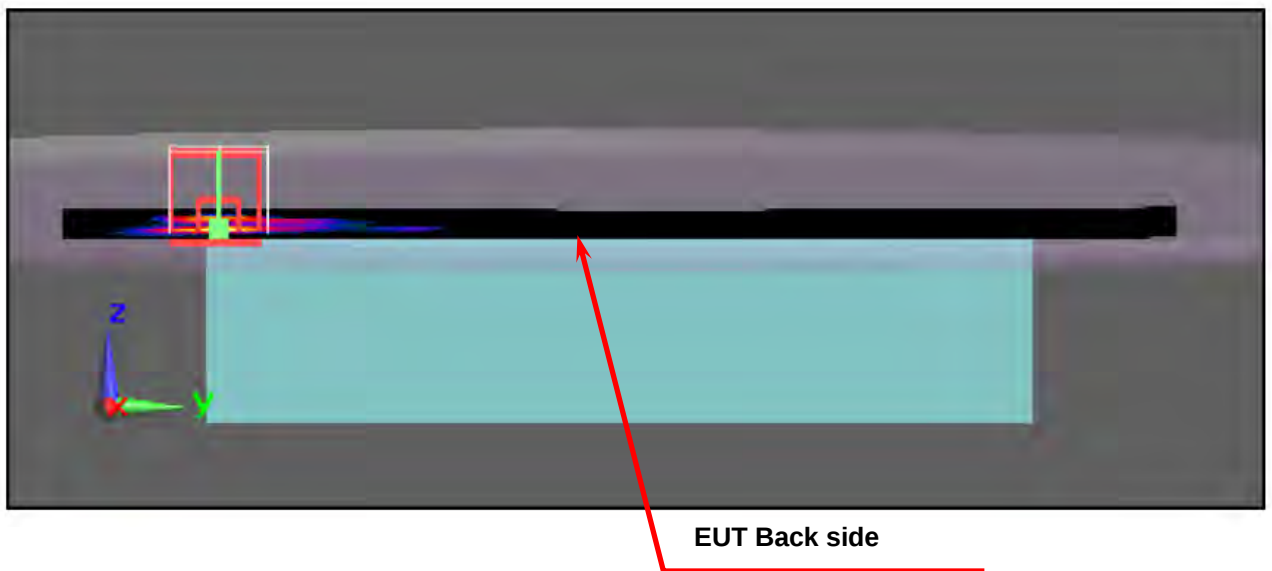
Body SAR Test Setup (Flat Section)
