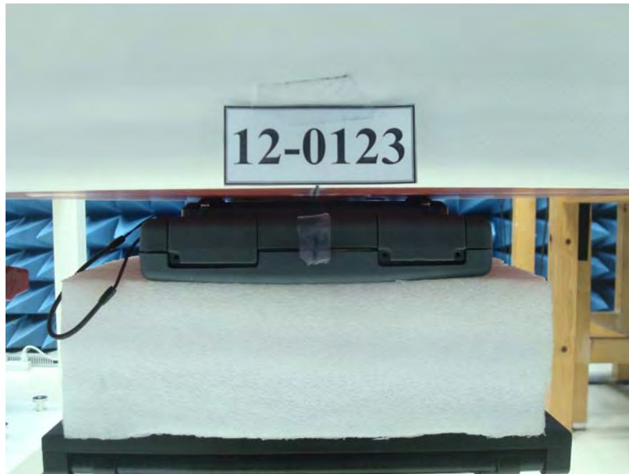
Body Setup (EUT with Thick Battery, Back surface to phantom 0mm)
