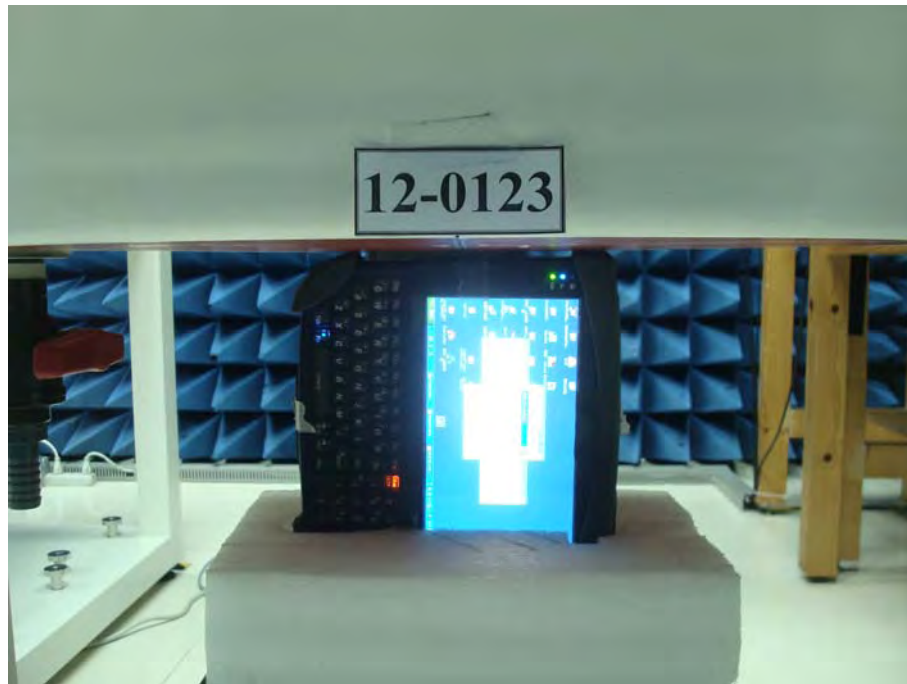
Body Setup (EUT with Internal Battery, Edge Left to phantom 0mm)
