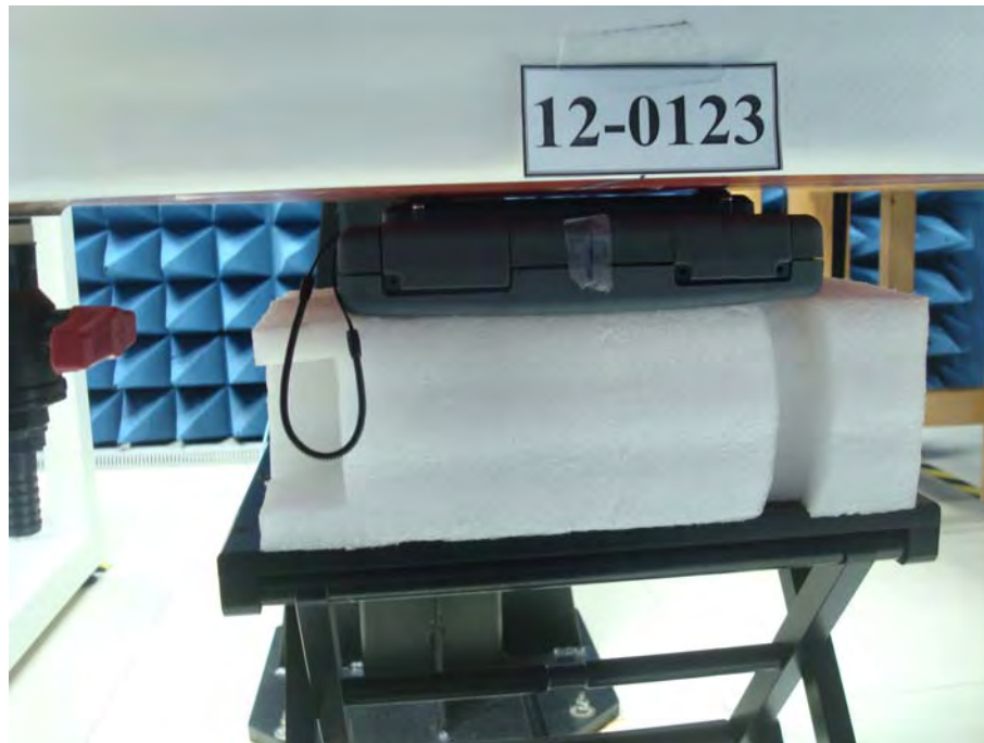
Body Setup (EUT with Thin Battery, Back surface to phantom 0mm)
