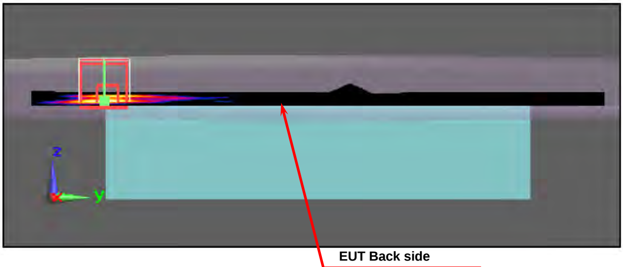
Body SAR Test Setup (Flat Section)
