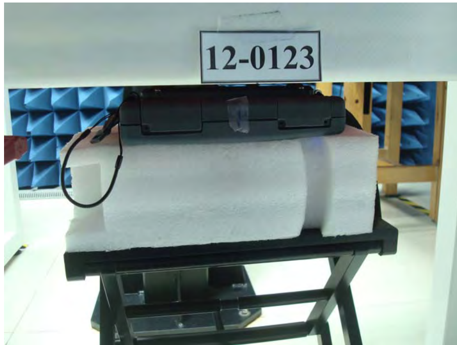
Body Setup (EUT with Thick Battery and Hand Strap, Back surface to phantom 0mm)
