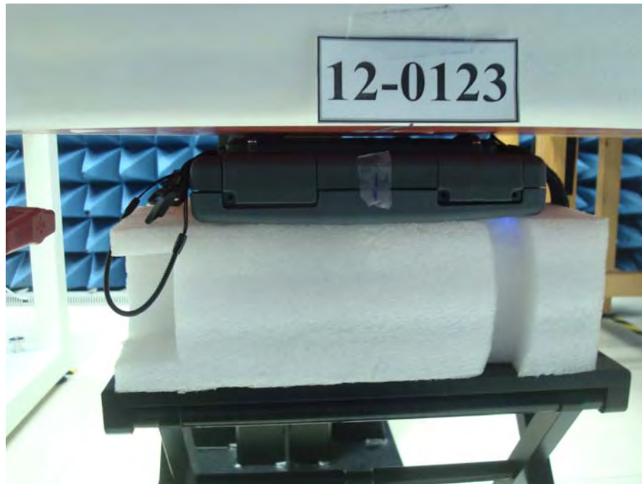
Body Setup (EUT with Hip Pad Battery and Hand Strap, Back surface to phantom 0mm)
