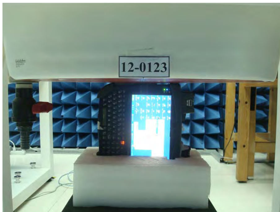
Body Setup (EUT with Internal Battery, Barcode and Magnetic Stripe, Edge Left to phantom 0mm)
