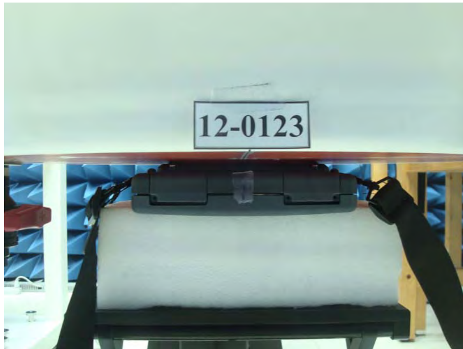
Body Setup (EUT with Hip Pad Battery and Shoulder Strap, Back surface to phantom 0mm)
