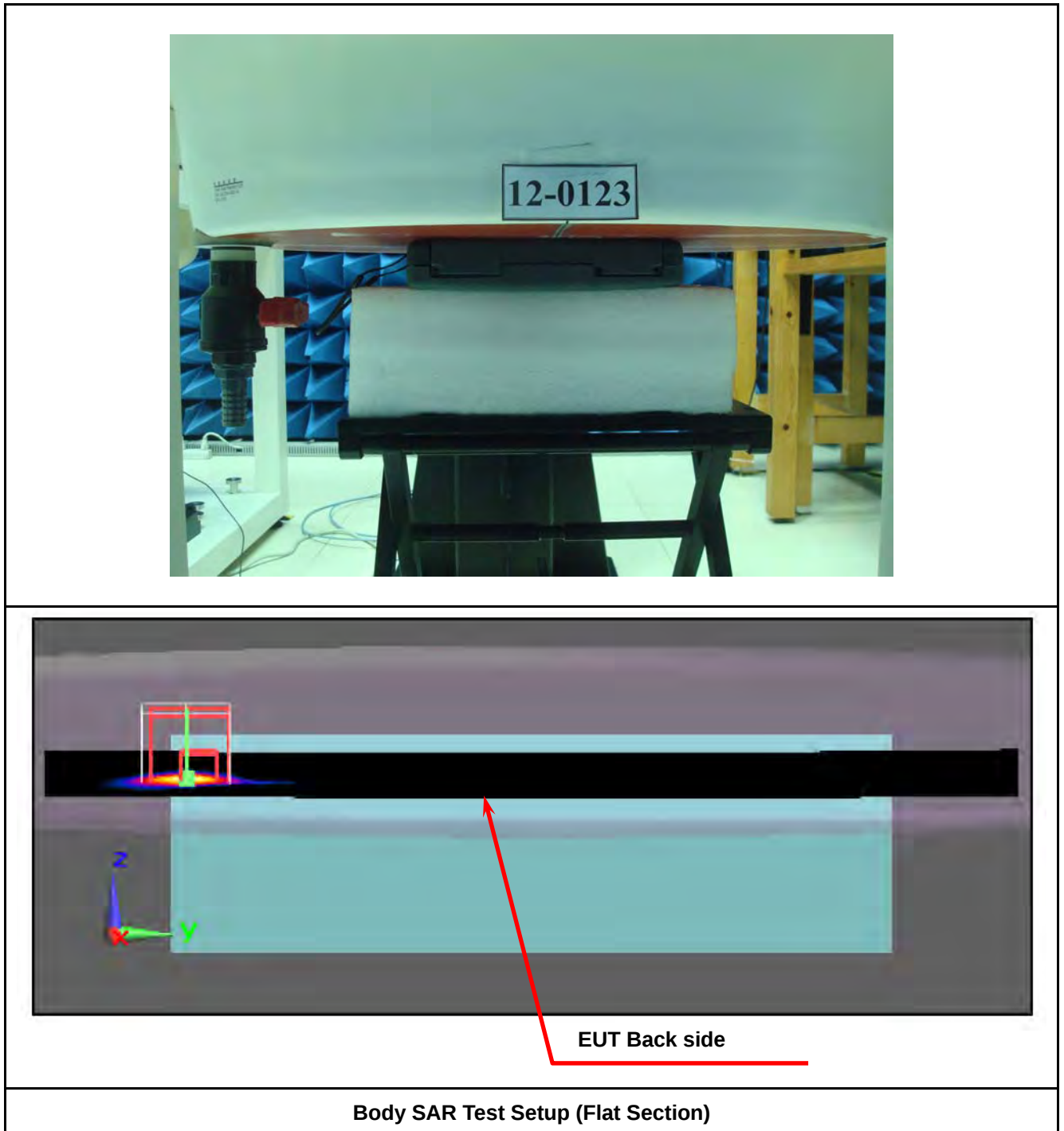
Body Setup (EUT with Internal Battery, Back surface to phantom 0mm)
