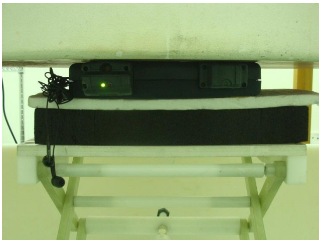
Rear Face of DUT with Earphone (DUT without Holster)
