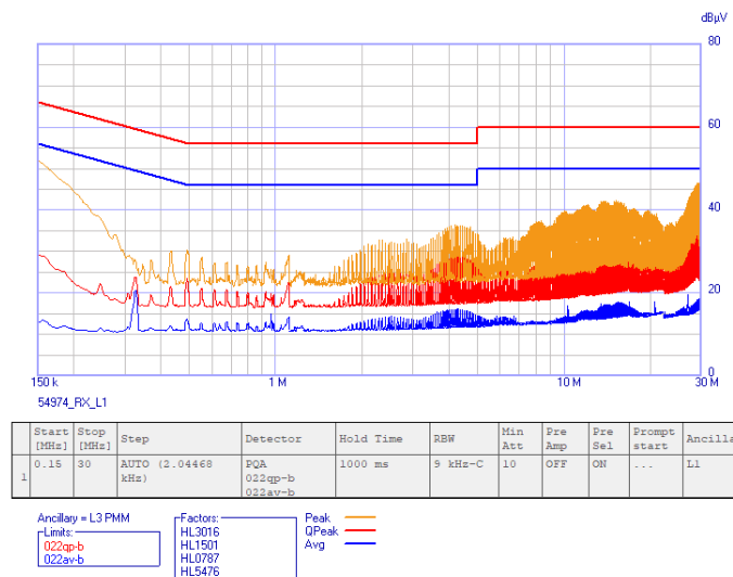
Plot 8.1.2 Conducted emission measurements, AC mains input of AC/DC adapter
