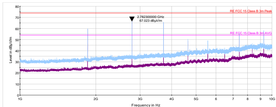
Plot 7.6.12 Radiated emission measurements from 1000 to 10000 MHz at the high carrier frequency
