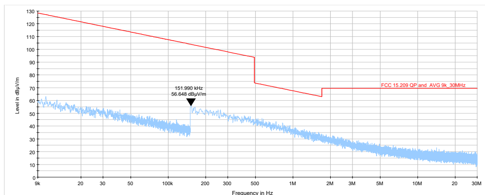
Plot 7.6.6 Radiated emission measurements from 9 to 30000 kHz at the high carrier frequency
