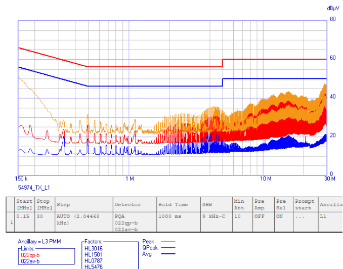
Plot 7.8.2 Conducted emission measurements, AC mains input of AC/DC adapter
