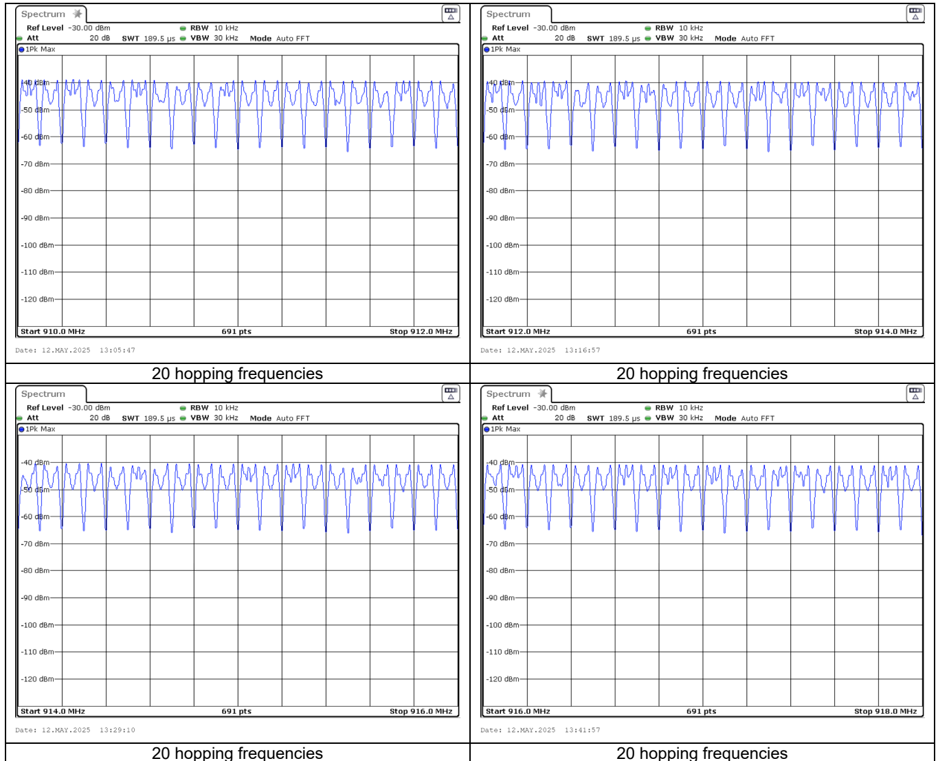
Plot 7.3.2 Number of hopping frequencies (continuation)
