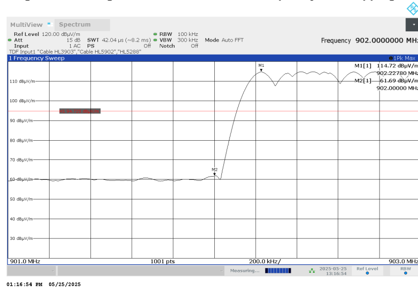
Plot 7.7.3 The highest band edge emission at low carrier frequency with hopping function enabled
