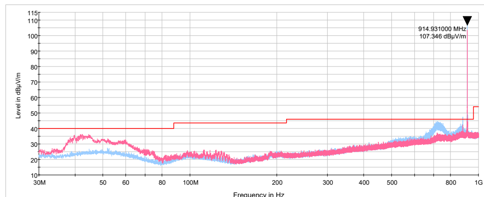
Plot 7.6.9 Radiated emission measurements from 30 to 1000 MHz at the high carrier frequency
