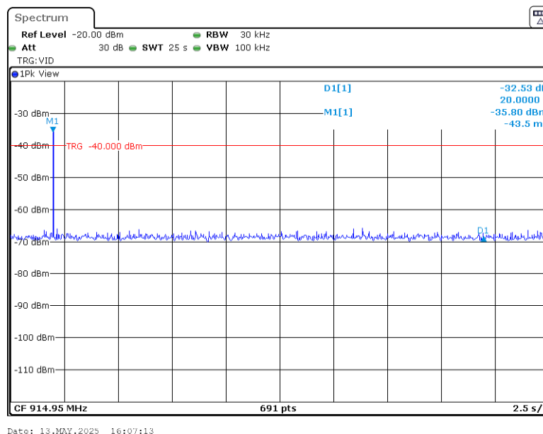
Plot 7.6.14 Transmission pulse period
