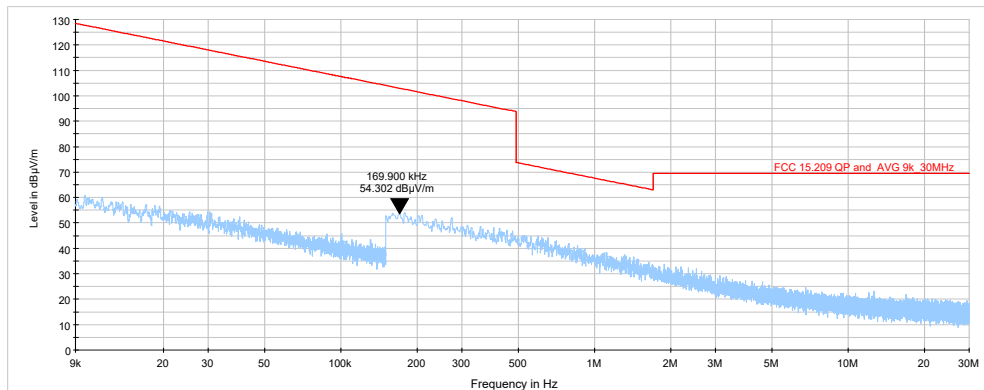
Plot 7.6.5 Radiated emission measurements from 9 to 30000 kHz at the mid carrier frequency
