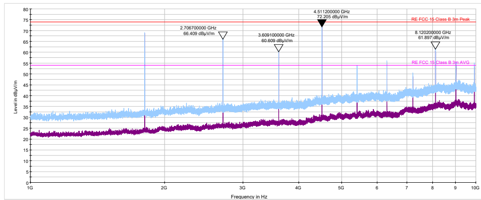
Plot 7.6.11 Radiated emission measurements from 1000 to 10000 MHz at the mid carrier frequency
