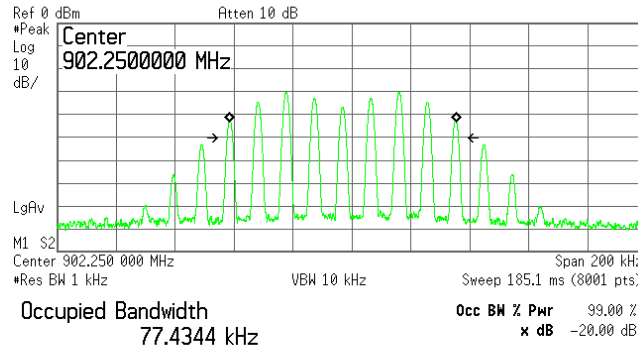
Plot 7.1.1 The 20 dB bandwidth test result at low frequency
