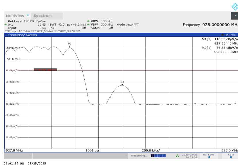
Plot 7.7.4 The highest band edge emission at high carrier frequency with hopping function enabled
