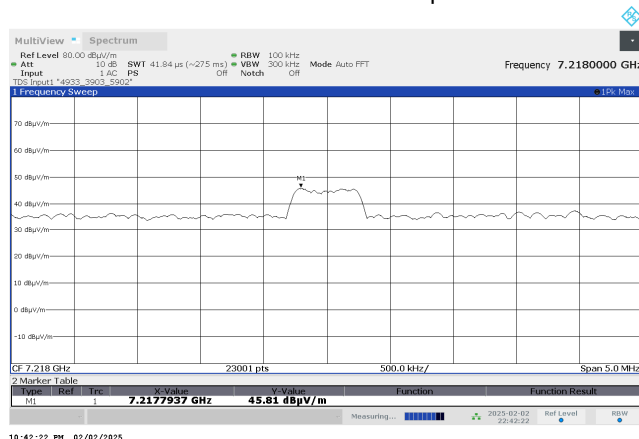
Plot 7.6.22 Radiated emission measurements at the 10 th harmonic of high carrier frequency
