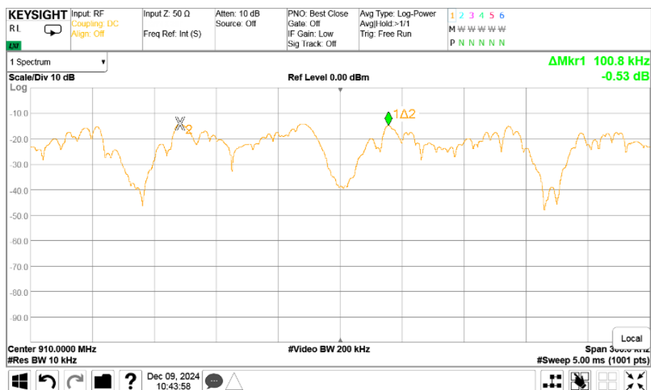
Plot 7.2.1 Carrier frequency separation
