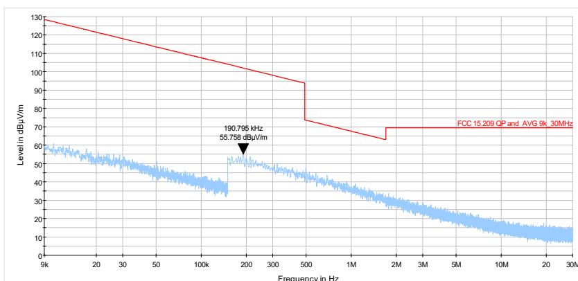
Plot 7.6.3 Radiated emission measurements from 9 kHz to 30 MHz at the high carrier frequency
