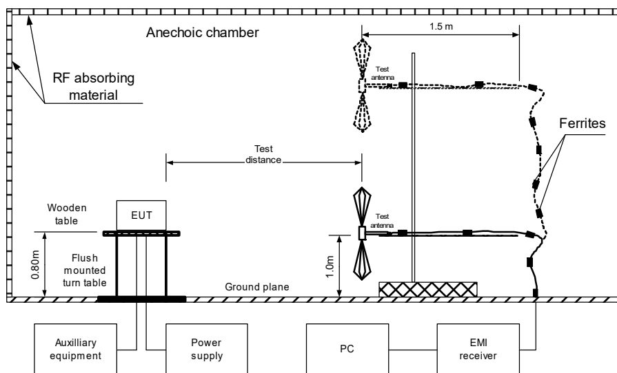
Figure 8.1.1 Setup for radiated emission measurements below 1 GHz, table-top EUT
