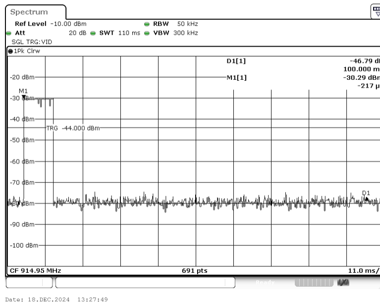
Plot 7.6.24 Transmission pulse period
