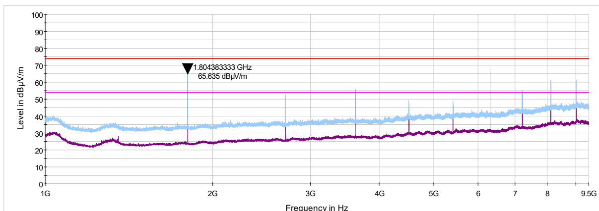
Plot 7.6.8 Radiated emission measurements from 1000 to 9500 MHz at the low carrier frequency (RBW 100 kHz)
