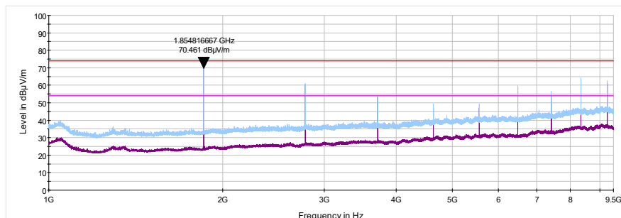
Plot 7.6.12 Radiated emission measurements from 1000 to 9500 MHz at the high carrier frequency (RBW 100 kHz)
