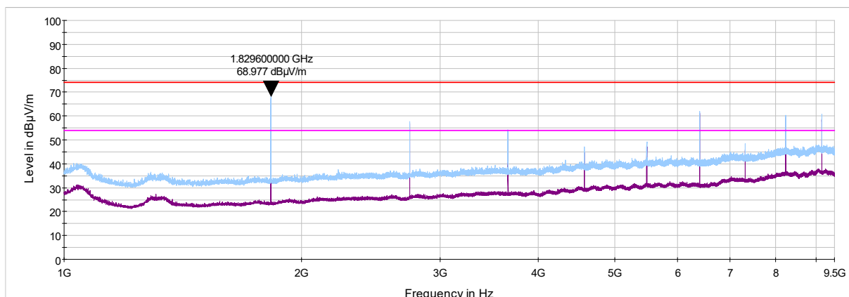
Plot 7.6.10 Radiated emission measurements from 1000 to 9500 MHz at the mid carrier frequency (RBW 100 kHz)
