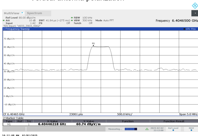
Plot 7.6.20 Radiated emission measurements at the 7 th harmonic of high carrier frequency
