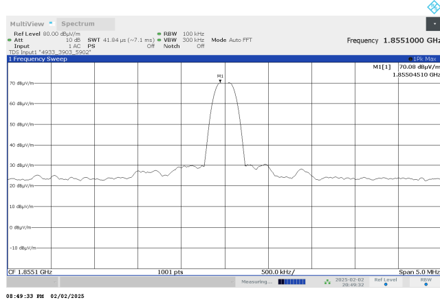
Plot 7.6.16 Radiated emission measurements at the 6 th harmonic of mid carrier frequency
