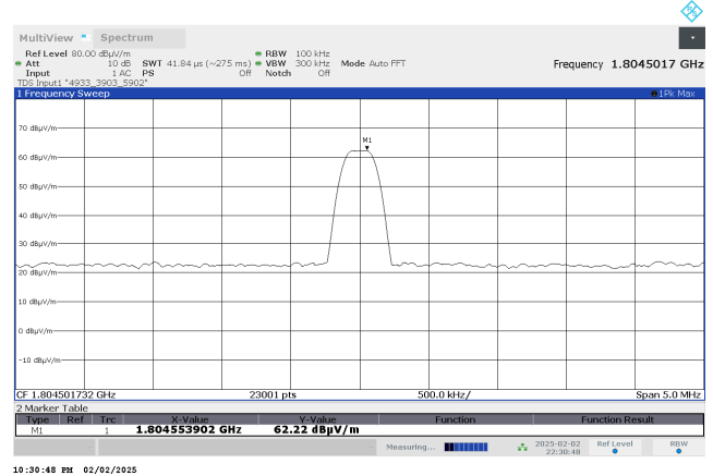
Plot 7.6.14 Radiated emission measurements at the 2 nd harmonic of mid carrier frequency
