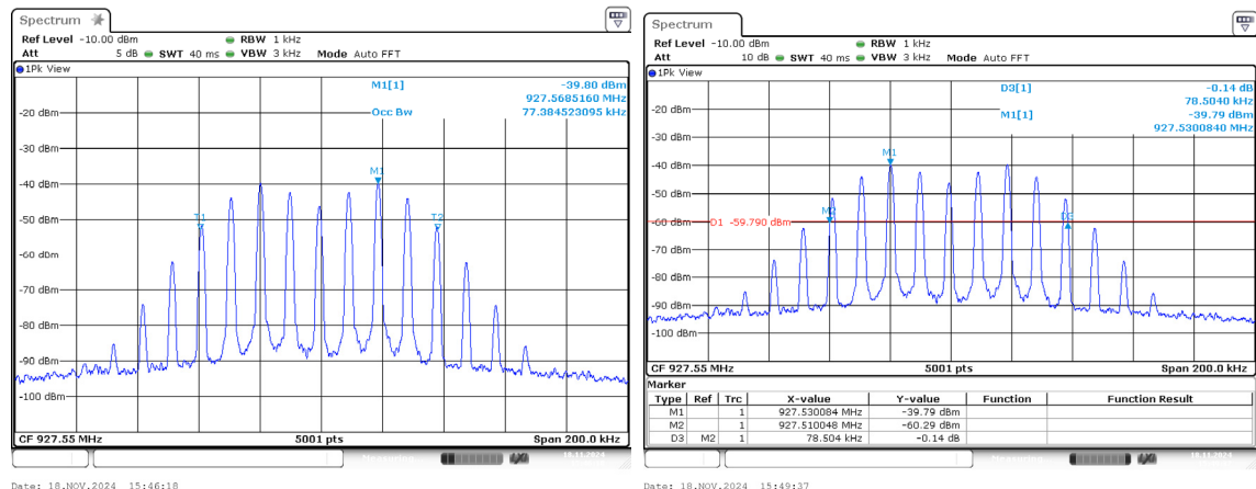
Plot 7.1.3 The 20 dB bandwidth test result at high frequency
