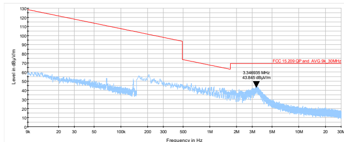
Plot 7.6.3 Radiated emission measurements from 9 to 30000 kHz at the high carrier frequency
