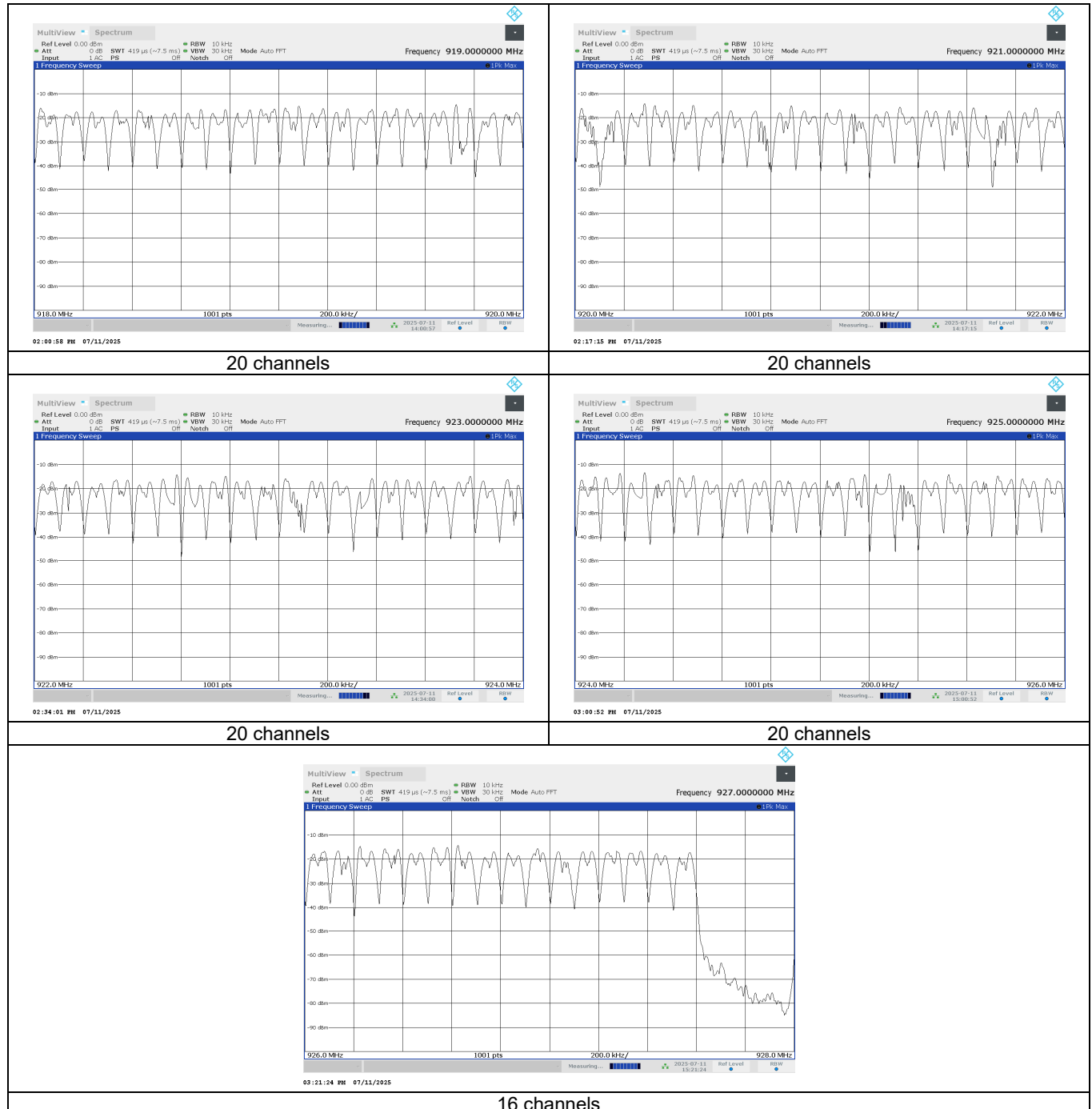
Plot 7.3.3 Number of hopping frequencies
