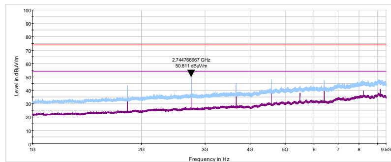
Plot 7.6.9 Radiated emission measurements from 1000 to 9500 MHz at the high carrier frequency
