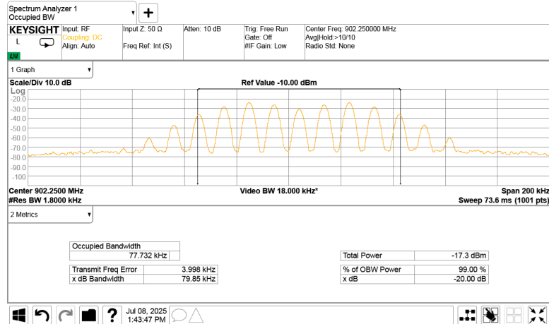
Plot 7.1.2 The 20 dB bandwidth test result at mid frequency
