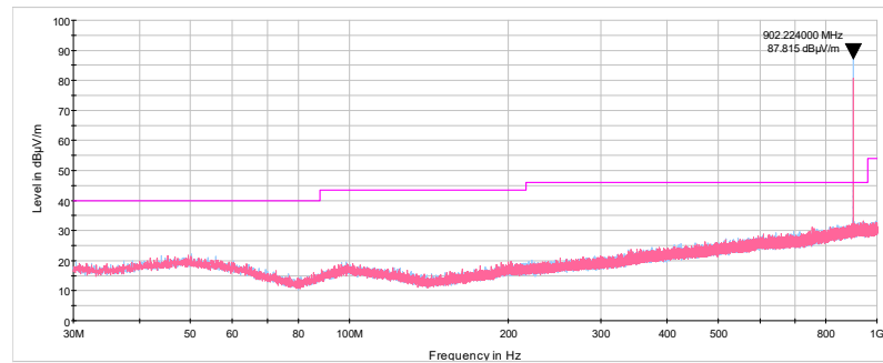
Plot 7.6.5 Radiated emission measurements from 30 to 1000 MHz at the mid carrier frequency
