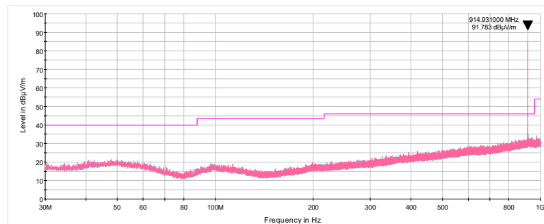
Plot 7.6.6 Radiated emission measurements from 30 to 1000 MHz at the high carrier frequency
