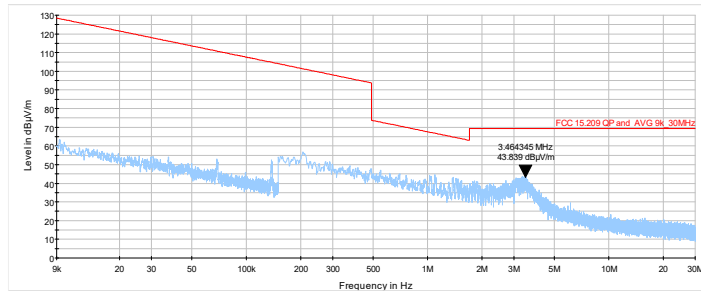
Plot 7.6.2 Radiated emission measurements from 9 to 30000 kHz at the mid carrier frequency
