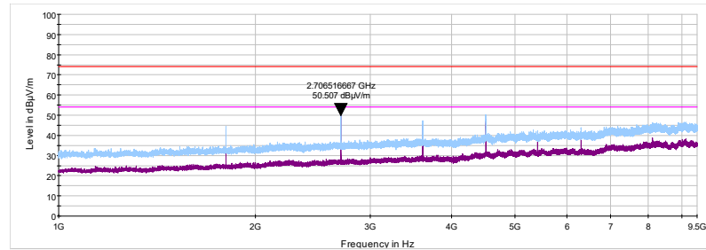
Plot 7.6.8 Radiated emission measurements from 1000 to 9500 MHz at the mid carrier frequency
