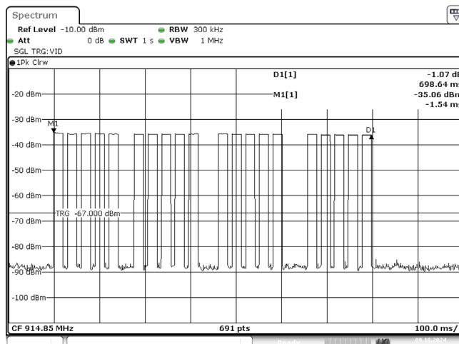
Plot 7.6.14 Transmission train duration
