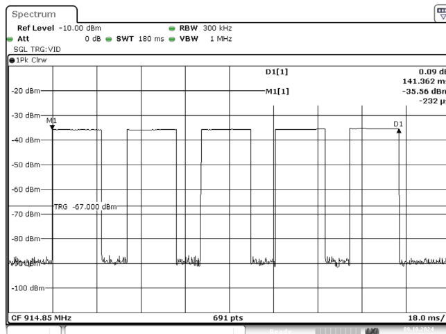
Plot 7.6.13 Transmission burst period
