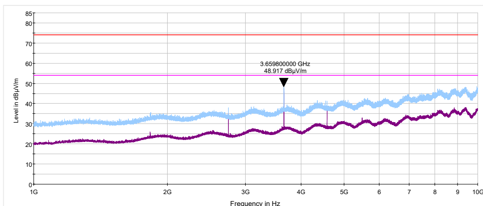
Plot 7.6.9 Radiated emission measurements from 1000 to 10000 MHz at the high carrier frequency
