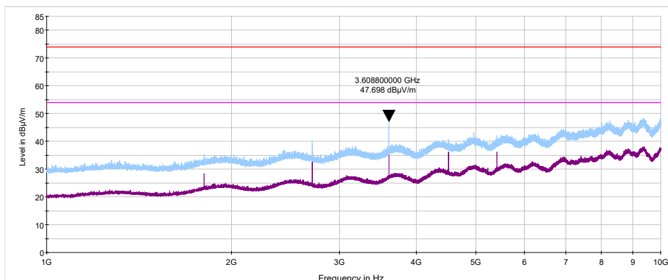
Plot 7.6.8 Radiated emission measurements from 1000 to 10000 MHz at the mid carrier frequency
