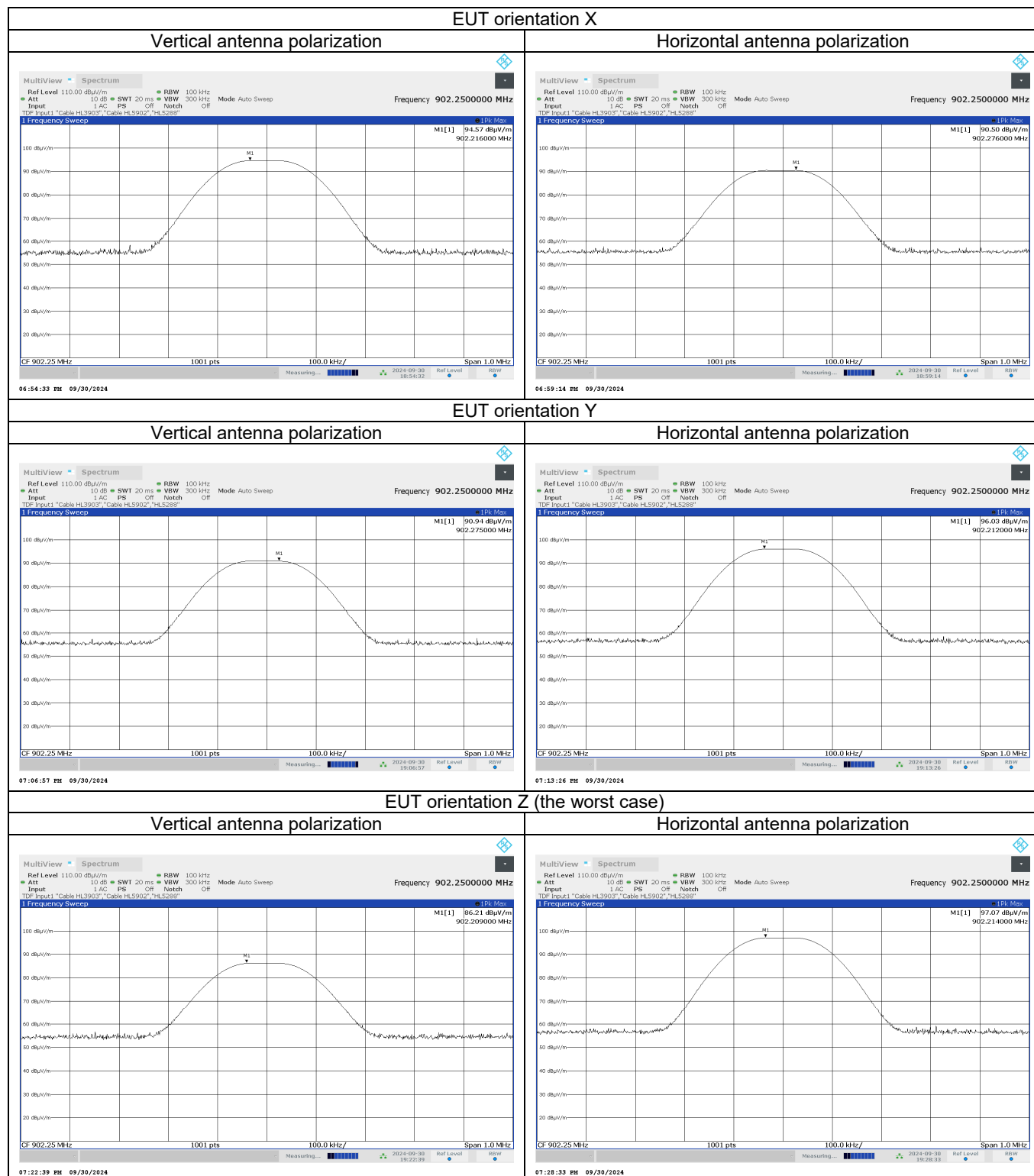
Plot 7.5.1 Field strength of carrier at low frequency
