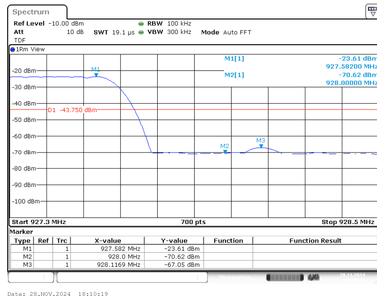
Plot 7.7.4 The highest band edge emission at low carrier frequency with hopping function enabled
