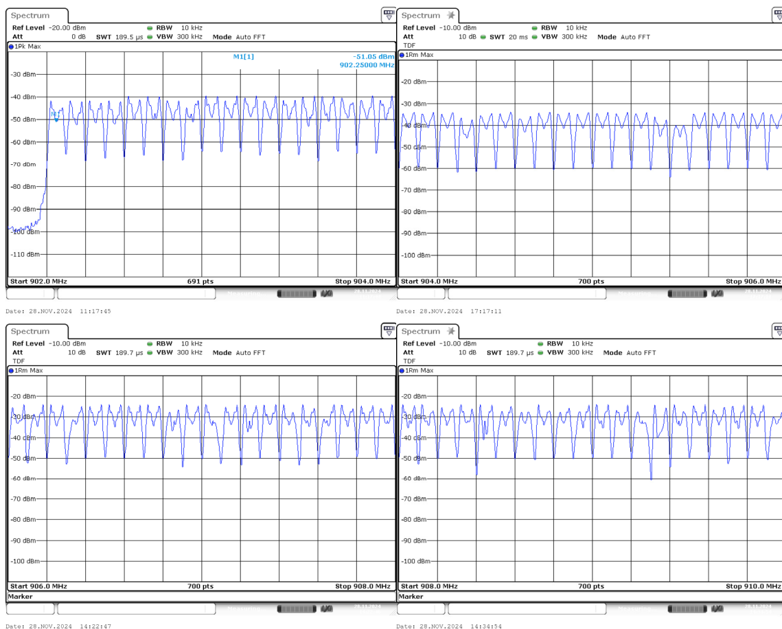
Plot 7.3.1 Number of hopping frequencies
