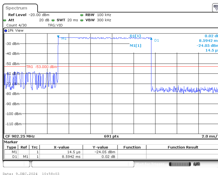
Plot 7.4.1 Single transmission duration
