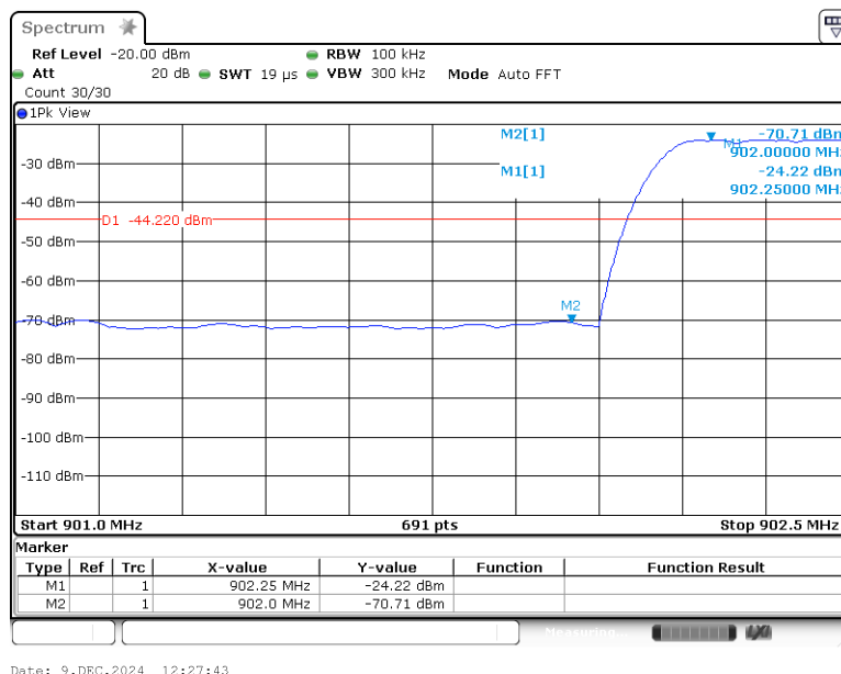
Plot 7.7.3 The highest band edge emission at low carrier frequency with hopping function enabled
