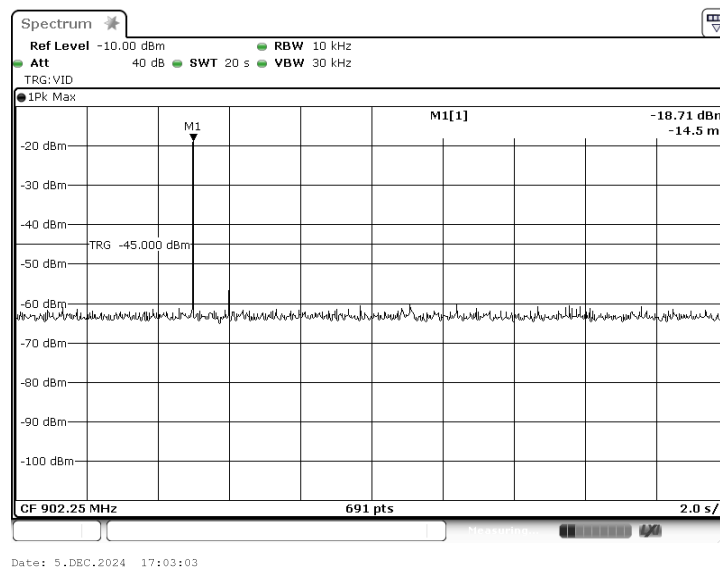
Plot 7.6.11 Number pulse during 100 msec
