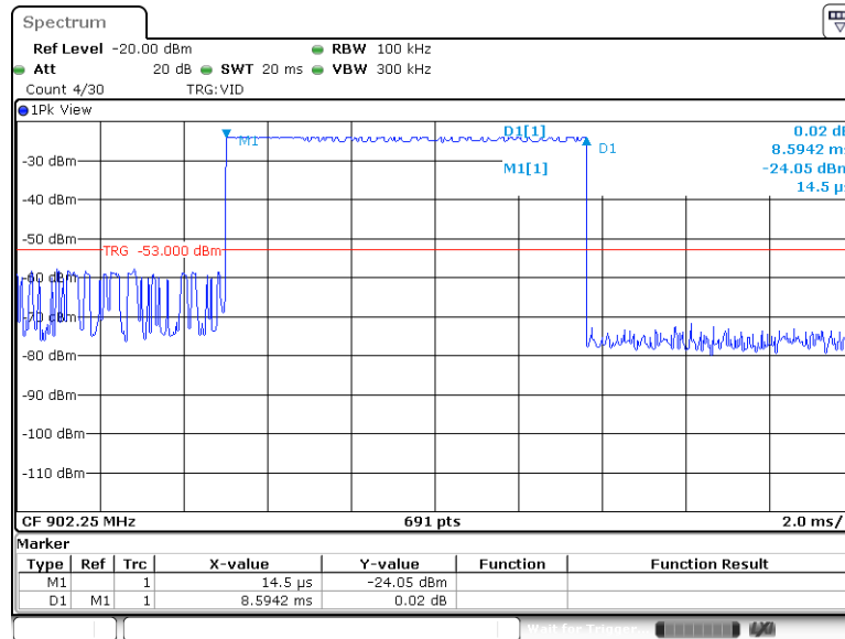
Plot 7.6.10 Transmission pulse duration
