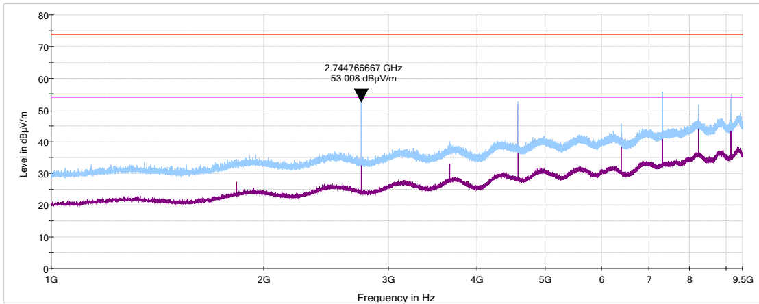
Plot 7.6.12 Radiated emission measurements from 1000 to 9.500 MHz at the high carrier frequency
