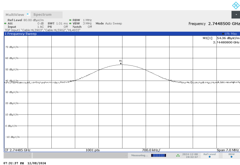
Plot 7.6.16 Radiated emission measurements at the third harmonic of high carrier frequency
