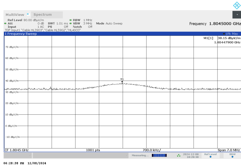
Plot 7.6.14 Radiated emission measurements at the third harmonic of low carrier frequency
