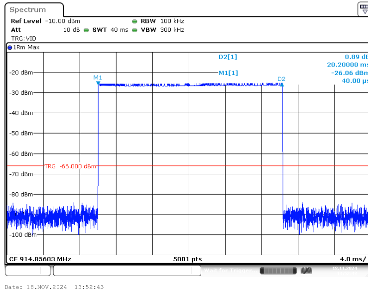
Plot 7.6.32 Transmission pulse period
