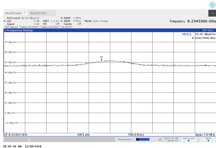
Plot 7.6.27 Radiated emission measurements at the ninth harmonic of high carrier frequency
