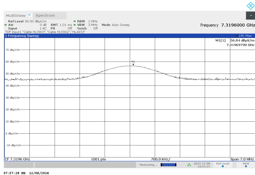
Plot 7.6.25 Radiated emission measurements at the eighth harmonic of high carrier frequency
