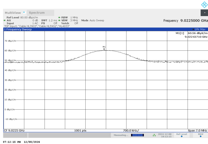
Plot 7.6.29 Radiated emission measurements at the tenth harmonic of mid carrier frequency
