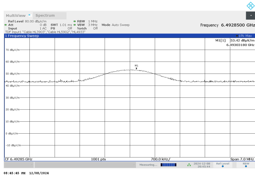
Plot 7.6.23 Radiated emission measurements at the eighth harmonic of low carrier frequency
