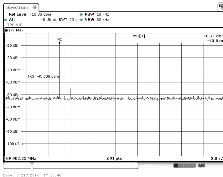
Plot 7.6.32 Transmission pulse period
