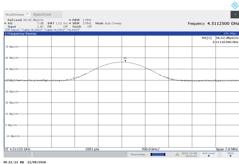
Plot 7.6.18 Radiated emission measurements at the fifth harmonic of mid carrier frequency
