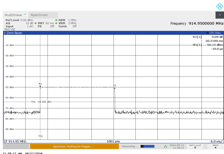
Plot 7.4.1 Single transmission duration
