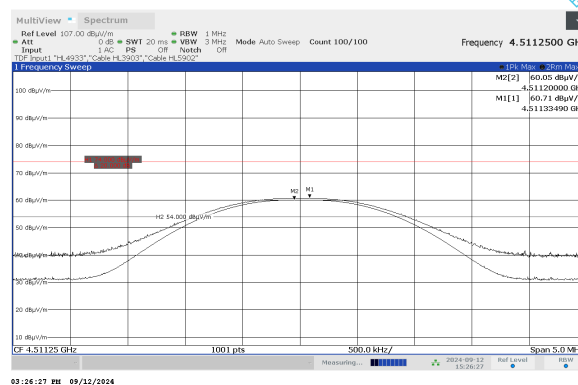
Plot 7.6.11 Radiated emission measurements at the fifth harmonic of mid carrier frequency
