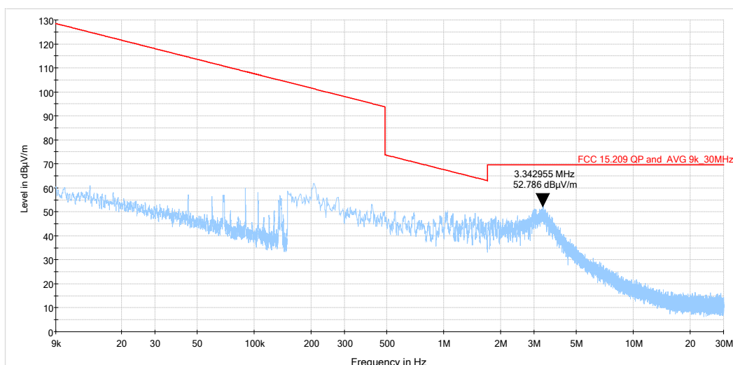
Plot 7.6.2 Radiated emission measurements from 0.009 to 30 MHz at the mid carrier frequency
