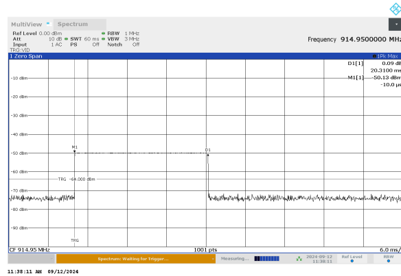
Plot 7.6.2 Transmission pulse period
