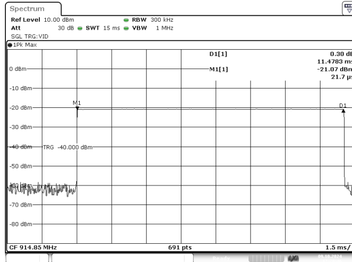
Plot 7.6.15 Transmission pulse duration
