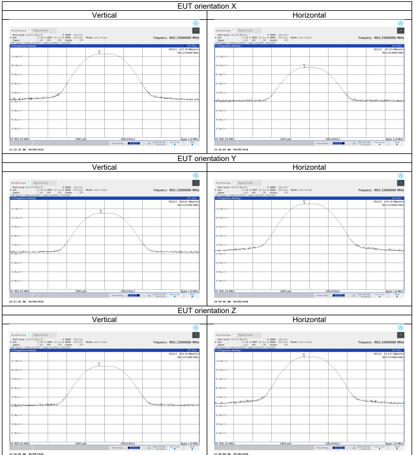
Plot 7.5.1 Field strength of carrier at low frequency
