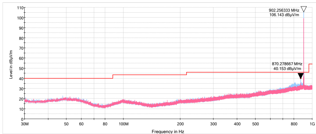
Plot 7.6.5 Radiated emission measurements from 30 to 1000 MHz at the mid carrier frequency
