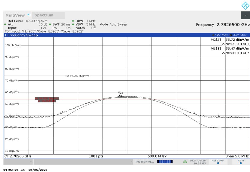
Plot 7.6.11 Radiated emission measurements at the fifth harmonic of low carrier frequency
