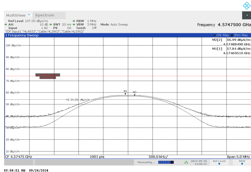
Plot 7.6.13 Radiated emission measurements at the fifth harmonic of high carrier frequency
