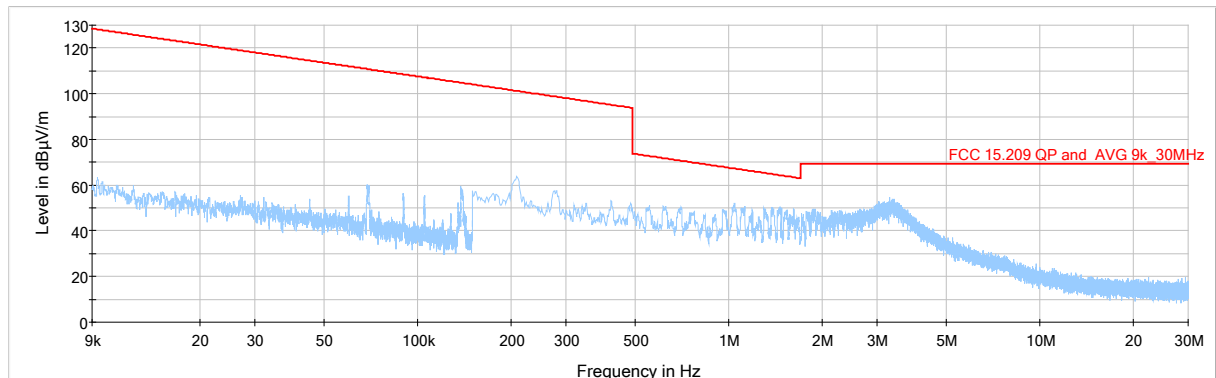
Plot 7.6.2 Radiated emission measurements from 0.009 to 30 MHz at the mid carrier frequency
