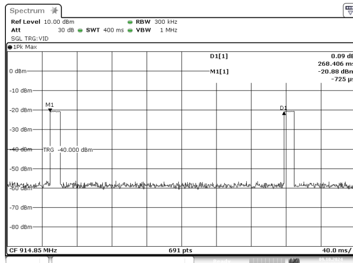
Plot 7.6.16 Transmission pulse period
