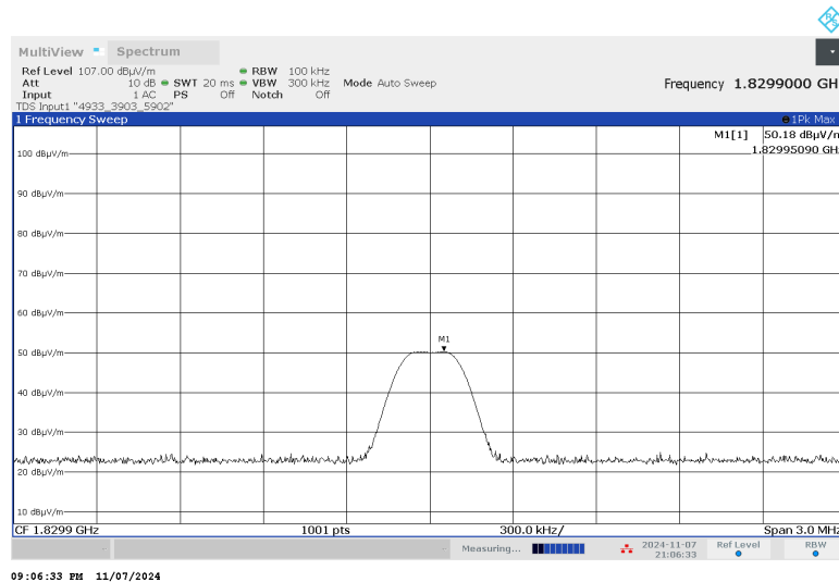
Plot 7.6.11 Radiated emission measurements at the eighth harmonic of low carrier frequency
