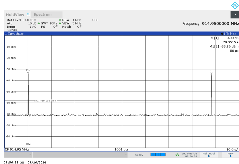
Plot 7.6.14 Transmission pulse period
