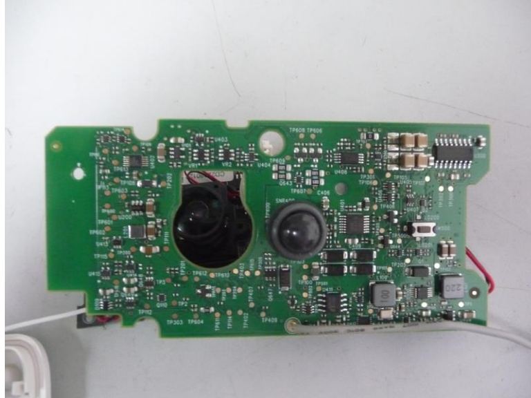
Photograph No.2 Print side of the main PCB
