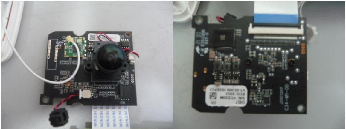
Photograph No.3 Camera Module
